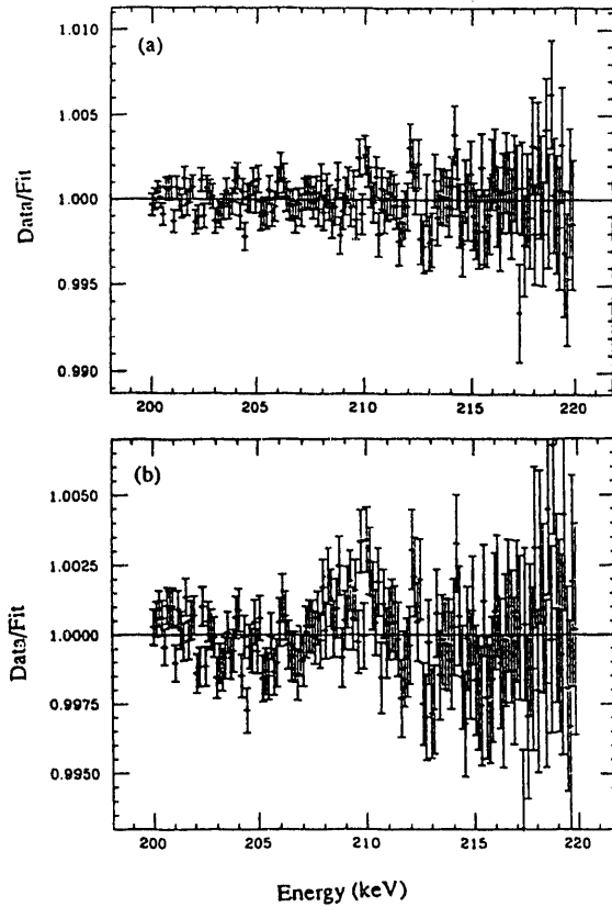
Fig. 5. Ratio of the type (3) ^{55}\text{Fe} data to fits using Eqn. 1. (a) Fit performed assuming m_\nu = 0 . The horizontal line is the expectation for massless neutrinos. (b) Fit performed assuming m_\nu = 17 keV and \tan^2\theta = 0.007 . The horizontal line is the expectation for m_\nu = 17 keV and \tan^2\theta = 0.007 .
