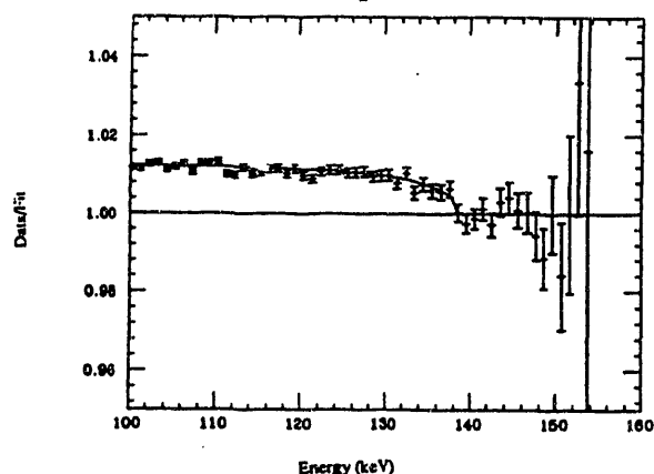
Fig. 2. The ratio of the ^{14}\text{C} data to the extrapolation of a theoretical fit performed over the region 141-156 keV assuming m_\nu = 0 . The horizontal line is the shape expected for zero-mass neutrinos. The curve illustrates the shape expected if a 17-keV neutrino were emitted in 1.3% of the ^{14}\text{C} beta decays.
