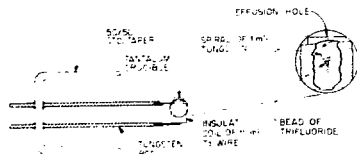
Fig. 6. Schematic diagram of low heat capacity reduction system.
