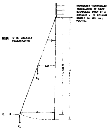
PRINCIPLE OF THE MAGNETIC SUSCEPTIBILITY APPARATUS
