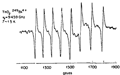
Fig. 15. EPR spectrum of \text{ThO}_2: {}^{249}\text{Bk}^{4+} at \sim 1.5\text{K} . The nuclear spin is equal to 7/2 and the spectrum is isotropic for all crystal orientations at this frequency.
