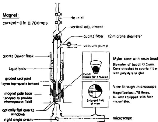
Fig. 2. Magnetic susceptibility apparatus.
