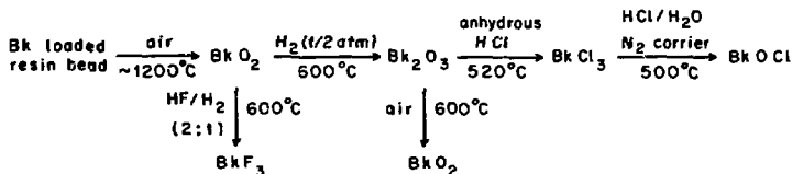
Fig. 15. Preparation of five Bk compounds.
