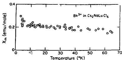
Fig. 10. Magnetic susceptibility of \text{Bk}^{3+} in \text{Cs}_2\text{NaLuCl}_6 below 70^{\circ}\text{K} . The correction for \text{Cf}^{3+} impurity is negligible. Below 40^{\circ}\text{K} the temperature-independent paramagnetic susceptibility is 192\,000 \times 10^{-6} emu/mole.
