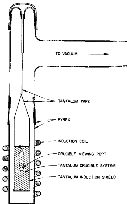
Berkelium Metal Reduction System.
