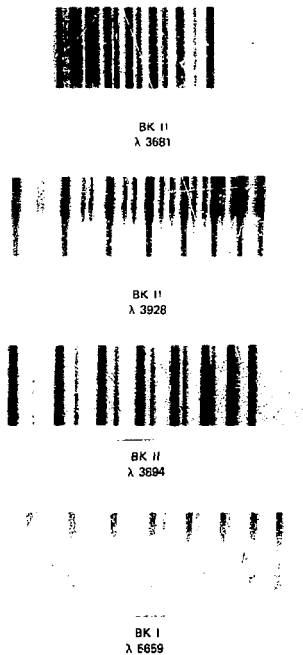
Fig. 1. Four examples of berkelium lines exhibiting hyperfine structure.
