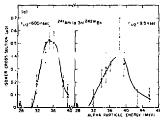
Fig. 4. Excitation curves for the formation of two excited isomers of ^{242}\text{Bk} that decay by spontaneous fission.
