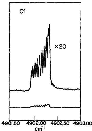
Fig. 3. Fourier transform tracing of a Cf line at 4902.215 \text{ cm}^{-1} .
