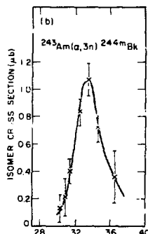
Fig. 5. Excitation curve for the formation of an excited isomer of ^{244}\text{Bk} that decays by spontaneous fission.
