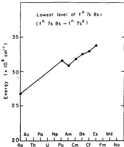
Fig. 9. The difference between the lowest level of f^n 7s 8s and f^n 7s^2 is plotted for the actinides.
