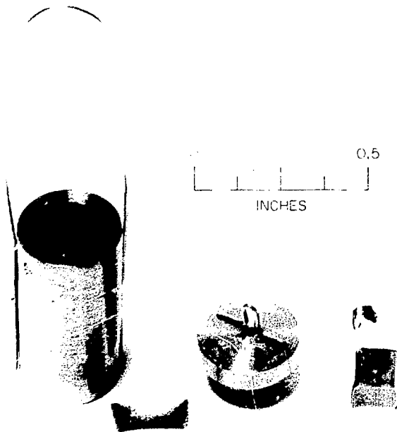
Berkelium Metal Reduction Crucible and Metal Spiral.
