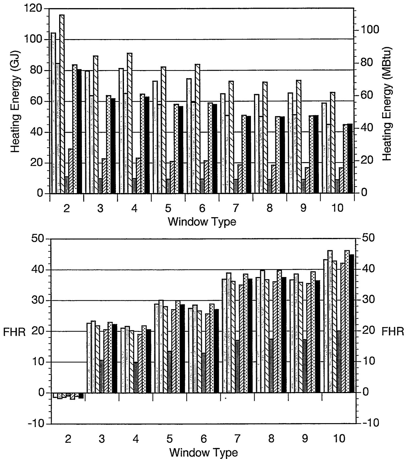
Figure 1: Heating energy and FHR values for seven geographic locations using window number 1 as a base. Base heating energy values are: Boston (102.7 GJ, 97.4 MBtu), Denver (83.1 GJ, 78.8 MBtu), Madison (114.2 GJ, 108.3 MBtu), Miami (10.9 GJ, 10.3 MBtu), Phoenix (28.6 GJ, 27.1 MBtu), Seattle (82.7 GJ, 78.4 MBtu), and St. Louis (79.3 GJ, 75.2 MBtu).
