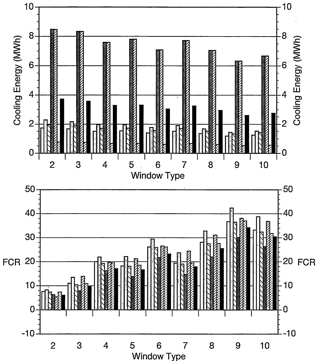
Figure 2: Cooling energy and FCR values for seven geographic locations using window number 1 as a base. Base cooling energy values are: Boston (1881 kWh), Denver (2502 kWh), Madison (2108 kWh), Miami (9048 kWh), Phoenix (9932 kWh), Seattle (827 kWh), and St. Louis (3962 kWh).
