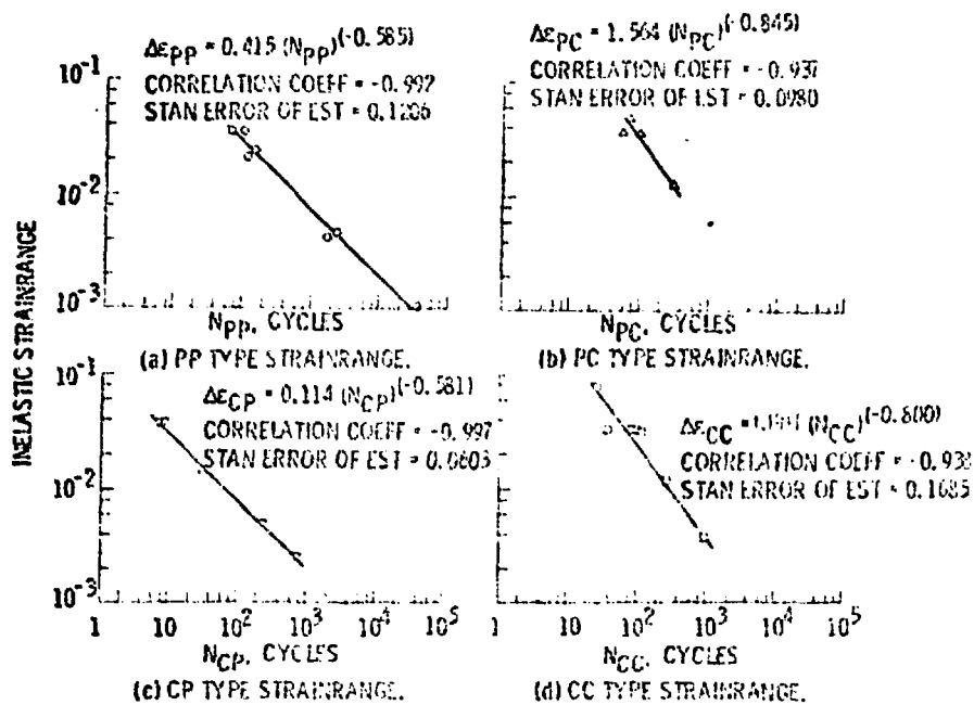
Figure 5. - Partitioned strainrange - life relations for AISI Type 316 stainless steel, 1300° F (705° C), Ref. (6).
