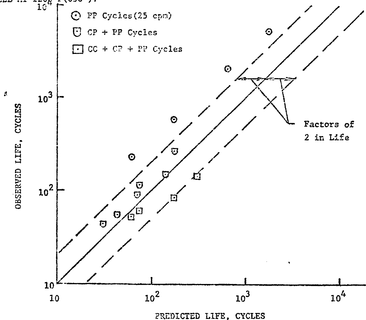
FIG. 8 - APPLICABILITY OF STRAINRANGE PARTITIONING MULTIAXIALITY RULES TO PREDICTION OF ZAMRIK AND BILIR'S(7) TORSIONAL CREEP-FATIGUE LIVES FOR AISI TYPE 304 STAINLESS STEEL AT 1200^{\circ}\text{F} ( 650^{\circ}\text{C} ).
