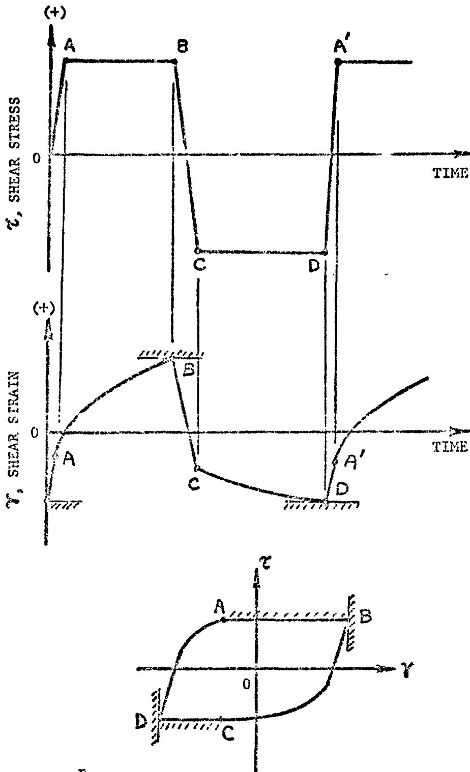
FIG. 6 - SCHEMATIC SHEAR STRESS AND SHEAR STRAIN CONDITIONS USED BY ZAMRIK AND BILIR, REF. (7).
