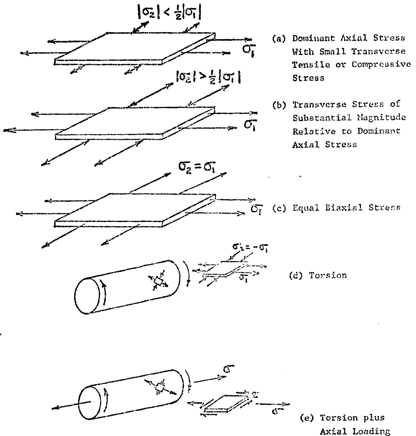
FIG. 3 - SEVERAL CASES OF BIAXIAL LOADING DISCUSSED IN CONNECTION WITH ANALYSIS BY STRAINRANGE PARTITIONING.
