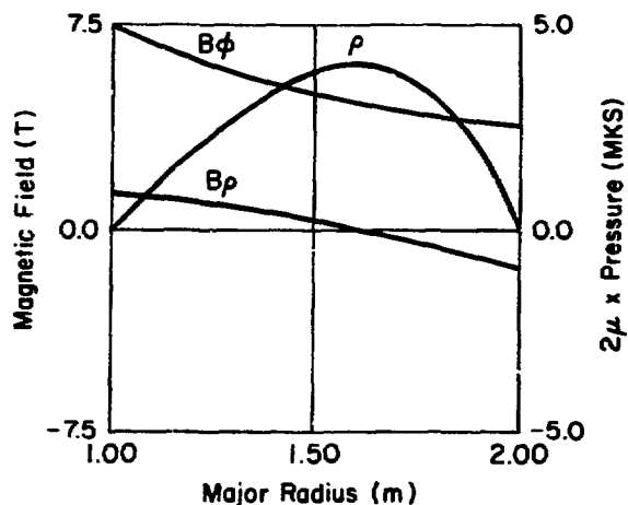
Fig. VII-3. Tokamak profile with toroidal and poloidal magnetic fields.
