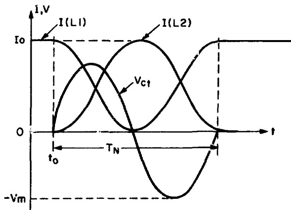
Fig. IX-10. Notch circuit current and voltage waveforms.
