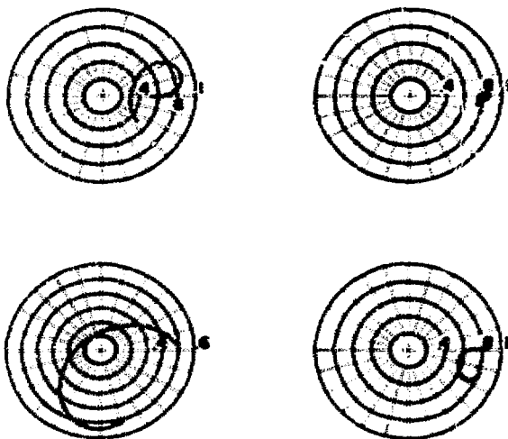
Fig. VII-13. Typical ion orbits.
