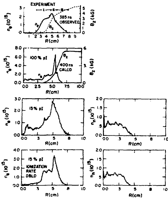
Fig. VII-12 Comparison of experiment and theory for Scylla 1B.
