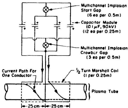
consisting of two 25-cm-long, back-to-back, counter-wound Marshall coils. Each Marshall coil is driven by six parallel pairs of two series, 0.1- \mu F, 90-kV capacitor modules. One-half of the series capacitors are charged positive, and the other half are charged negative. Figure IX-6 shows an end view of the implosion-heating system. The start and crowbar gaps are linear, multichannel spark gaps. The length of the Marshall coils (25 cm) was chosen as 1/16 of the wavelength for fabrication considerations. The capacitor modules are dc charged to positive and negative 75 kV. The Marshall coil produces the implosion voltage necessary to obtain a 1-keV implosion temperature by the transformer properties of the fractional-turn coil.
