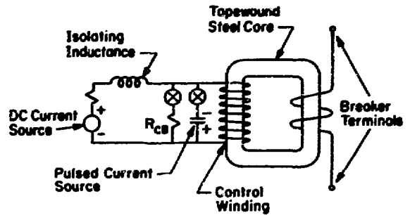
Fig. IX-11. Saturable inductor breaker for notch circuit.
