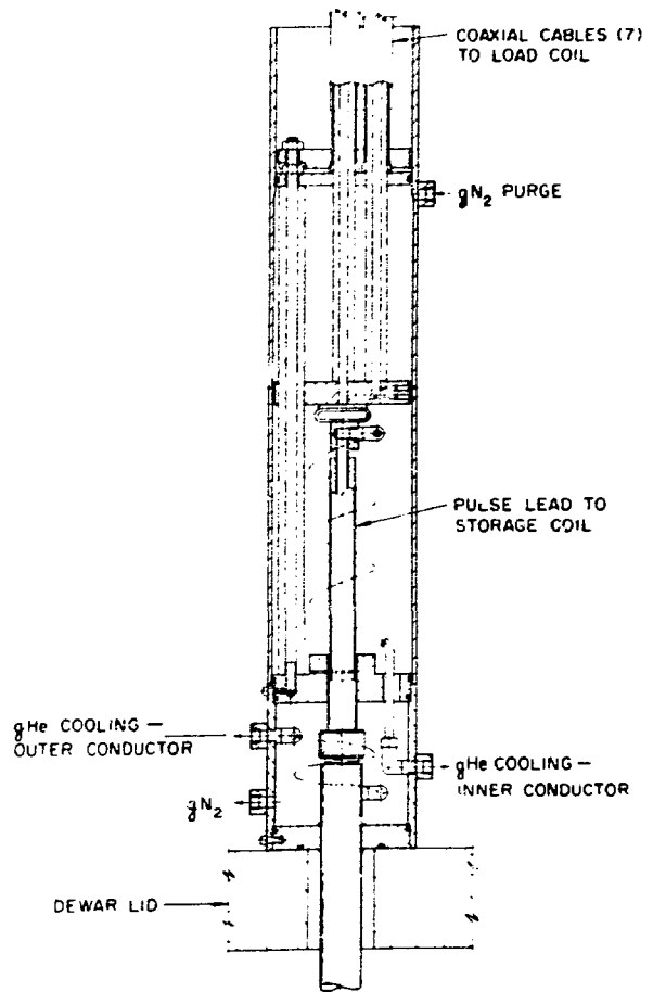
Fig. XII-3. Pulsed Lead - Cable Connector.
