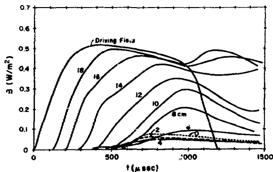
IHX Magnetic Field in Plasma as Measured by Probe
