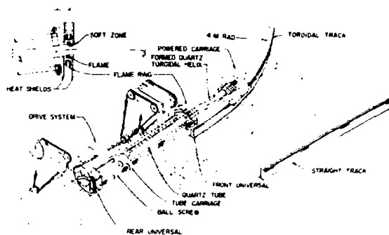
QUARTZ TUBE FORMING MACHINE
