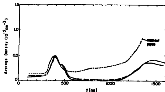
IHX Interferometer Density Showing Effect of Plasma at Ends
