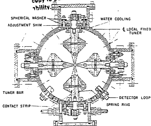
Fig. 1. Typical cavity cross section.
