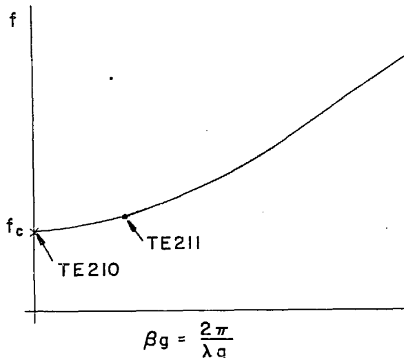
Fig. 4. Dispersion curve for uniform structure.
