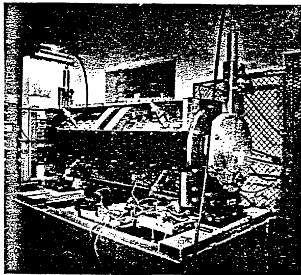
Fig. 2. RFQ complete on transporter.
