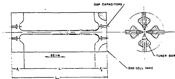
Fig. 3. Diagrammatic representation of RFQ.
