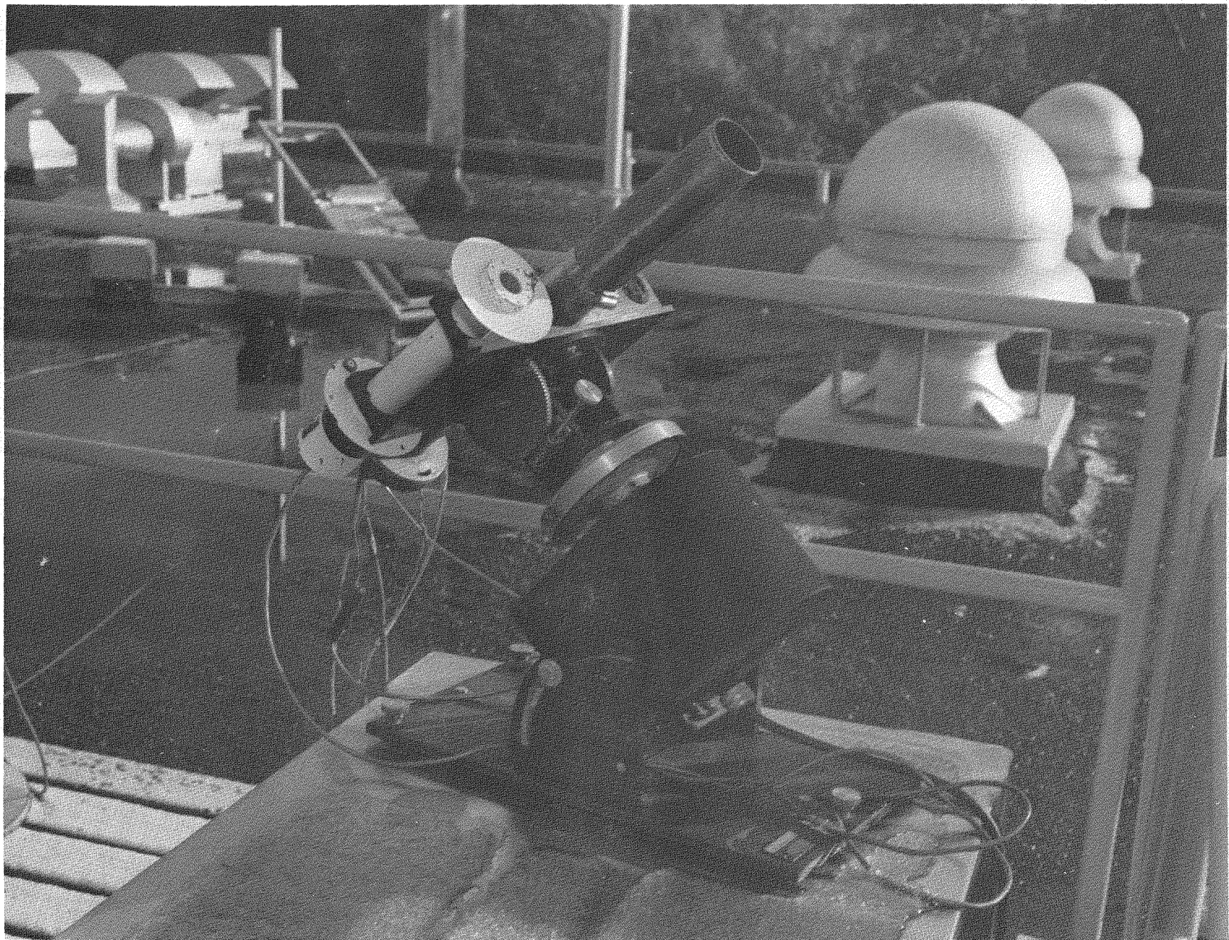
Figure 3. - Solar cell calibration apparatus
