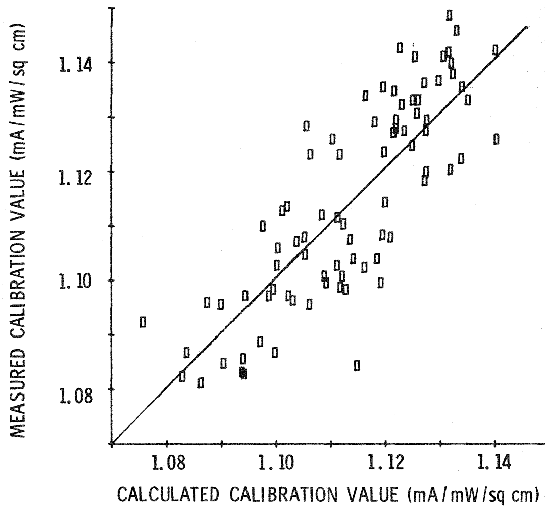
Figure 5. - Measured versus calculated calibration value
