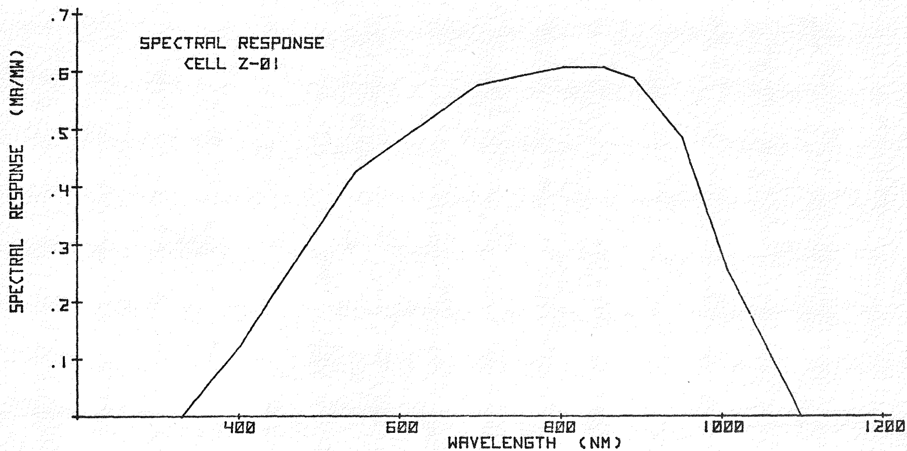
Figure 2. - Spectral response curve of cell Z 01
