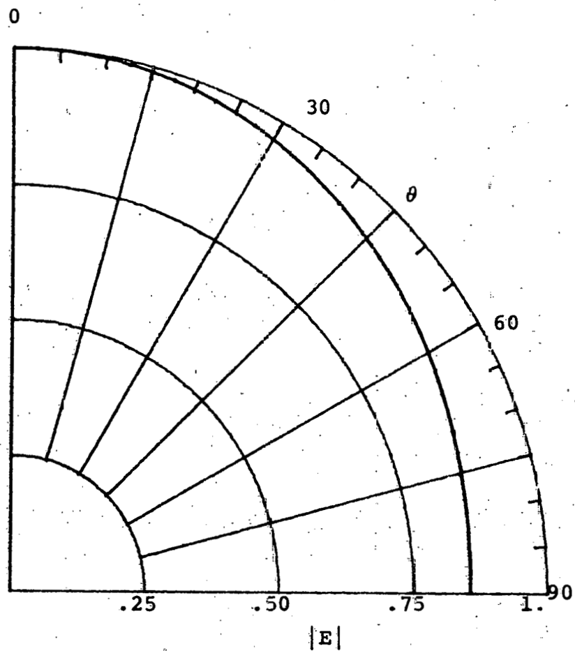
Figure 6. Circular Microstrip Antenna (r_0/\lambda = 0.1, \nu = 1)
