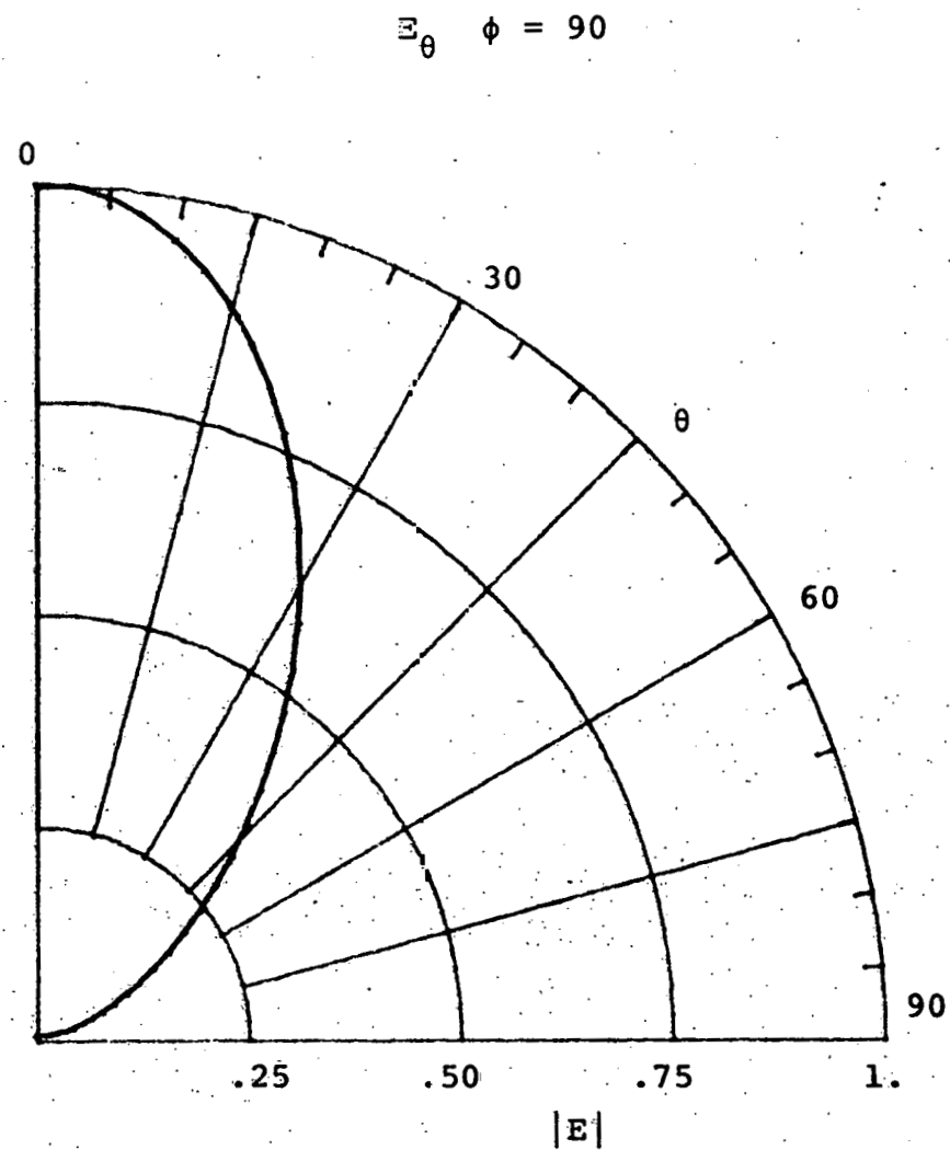
Figure 10. Circular Microstrip Antenna (r_o/\lambda = 0.5, \nu = 1)
