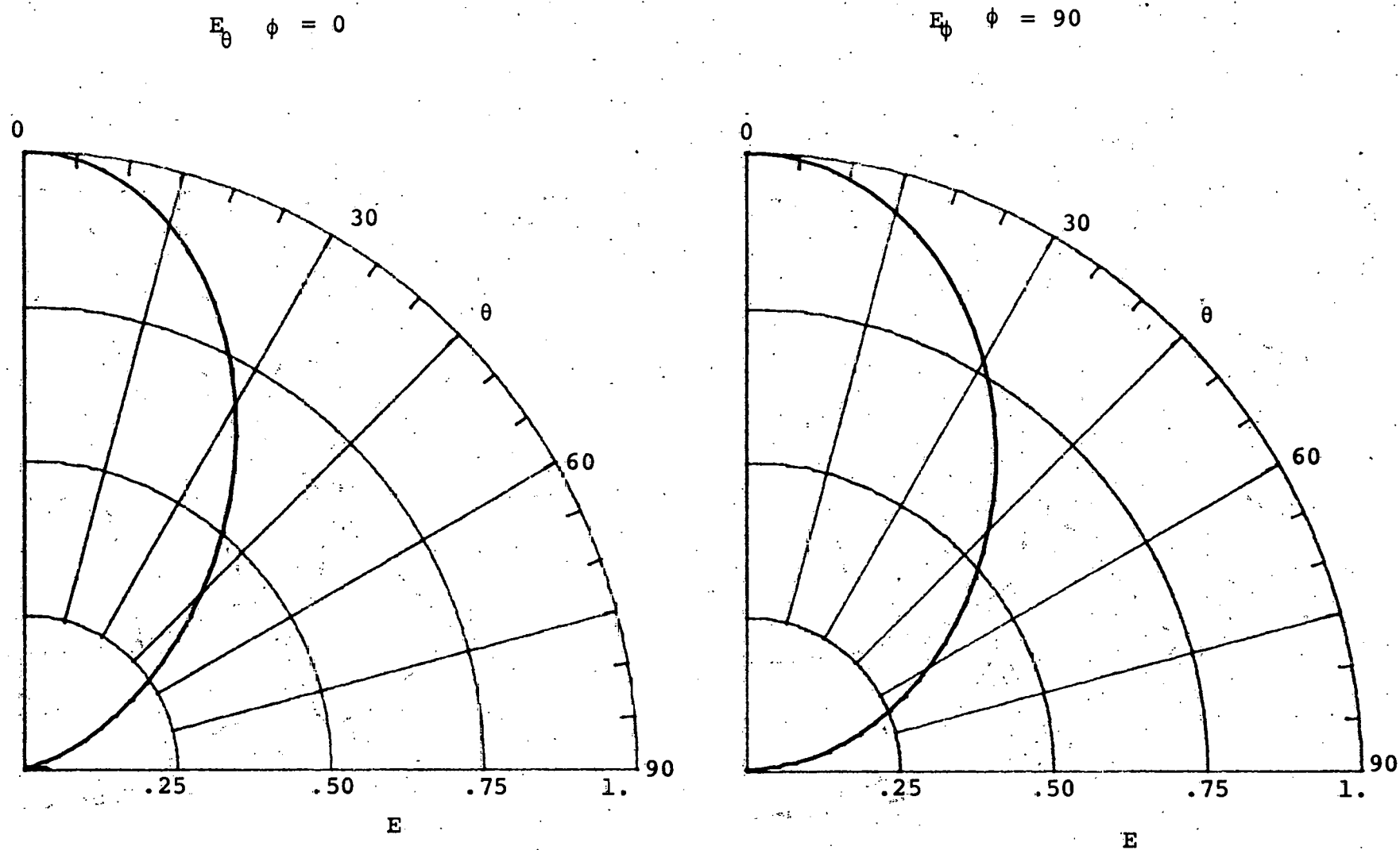
Figure 8. Circular Microstrip Antenna (r_o/\lambda = 0.3, \nu = 1)
