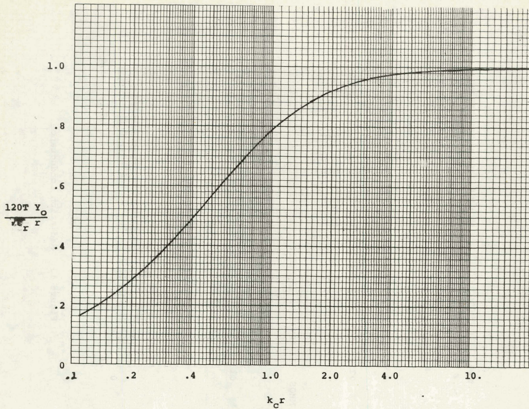
Figure 14. Normalized Characteristic Admittance
