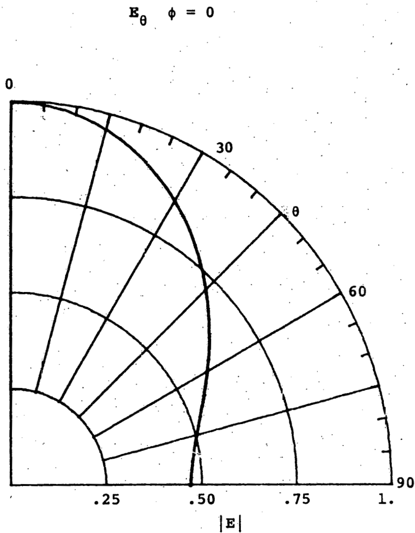
Figure 7. Circular Microstrip Antenna (r_o/\lambda = 0.2, \nu = 1)
