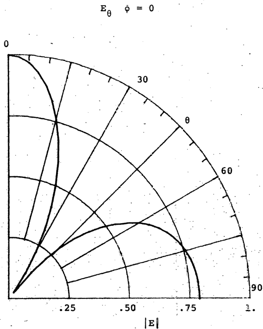
Figure 10. Circular Microstrip Antenna (r_o/\lambda = 0.5, \nu = 1)
