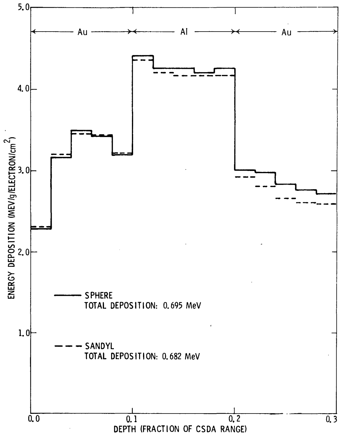
Figure 5. Comparison of electron energy deposition profiles calculated with the SPHERE and SANDYL codes.
