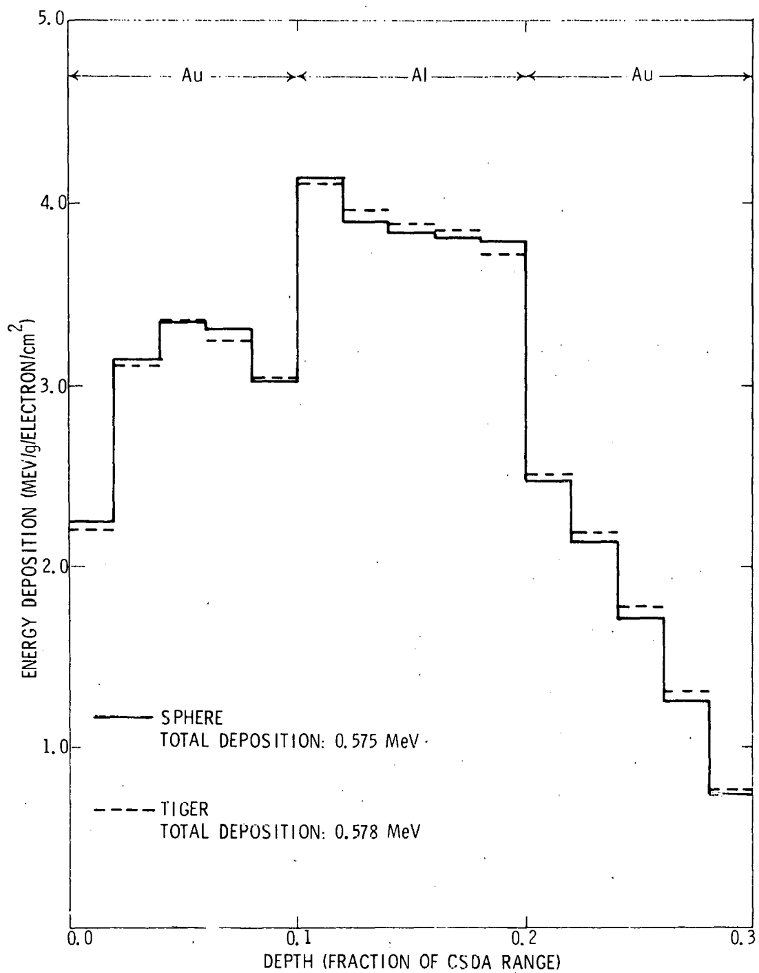
Figure 7. Comparison of electron energy deposition profiles calculated with the SPHERE and TIGER codes.
