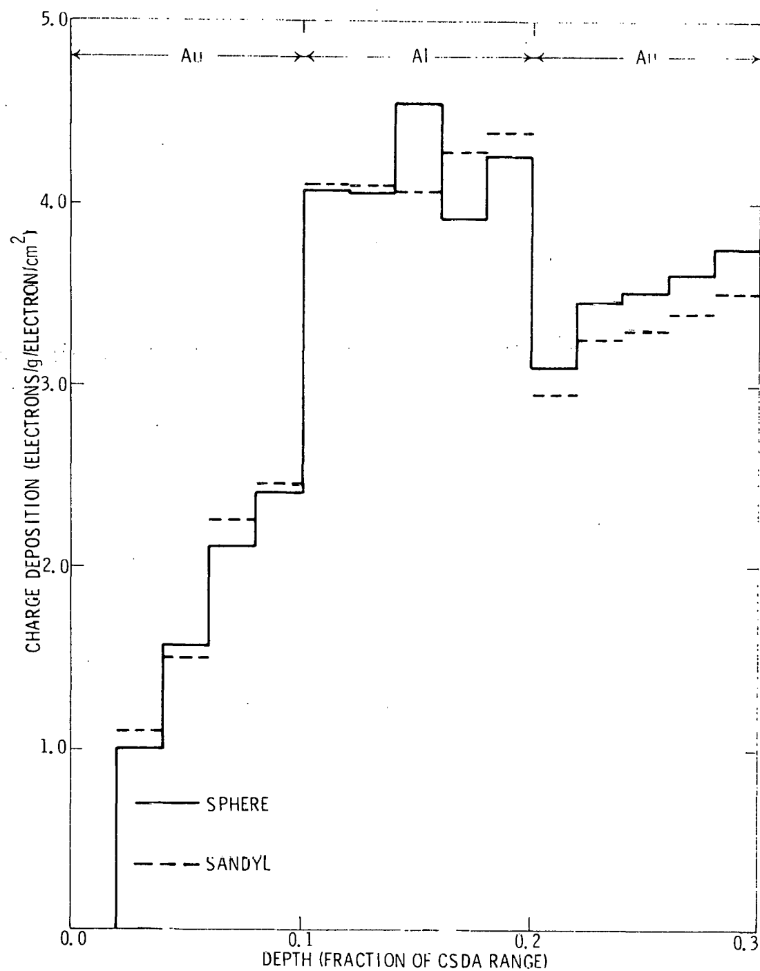
Figure 6. Comparison of electron charge deposition profiles calculated with the SPHERE and SANDYL codes.
