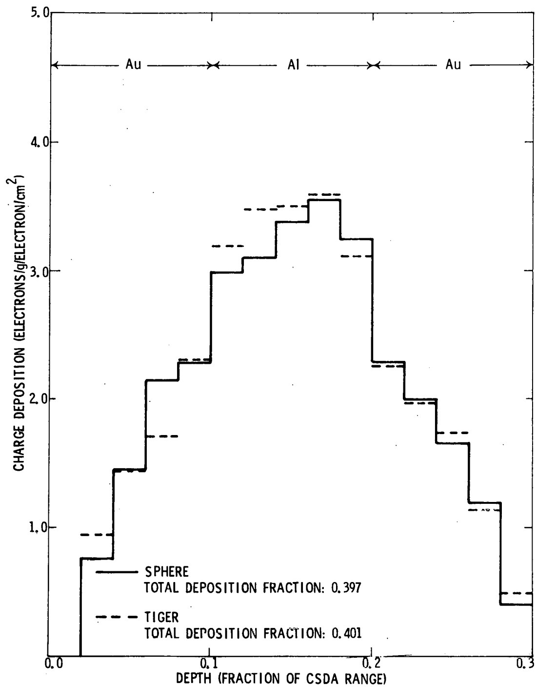
Figure 8. Comparison of electron charge deposition profiles calculated with the SPHERE and TIGER codes.
