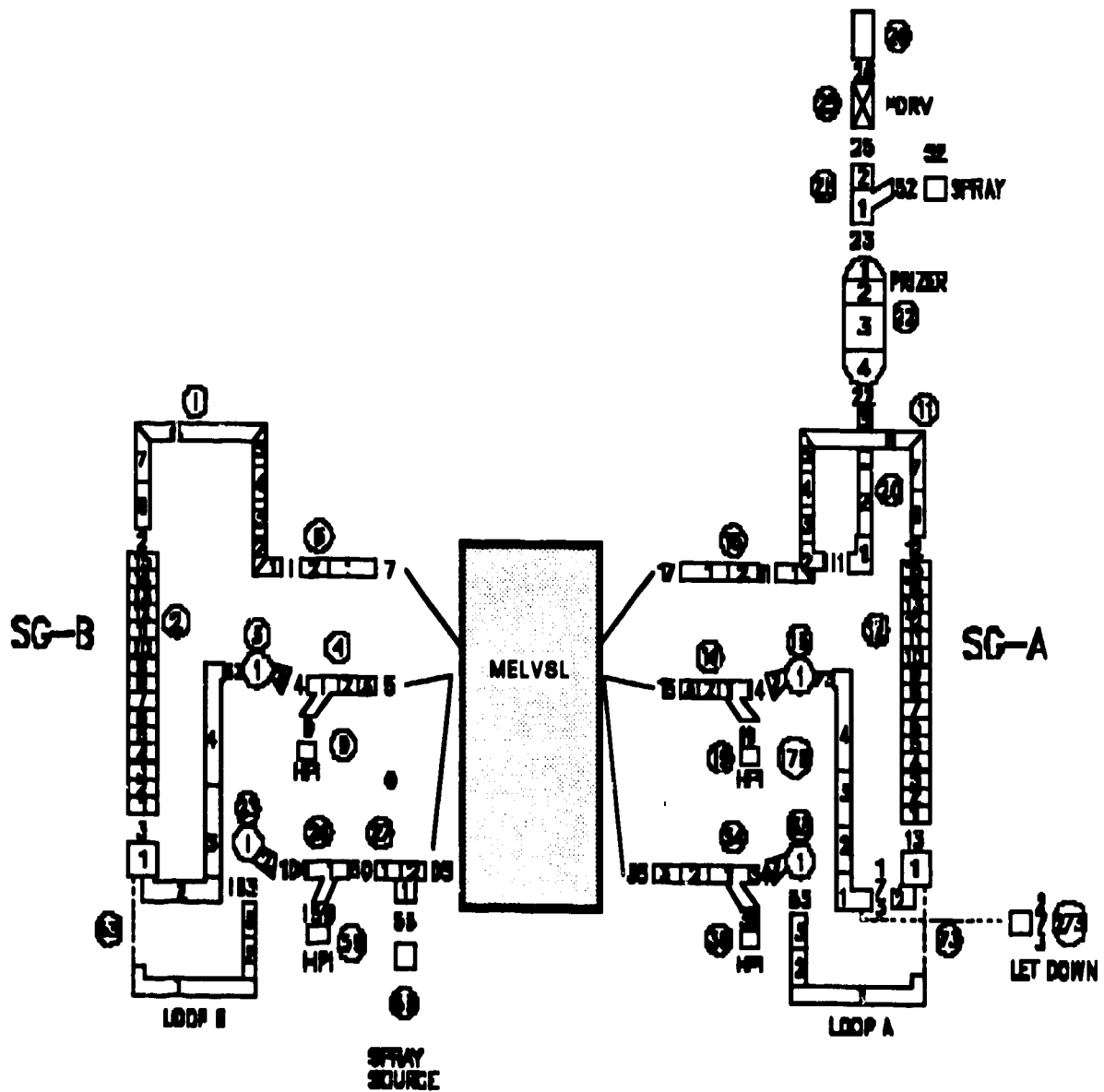
Figure 2. TMI-2 TRAC PRIMARY-SYSTEM MODEL
