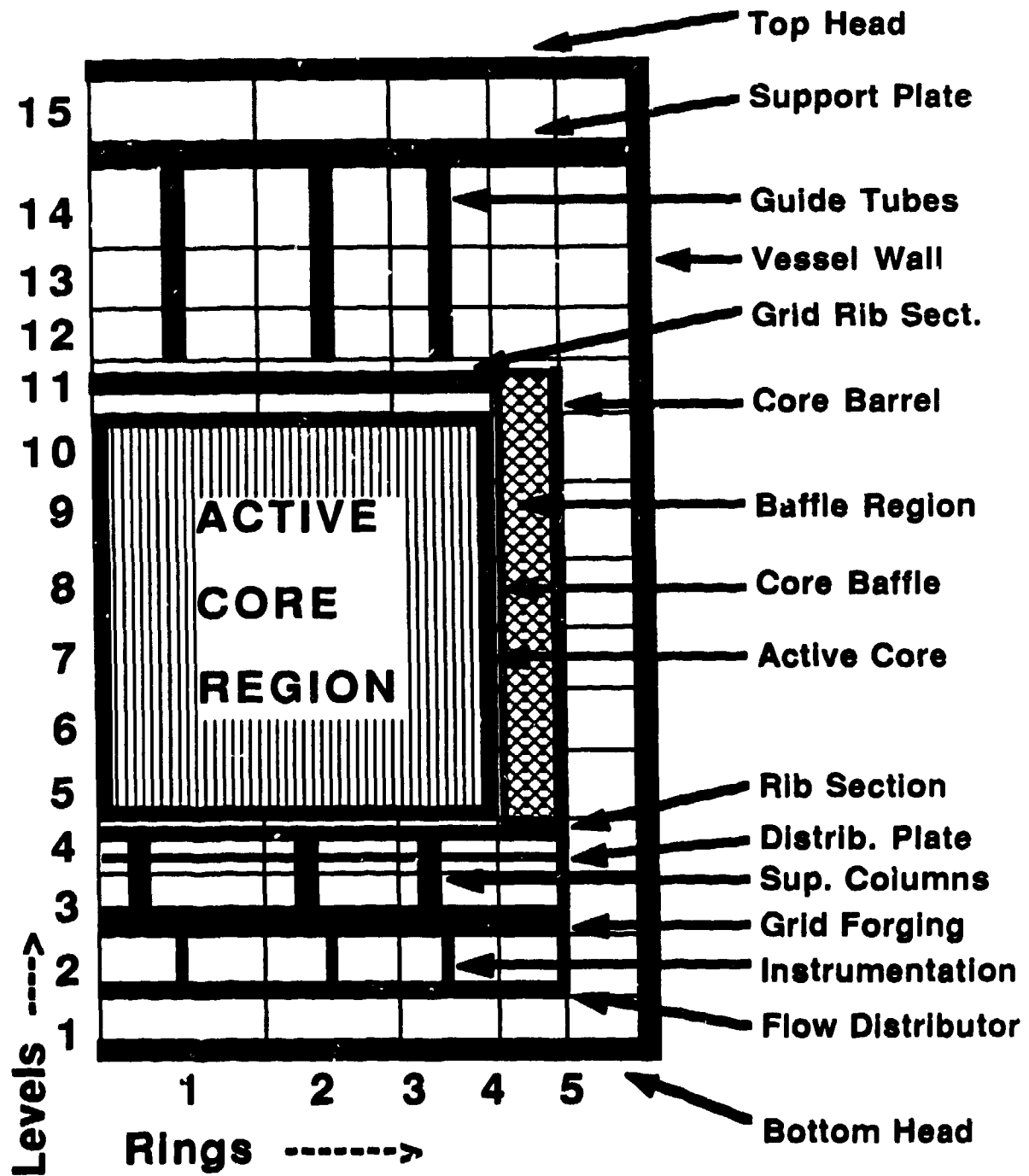
Figure 1. TMI-2 MELPROG VESSEL MODEL
