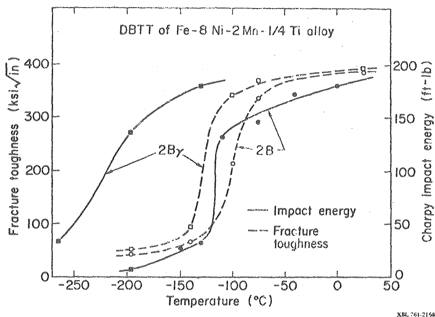
Fig. 5. Charpy impact and fracture toughness transition temperatures vs. treatment for Fe-8Ni-2Mn-0.25Ti. 2Br (= 2B + 600°C, 2 hrs.) has ~5% retained austenite.
