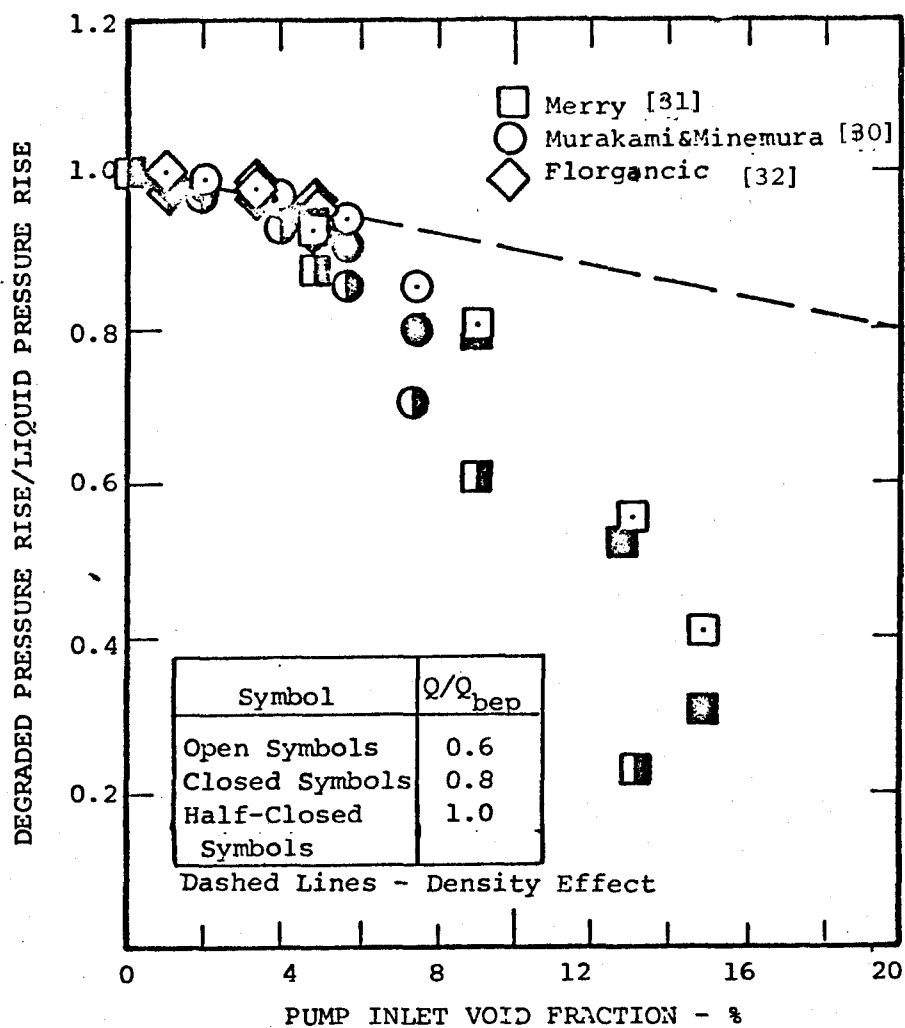
FIGURE 4-1. HEAD DEGRADATION UNDER AIR INGESTING CONDITIONS AS A FUNCTION OF INLET VOID FRACTION (% OF TOTAL FLOW RATE BY VOLUME).
