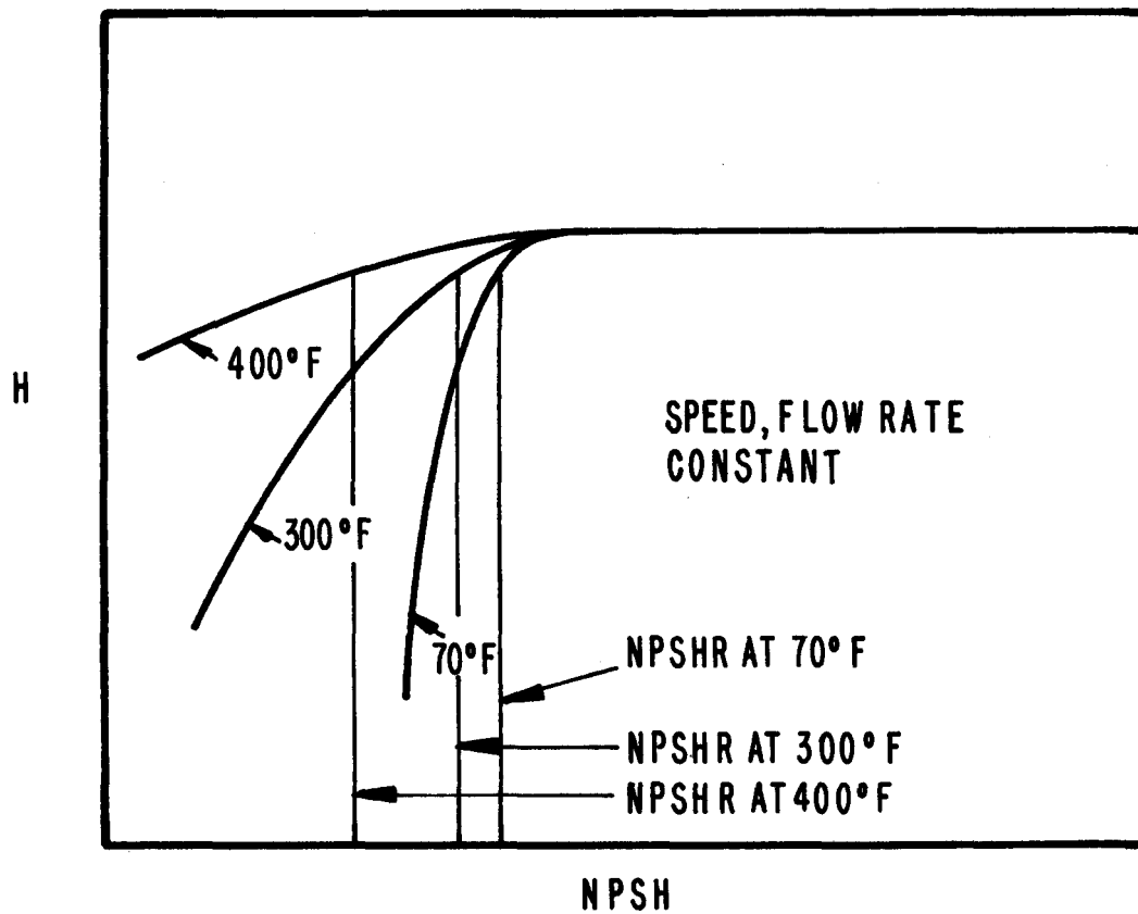
Figure 4-4. RELATIONSHIP BETWEEN PUMP CAVITATION AND WATER TEMPERATURE
