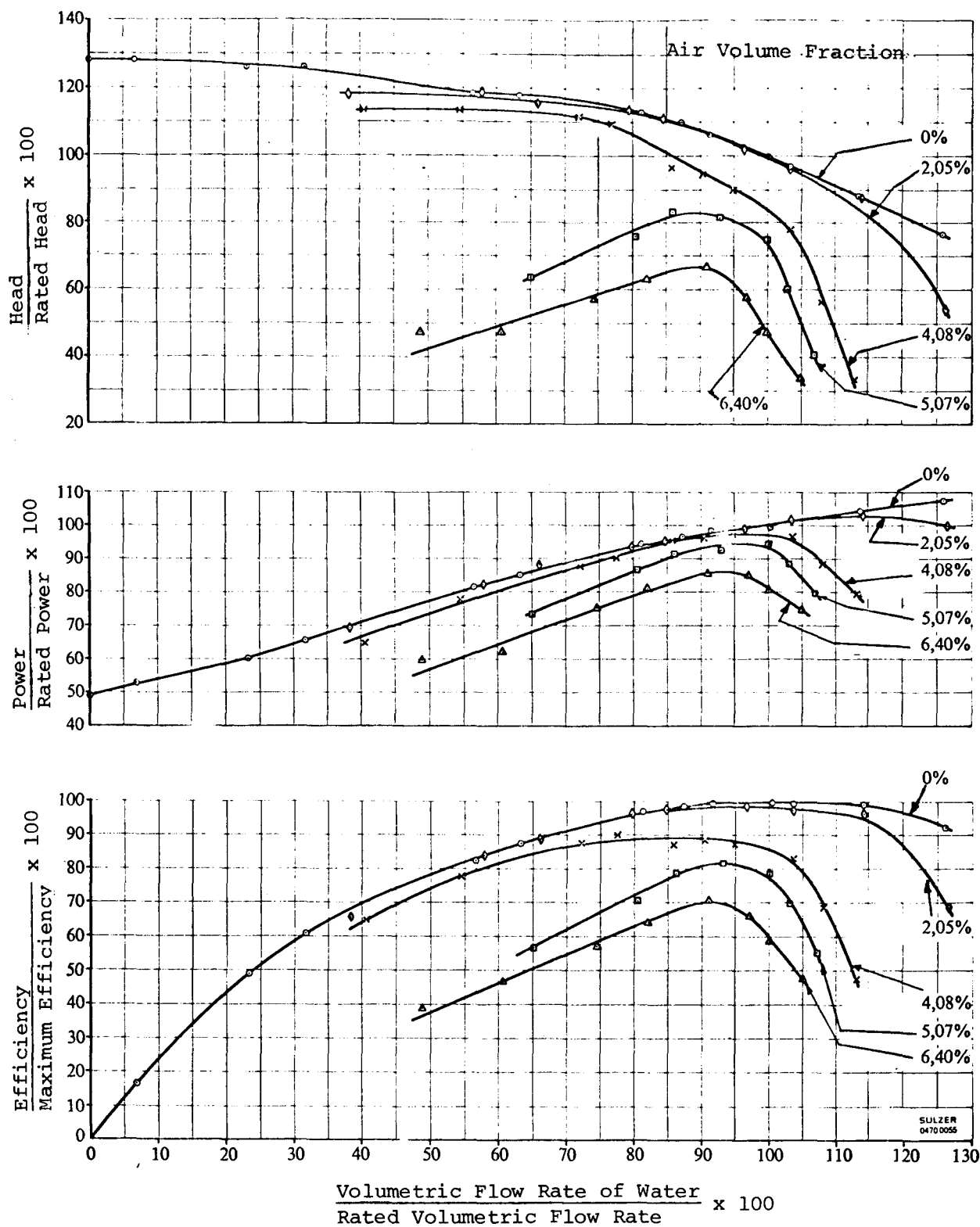
Figure 3-7. NORMALIZED HEAD, POWER AND EFFICIENCY IN AIR/WATER FLOW FROM FLORJANCIC [32]
