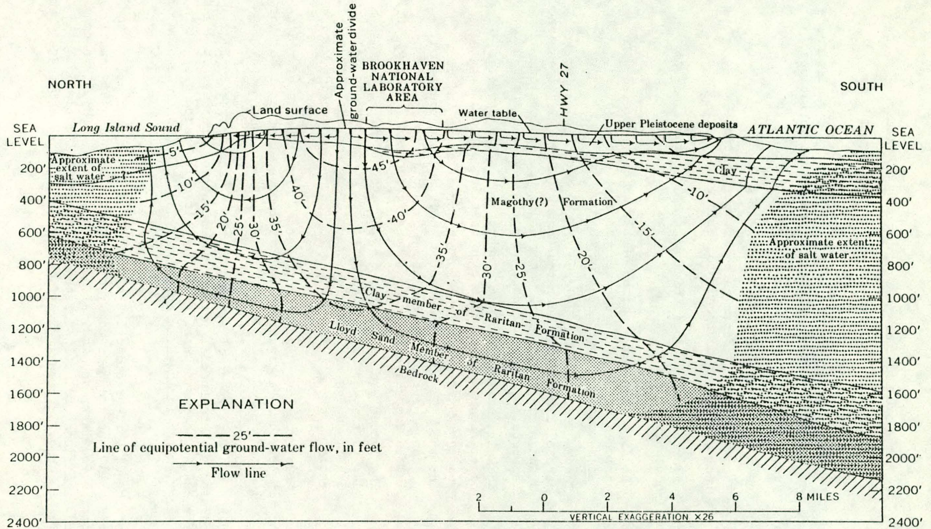
Schematic ground-water flow lines, central Upton area.
