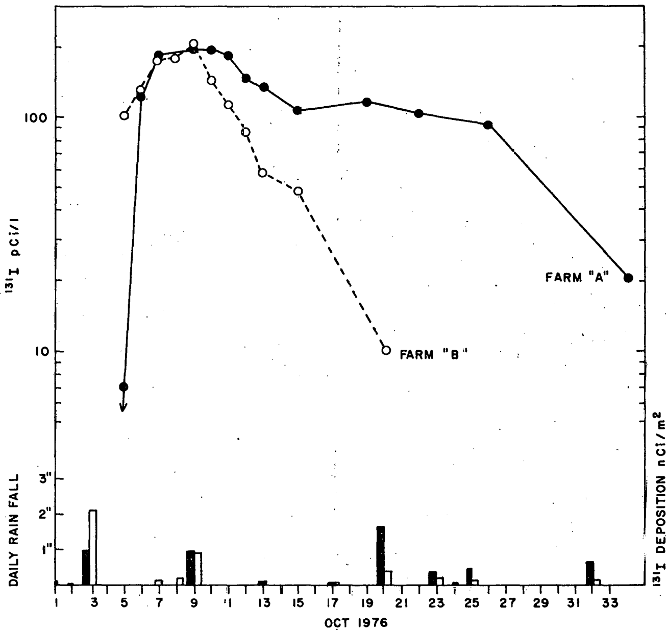
^{131}\text{I} Concentrations in Milk produced in Suffolk County following the Chinese test, September 26, 1976.
