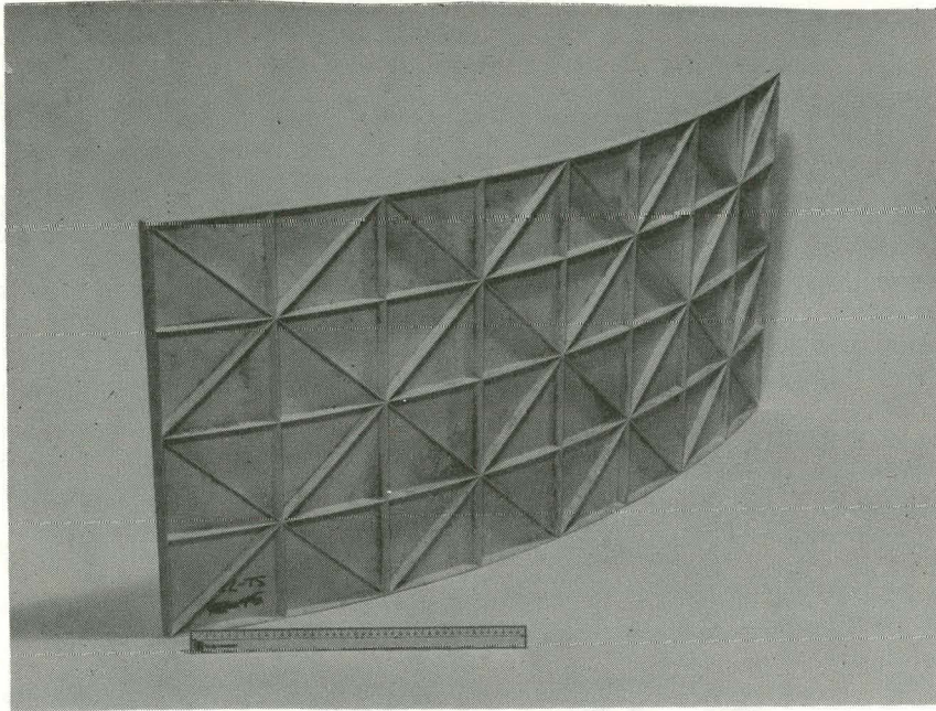
Figure 5. Early SMC Molded Reflector Panel
