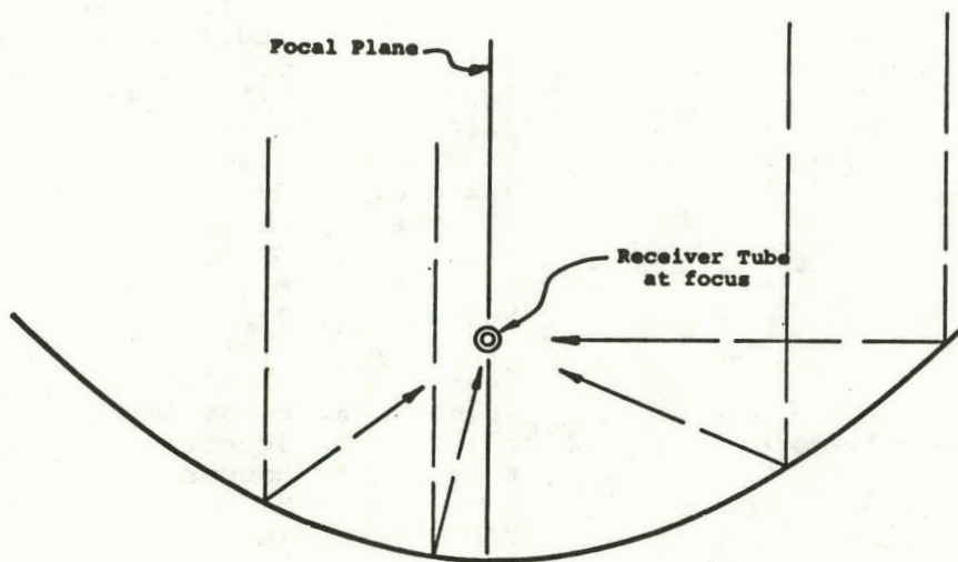
Figure 2. Parabolic Reflector
