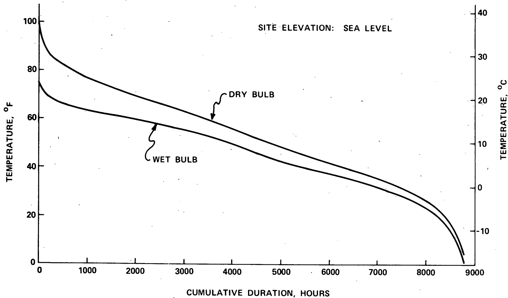
FIGURE 13-1 TEMPERATURE DURATION CURVES: MIDDLETOWN, U.S.A.
