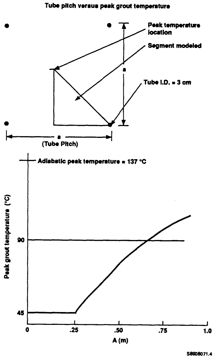
Fig. 5. Tube Pitch Versus Peak Grout Temperature.
