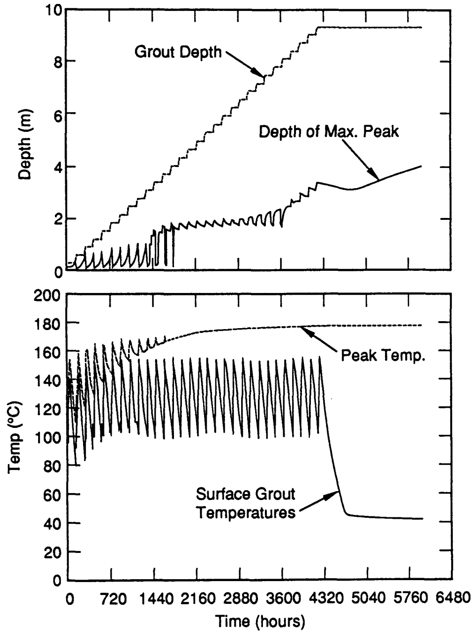
Fig. 7. Depth of Grout and Grout Temperatures for Staged Pour Scenario.
