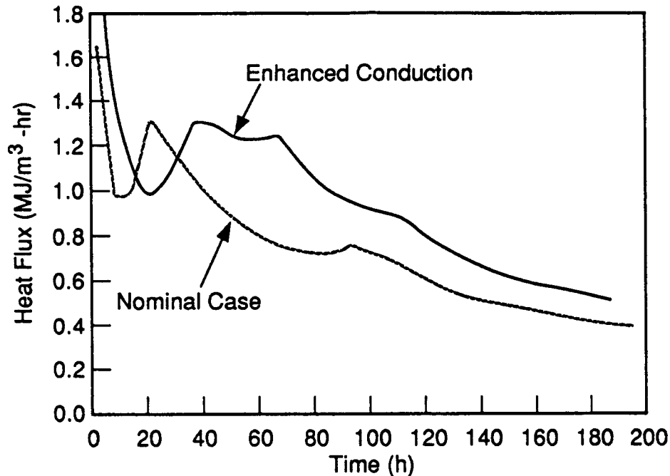
Fig. 6. Comparison of Surface Heat Flux Between Nominal Case and Enhanced Conduction Case.
