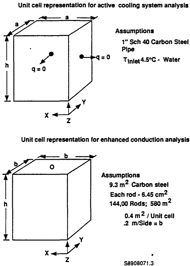
Fig. 4. Unit Cell Representations.
