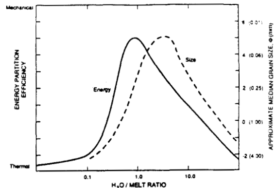
Figure 1. Results of water/magma interaction experiments showing the affect of water:melt mass ratio on explosive energy and fragment size (adapted from Frazzetta et al., 1983).
