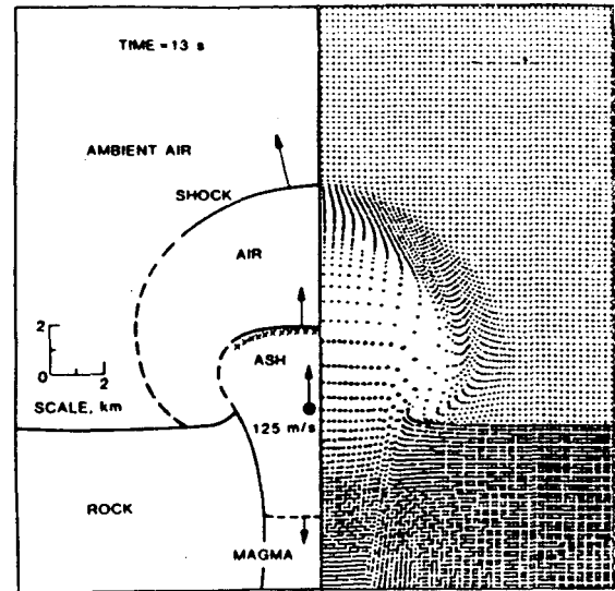
Figure 3. Representation of a volcanic blast eruption predicted by numerical simulation of an overpressured eruption. The right-hand side of the plot shows calculated ash and atmospheric marker particles (Wohletz and others, 1984).
