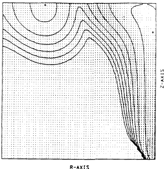
Figure 4. Simulated Plinian eruption column portrayed as contours of volume fraction of volcanic ash. Dots and lines are nodal dust velocity vectors. Note axisymmetry around the vent (lower right) and the 7X7 km calculational regime.
