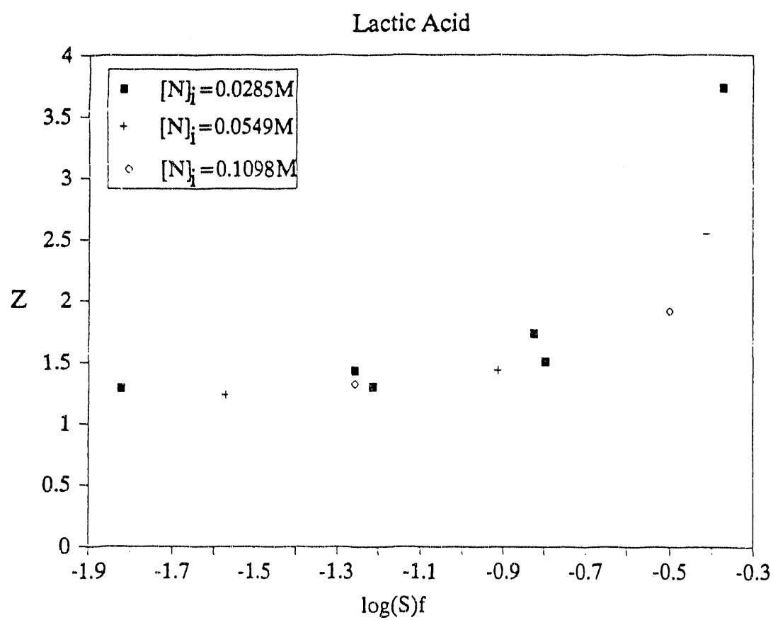
Fig.7.15 Lactic acid extraction results expressed in the form of a loading curve
