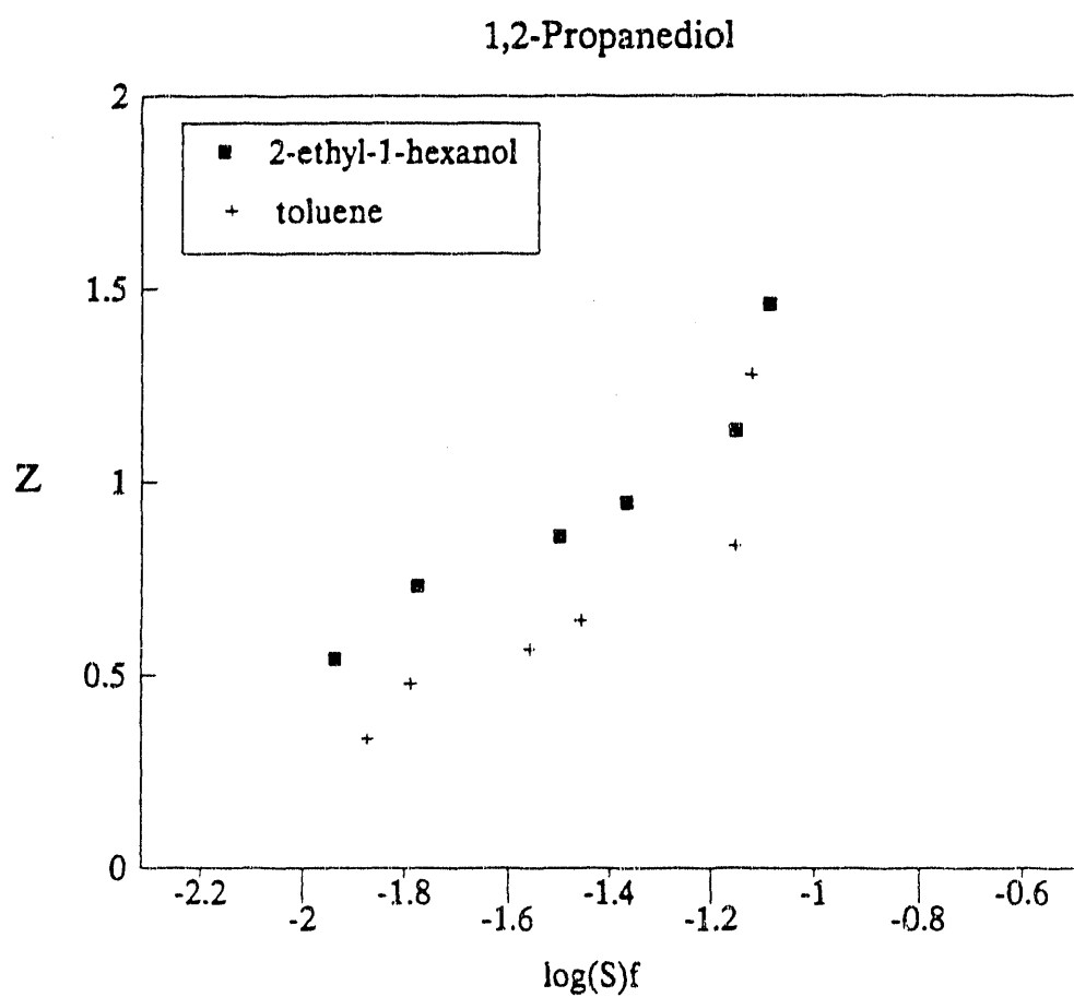
Fig. 7.14 Comparing extraction results for 1,2 propanediol obtained by using two different diluents
