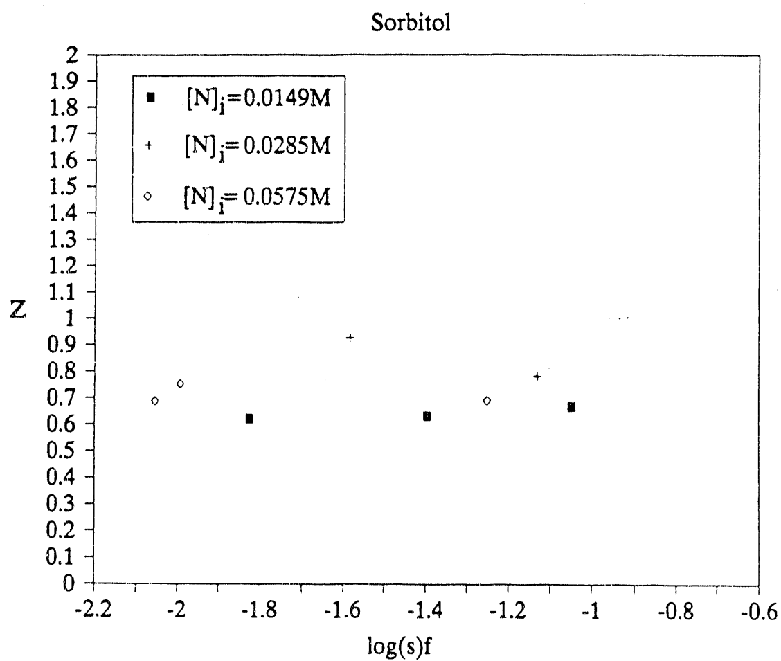
Fig. 7.8 Extraction results for sorbitol expressed in the form of loading curve
