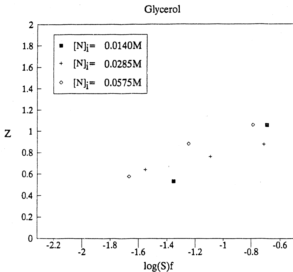
Fig. 7.1 Glycerol extraction results expressed in the form of a loading curve
