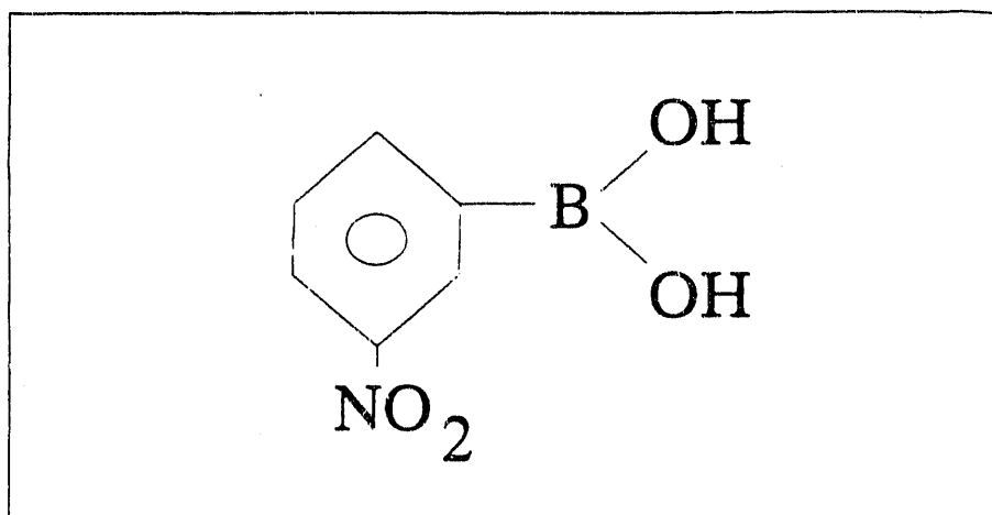
Fig.2.1 Molecular structure of NPBA
