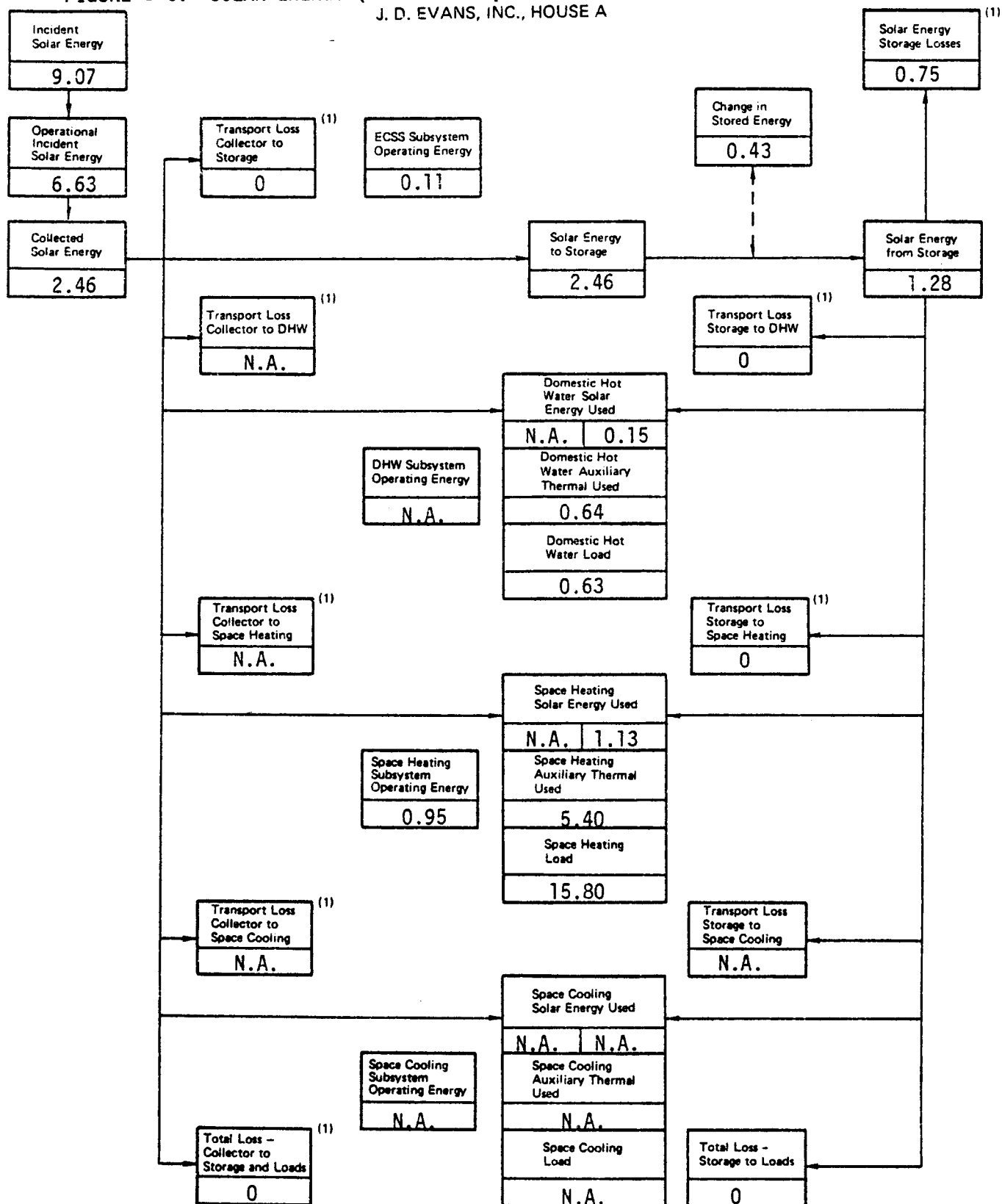
FIGURE D-3. SOLAR ENERGY (MILLION BTU) DISTRIBUTION FLOWCHART - FEBRUARY 1979 J. D. EVANS, INC., HOUSE A
