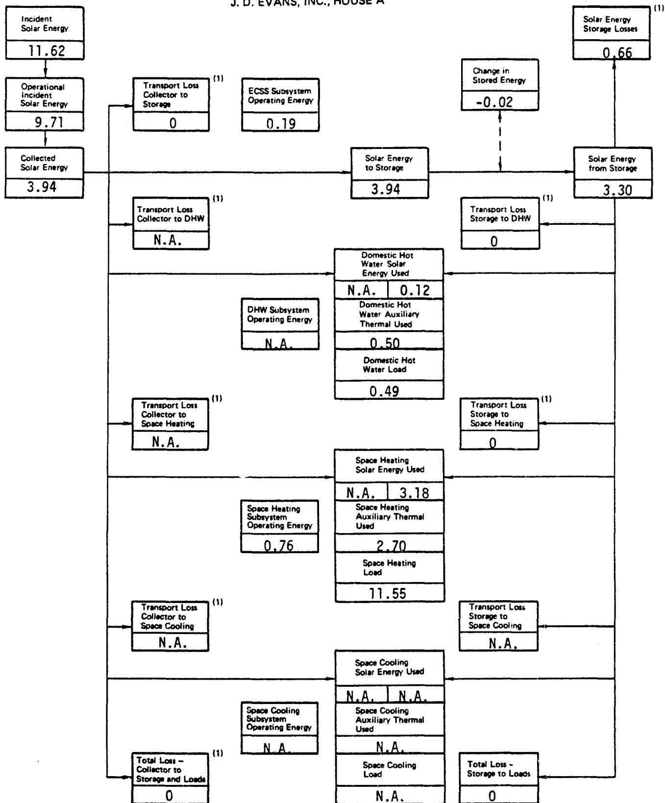
FIGURE D-2. SOLAR ENERGY (MILLION BTU DISTRIBUTION FLOWCHART - DECEMBER 1978 J. D. EVANS, INC., HOUSE A
