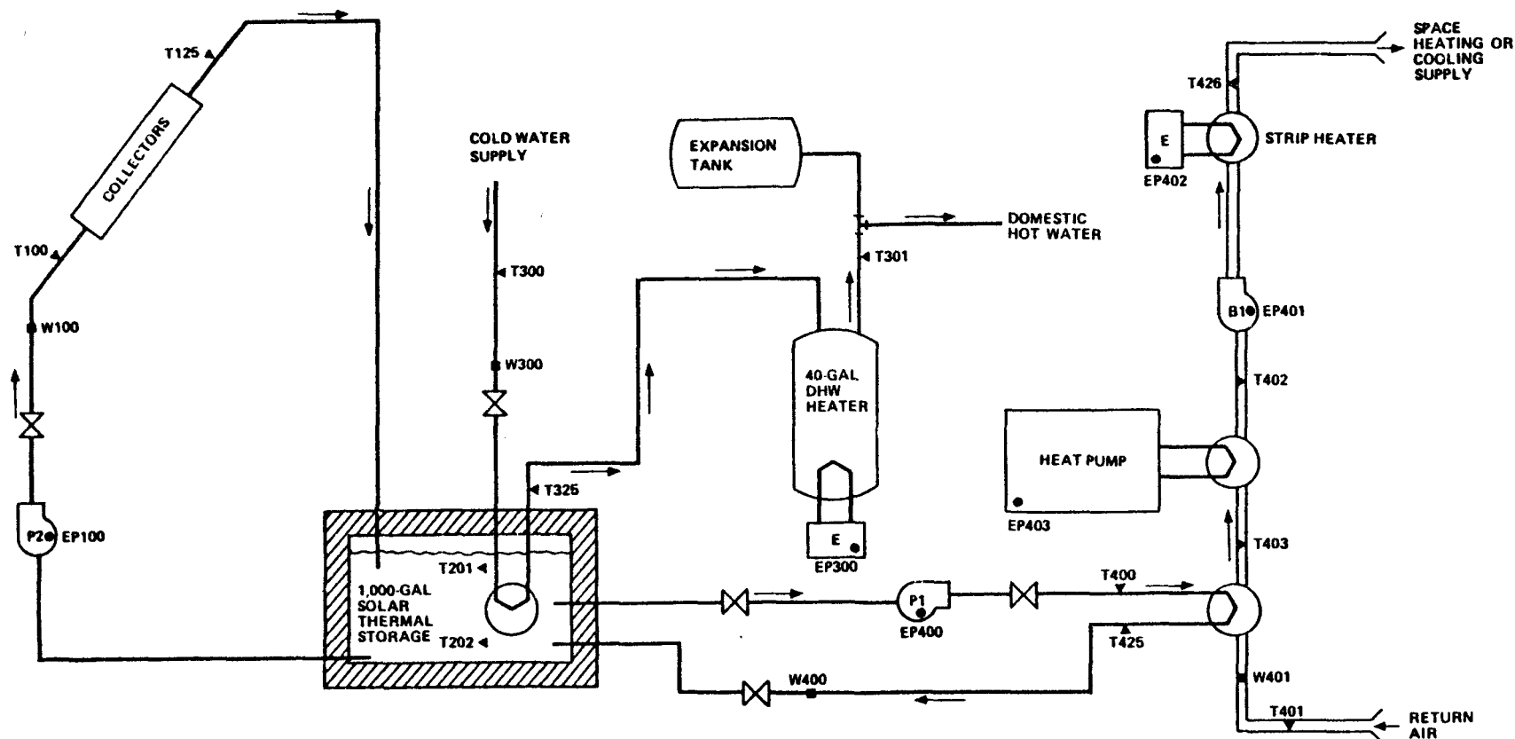
FIGURE 3-1. SOLAR ENERGY SYSTEM SCHEMATIC J. D. EVANS, INC., HOUSE A
