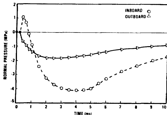
Figure 4. Normal Pressure Time History, Inboard Plasma Motion, Extraordinary Disruption
