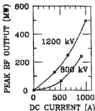
FIG. 1. MASK simulations of SL4.
