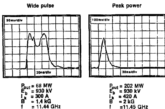
FIG. 2. Low and high peak power pulses in SL4 tests.
