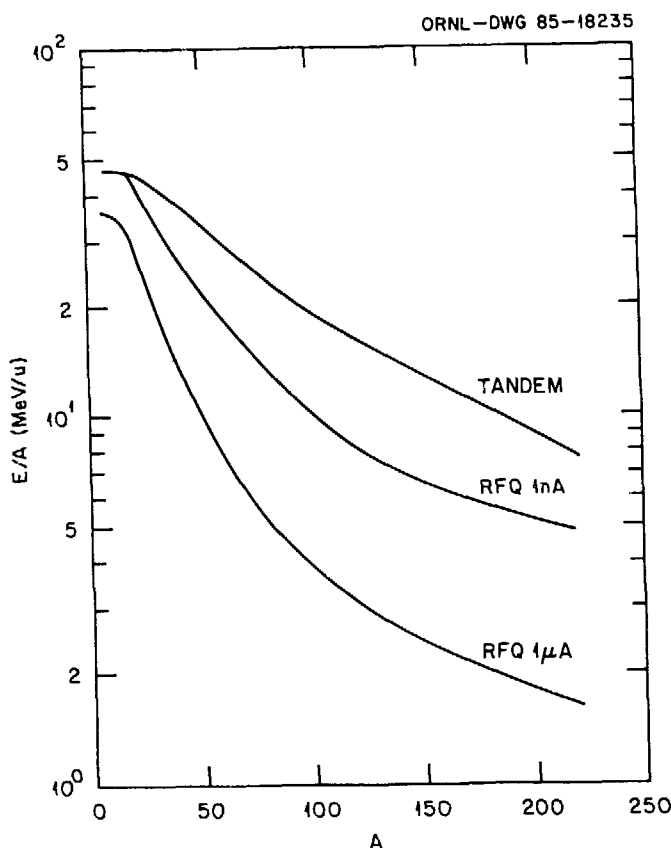
Fig. 4. Maximum ion energy from HISTRAP as a function of mass number with injection from either the tandem accelerator or injection from the ECR and RFQ preaccelerator. For injection from the RFQ two cases are shown: a high-charge-state low-current case (1 nA) and a low-charge-state high-current case (1 \mu A).
