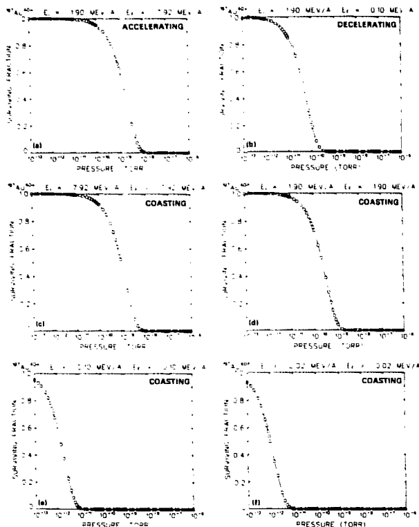
Fig. 7. The surviving fraction for tandem-injected Au beams as a function of vacuum system pressure for various HISTRAP operating modes. The residual gas was assumed to be 90% H 2 and 10% N 2 . E i and E f are the initial and final kinetic energies per nucleon, respectively.
