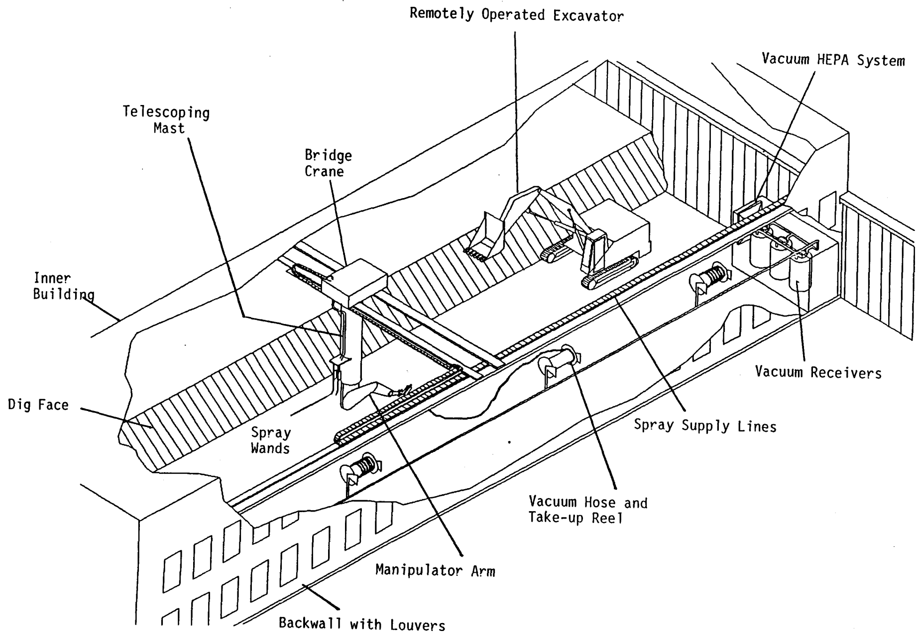
Figure 1. Inner Building with Dust Suppression System
