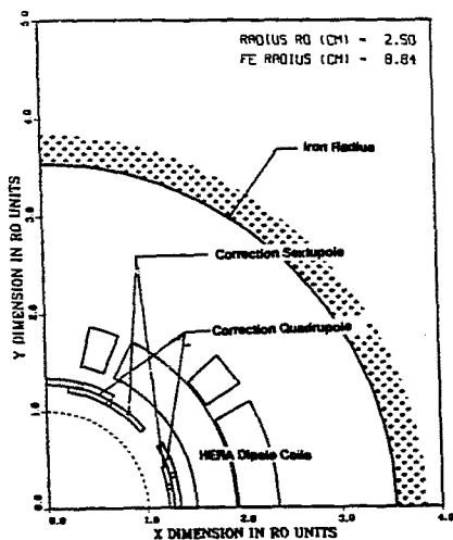
Fig. 1 A quarter cross-section of the HERA dipole showing the dipole coils, the quadrupole corrector and the sextupole corrector.
