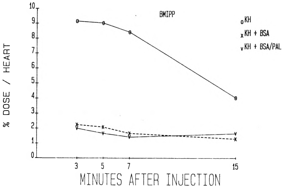
Figure 1. Effects of buffer solution composition on the global retention of [I-125]BMIPP.
