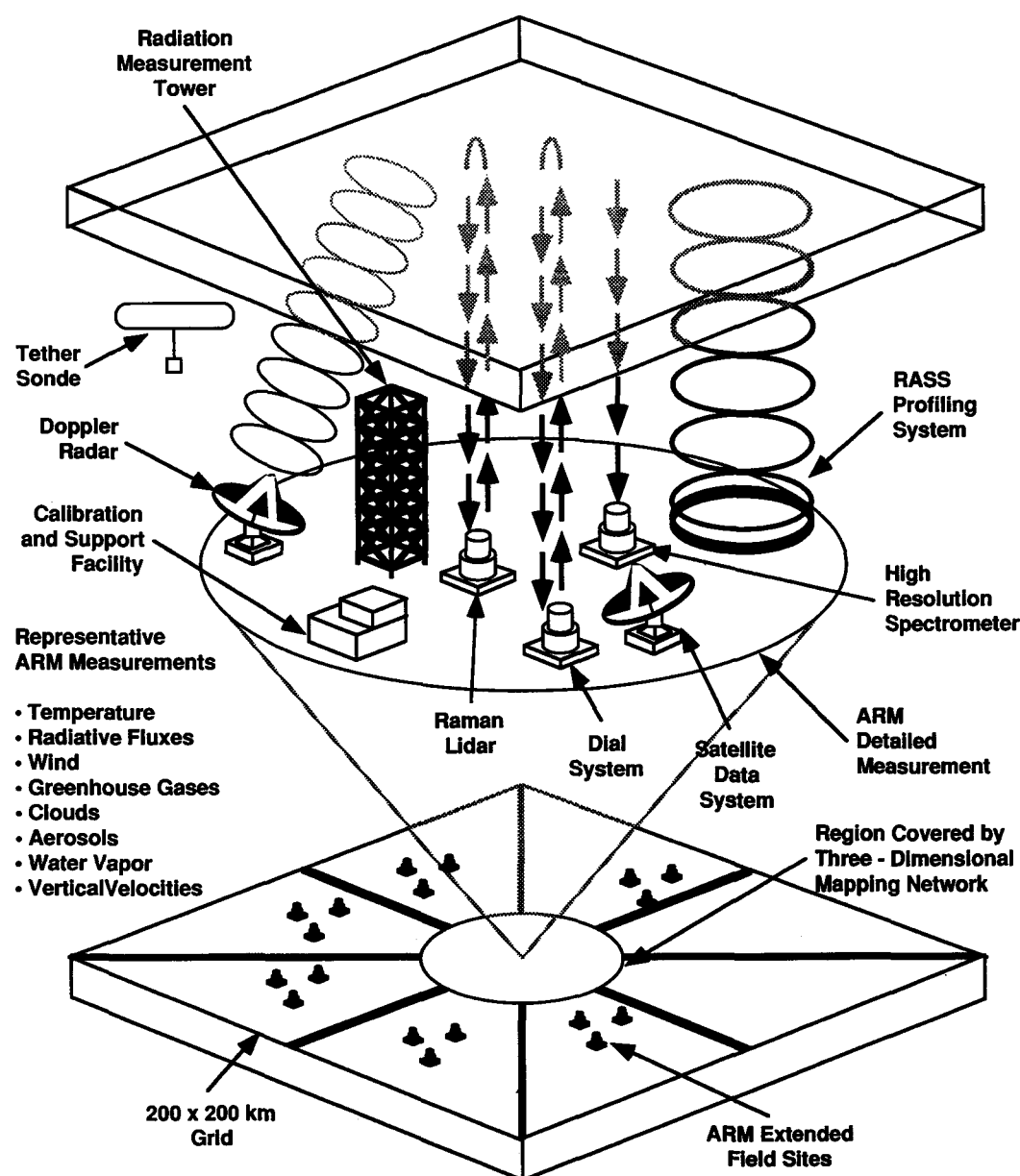
Figure 2. The ARM experimental configuration. An ARM site will have three components as described in the text. The central facility, for which representative equipment is shown, will be supported by a system for mapping the three-dimensional distribution of meteorological variables. In addition, 16 to 25 sets of instrumentation will provide critical data for understanding how to generalize the results to the 200 x 200 km GCM grid size.
