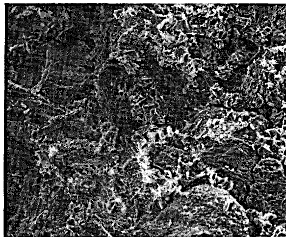
Figure 6. Cerro Prieto well NL-1, 2720 m depth. Sample showing clay platelets in both angular orientation and in the "book leaves" fabric. This sandstone illustrates the accicular clay fabric intermingled with the platelets, which show EDAX values of Fe 37%, Si 33%, K 15%, Al 9%, and Mg 6%.
