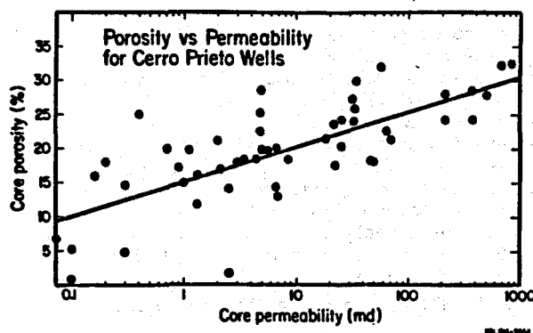
Figure 4. Permeability and porosity values for 55 Cerro Prieto cores.
