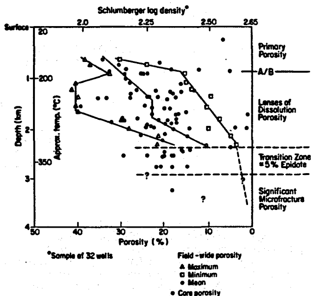
Figure 3. Field-wide porosity values for Cerro Prieto.
