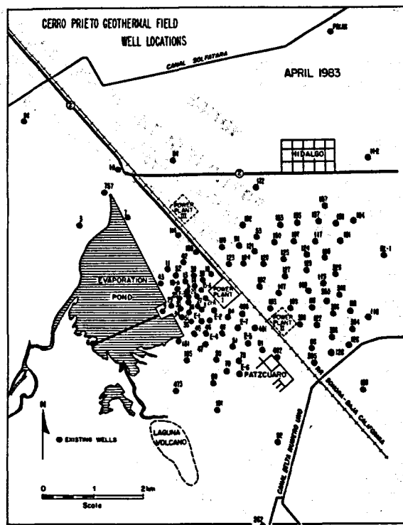
Figure 2. Cerro Prieto well locations.
