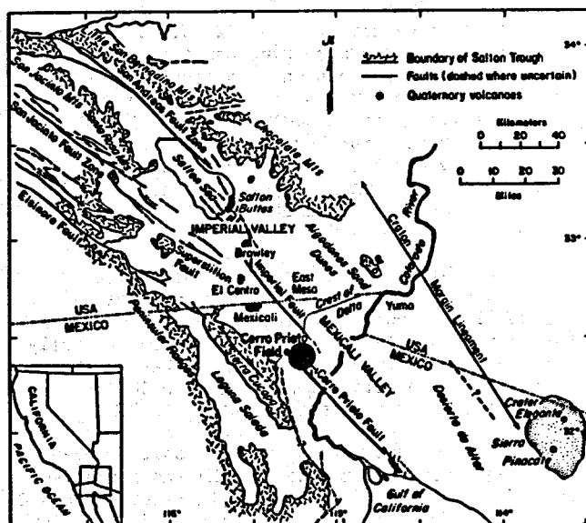
Figure 1. Location of the Cerro Prieto geothermal field in the Salton Trough.
