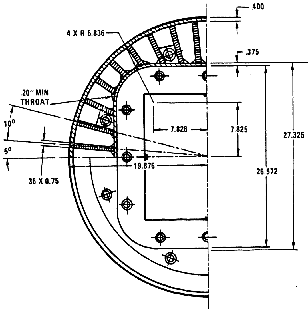
Fig. 3 Top View of GA-4 Closure-End Impact Limiter Support Structure
