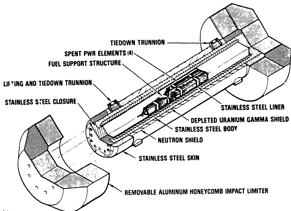
Fig. 1 GA-4 Cask Exploded View
