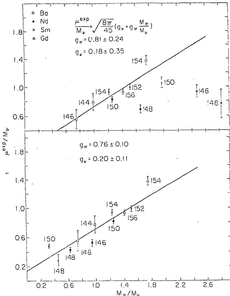
Fig. 7. Values of \mu^{\text{exp}}/M_v versus M_\pi/M_v for 2^+_{11} states in Ba, Nd, Sm and Gd. The upper portion assumes a Z=50-82 shell for all N , whereas the lower portion assumes Z=50-64 for N < 88 and Z=50-82 for N > 90 .
