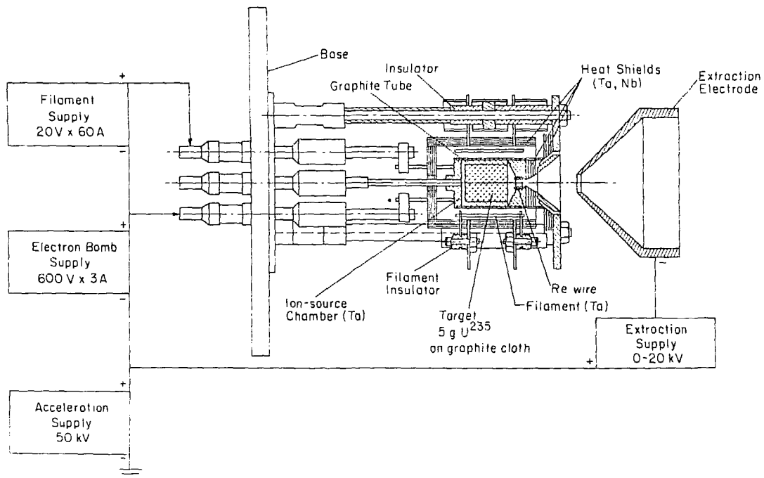
Fig. 3 The TRISTAN thermal ion source, showing the construction common to the family of sources.
