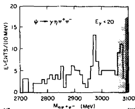
Fig. 28. The m_{\eta\pi^+\pi^-} distribution for the candidates
