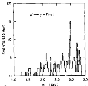
Fig. 27. The m_{\text{final}} distribution for the candidates \psi' \rightarrow \gamma + \text{Final} .
