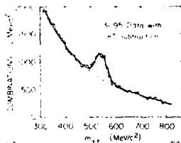
Fig. 15. The \pi^0 -subtracted m_{\gamma\gamma} spectrum of Fig. 14.
