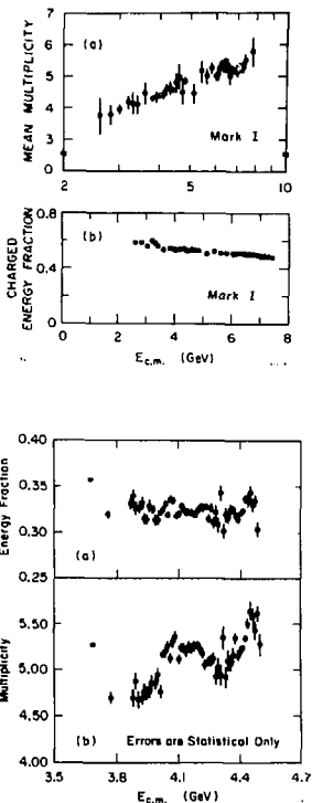
Fig. 10. Inclusive Quantities in the Crystal Ball Scan Mode: a) Neutral energy fraction, b) Neutral Multiplicity (Ref. 19).
