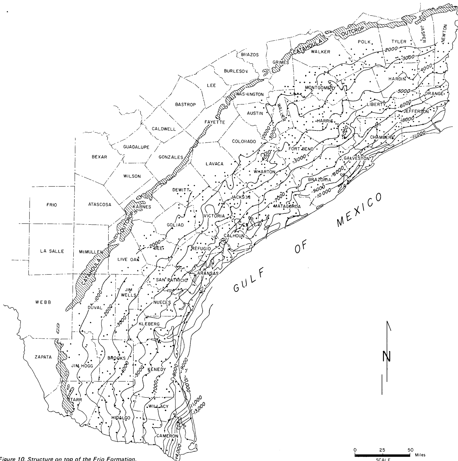
Figure 10. Structure on top of the Frio Formation.
