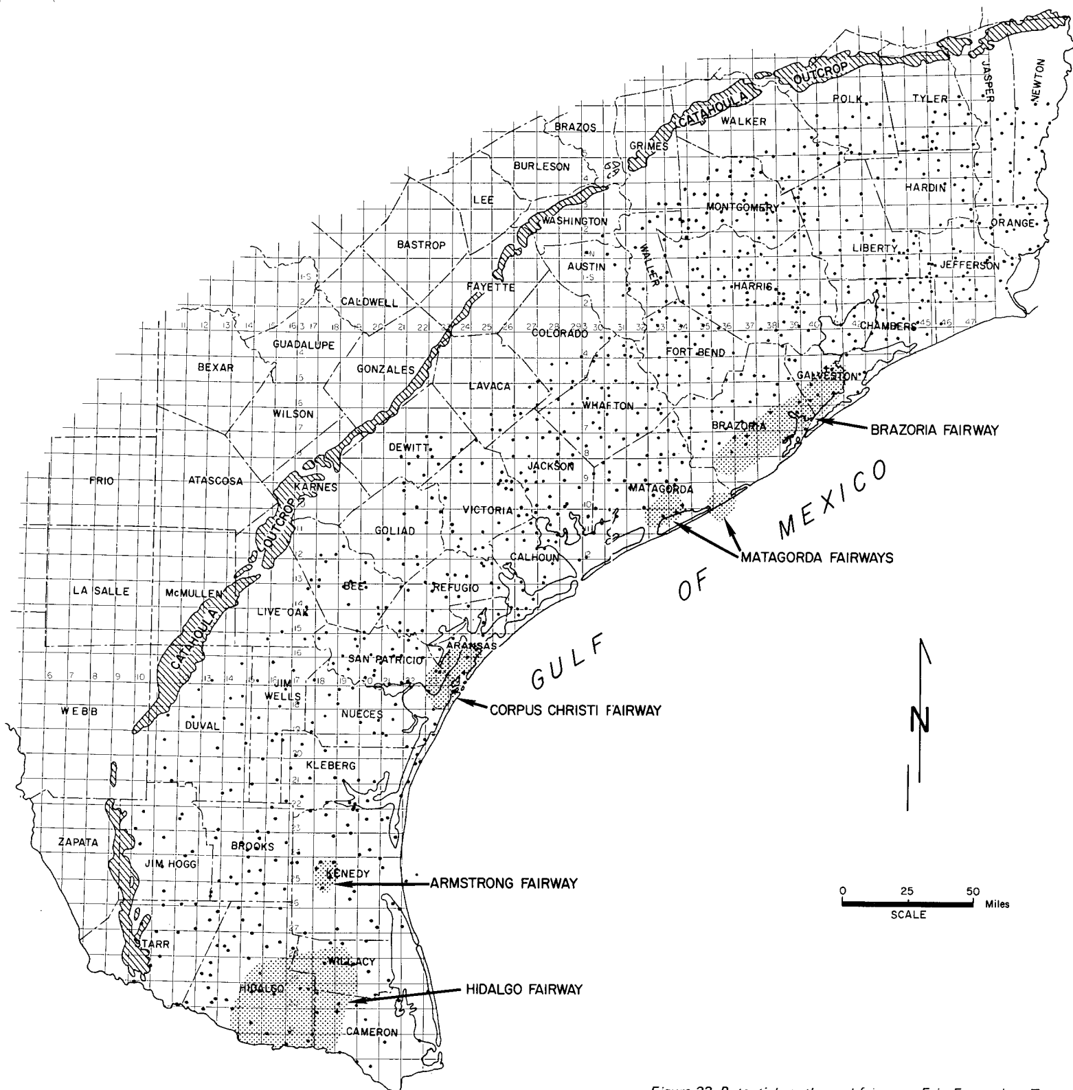
Figure 22. Potential geothermal fairways, Frio Formation, Texas Gulf Coast.
