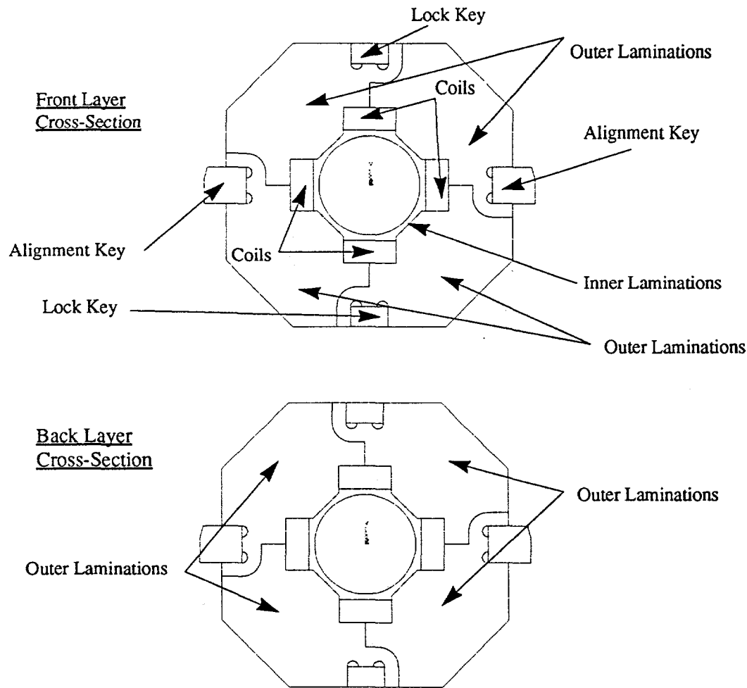
Figure 1. Collider 50mm Aperture Ordered Wound Quadrupoles - Front and Back Layer Cross-Sections
