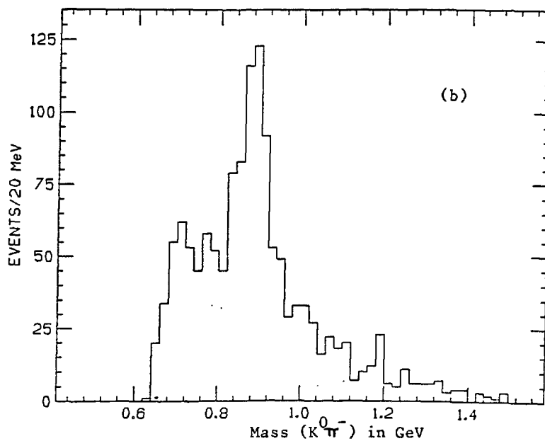
Figure 7. K^-p \rightarrow K^+K^0\pi^- X at 8 GeV/c and -t < 1.0 \text{ (GeV/c)}^2
