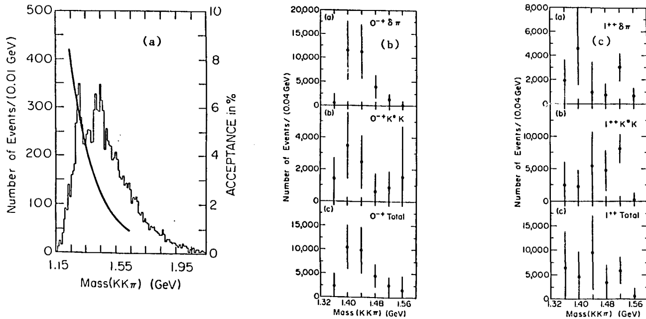
Figure 6. \bar{p}p \rightarrow K^+ K^0 \pi^- X at 6.6 GeV/c. a) K^+ K^0 \pi^- mass; smooth curve is acceptance. b) and c) Intensities of J^{PG} waves.
