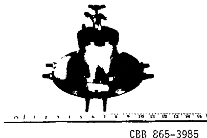
Fig. 6 A small multicusp H^- source.
