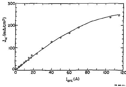
Fig. 7 Extracted H - current density versus arc current.
