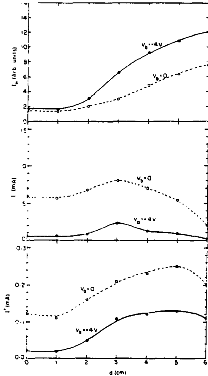
Fig. 2 H^- yield and the extracted electron and positive ion current as a function of the extractor position.
