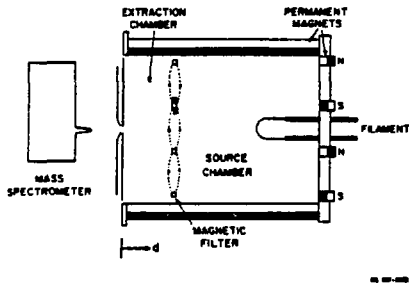
Fig. 1 Schematic of the multicusp ion source equipped with a magnetic filter.
