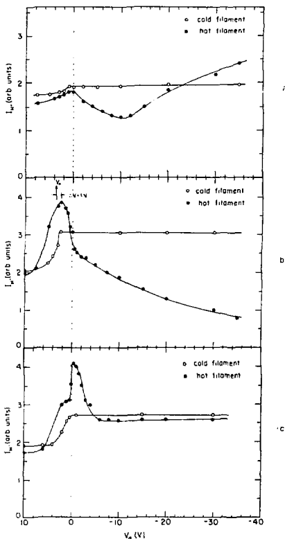
Fig. 5 H^- yield as a function of the discharge voltage of the second filament when it is installed inside (a) the source chamber, (b) the extraction chamber, and (c) the filter region. The data shows the H^- yield when the filament is operated with the without electron emission.
