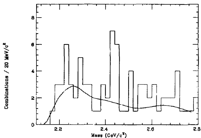
Figure 6.16. \Omega^- K^+ invariant mass plot. The solid line is the predicted background taken from Monte Carlo.
