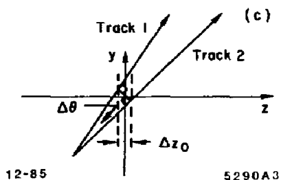
Figure 5.1. Pair finding algorithm geometry. RCOS is the cosine of the angle between R_{xy} and P_{xy} of the pair.
