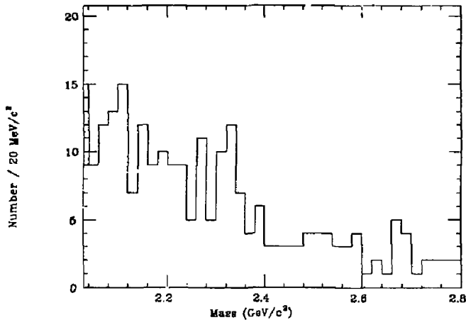
Figure 6.14. proton K_s invariant mass combinations.
