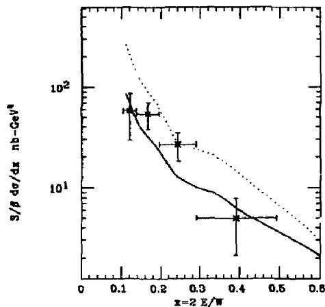
Figure 5.8. Inclusive cross section for \Xi^- + \Xi^{+\prime} . The solid points are the \Xi . The solid and dotted lines are the Lund string and Webber cluster model predictions, respectively.
