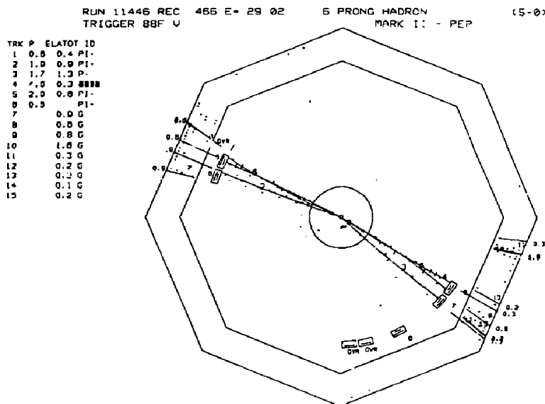
Figure 6.9. A candidate for e^+e^- \rightarrow \Lambda_c^+ \bar{\Lambda}_c^- \pi^0 . One \Lambda_c^+ decays semileptonically, the other decays hadronically to pK\pi\pi^0 . This event is not otherwise included in this analysis, because the \Lambda only satisfied the cuts if PTRAKR tracking was used; with SUPTRKR, one of the \Lambda tracks came too close to the origin. Since the PTRAKR track had a much lower \chi^2 , 8.5 for 6 degrees of freedom, compared with 42.1 for 7 degrees of freedom for SUPTRKR, I believe that PTRAKR found the track properly, and it really is a \Lambda .
