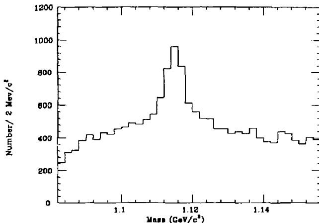
Figure 5.3. A mass peak for \Xi^- analysis.
