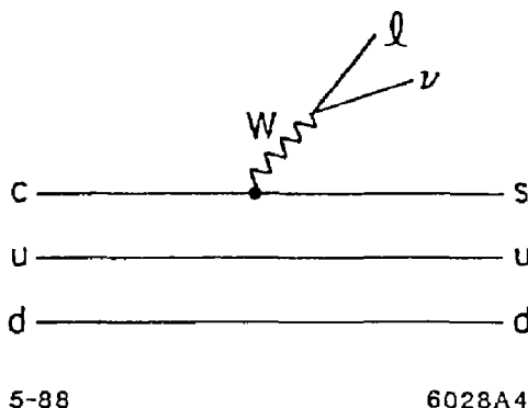
Figure 6.4. Feynman diagram for \Lambda_c^+ semileptonic decay.
