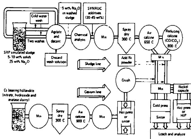
Fig. 4. Flow Diagram for Laboratory Scale Production of SYNROC D
