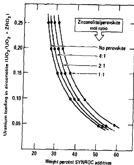
Fig. 3. Weight percent SYNROC D additives for SRP composite sludge plotted as a function of uranium loading in zirconolite and the desired zirconolite/perovskite ratio. Additives are TiO_2 (Z,P, spinel), CaO (Z,P), ZrO_2 (Z), and SiO_2 (nepheline).
