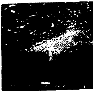
Fig. 1b. SEM photomicrograph of SYNROC D with granule of presynthesized hollandite. Matrix of SYNROC D consists of zirconolite, perovskite, spinel, nepheline and nickel metal. Scale bar is 10 microns.
