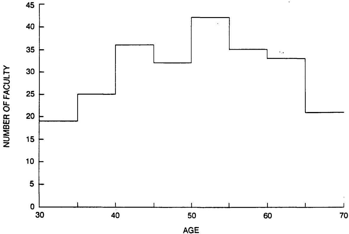
FIGURE 4-1 Distribution of nuclear engineering faculty by age. SOURCE: Committee survey (see Appendixes G and F).
