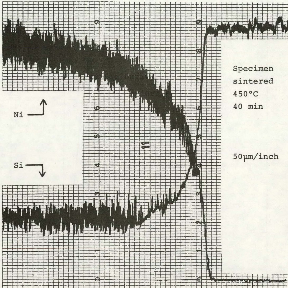
Figure 4. Electron microprobe scan of specimen sintered for 40 min at 450°C.
