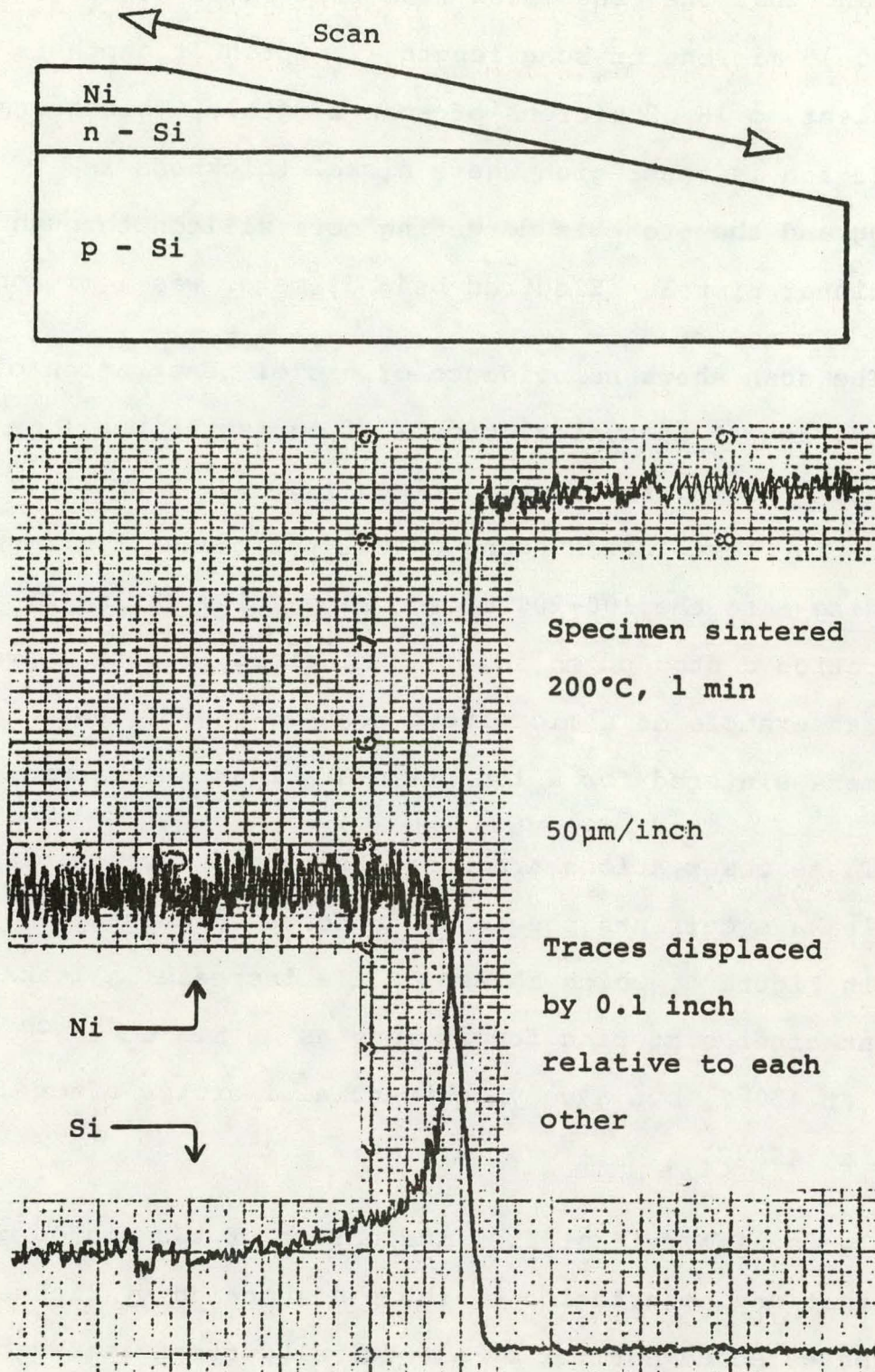
Figure 3. Electron Microprobe Analysis: Schematic of scan (above); data from a typical scan (below).
