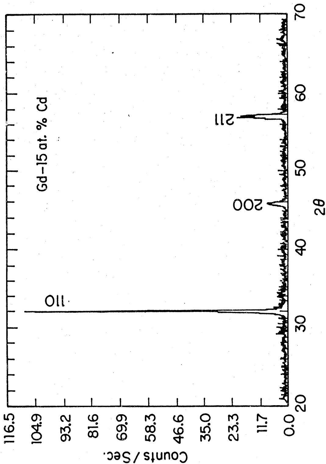
Fig. 2. X-ray diffraction pattern for quenched single phase bcc alloy Gd-15at.%Cd
