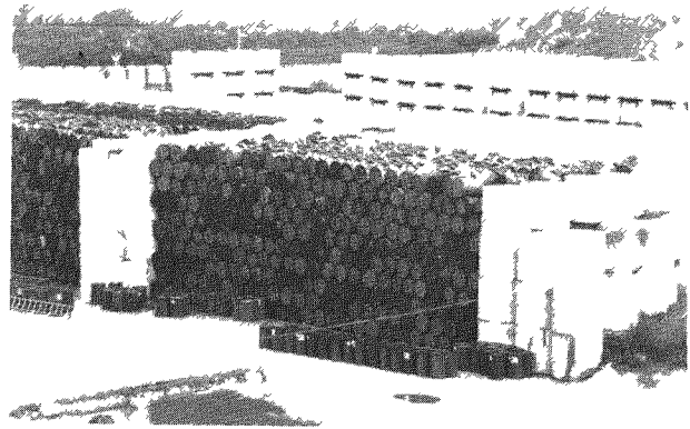
b. Metal drums containing low-level wastes which have been placed inside the "compartments" formed by rows of concrete blocks at the Centre de la Manche, France.
