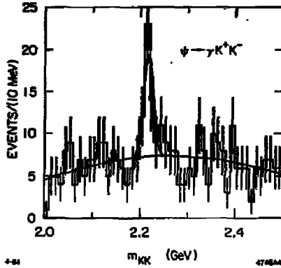
Fig. 4. Mass( K^+K^- ) (GeV) distribution from J/\psi \rightarrow \gamma K^+ K^- above 2 GeV. The curve represents a fit to a Breit-Wigner convoluted with a Gaussian plus a quadratic background.
