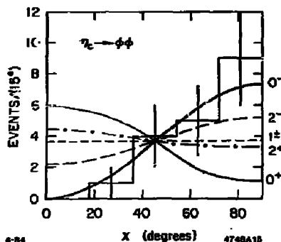
Fig. 9. Distribution of \chi , the angle between the \phi decay planes from \eta_c \rightarrow \phi\phi events. The curves represent the expectations from 0^- (thick solid), 0^+ (solid), 1^+ (short dashed), 2^+ (dashed dotted) and 2^- (long dashed).
