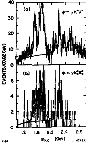
Fig. 2. Mass (KK) (GeV) distribution for (a) J/\psi \rightarrow \gamma K^+ K^- , and for (b) J/\psi \rightarrow \gamma K_S^0 K_S^0 . The curves represent fits to two incoherent Breit-Wigner curves plus a quadratic background.
