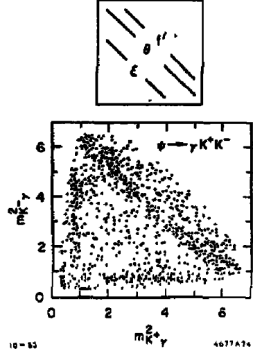
Fig. 3. Dalitz plot of mass (K+γ) 2 (GeV 2 ) versus mass (K-γ) 2 (GeV 2 ) from J/\psi \rightarrow \gamma K^+ K^- . The schematic drawing displays the bands of the f'(1515) , \theta and \xi decays.
