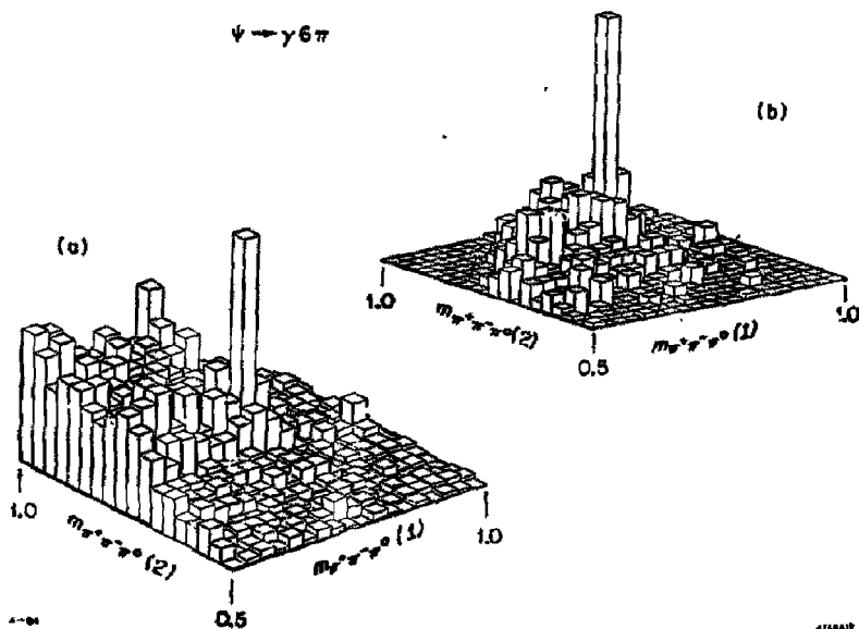
Fig. 16. Three dimensional histogram of m_{\pi^+\pi^-\pi^0}(1) versus m_{\pi^+\pi^-\pi^0}(2) in (GeV) from J/\psi \rightarrow \gamma\pi^+\pi^-\pi^0\pi^+\pi^- (four entries per event) for (a) all 6\pi -masses and (b) 1.6 \text{ GeV} \leq m_{6\pi} \leq 1.9 \text{ GeV} .
