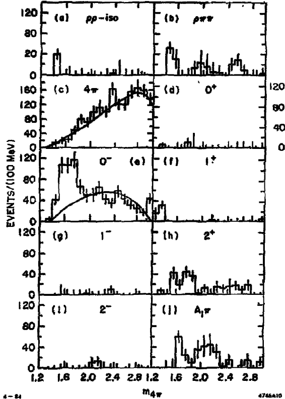
Fig. 13. Preliminary results of a 10-channel spin-parity analysis on J/\psi \rightarrow \gamma \pi^+ \pi^- \pi^+ \pi^- events. Plotted is m_{4\pi} (GeV) weighted with the fraction of the corresponding channel as determined by the fit. The curves drawn in (c) and (e) represent phase space for (c) J/\psi \rightarrow \gamma 4\pi , and (e) J/\psi \rightarrow \gamma \rho \rho , respectively.
