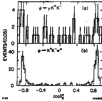
Fig. 6. Distributions of \cos \theta_{K^*}^* for (a) J/\psi \rightarrow \gamma K^+ K^- events at the mass of the \xi(2200) and (b) for background events from J/\psi \rightarrow K^+ K^- \pi^0 .
