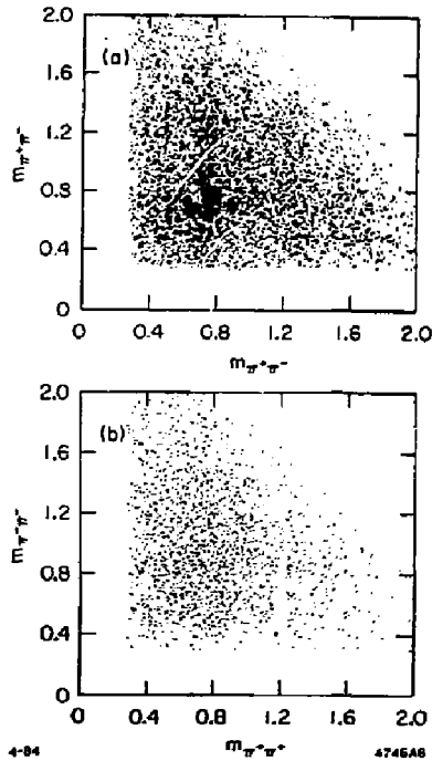
Fig. 11. Scatterplot of (a) m_{\pi^+\pi^-}(1) (GeV) versus m_{\pi^+\pi^-}(2) (GeV) with two entries per event and (b) m_{\pi^+\pi^+} (GeV) versus m_{\pi^-\pi^-} (GeV) providing evidence for \rho^0\rho^0 production in J/\psi \rightarrow \gamma\pi^+\pi^-\pi^+\pi^- .
