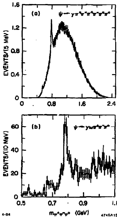
Fig. 15. Mass _{\pi^+\pi^-\pi^0} (GeV) distribution (a) for eight combinations per event from J/\psi \rightarrow \gamma\pi^+\pi^-\pi^0\pi^0\pi^0 and (b) for the recoiling \pi^+\pi^-\pi^0 combination after requiring 0.753 \text{ GeV} \leq m_{\pi^+\pi^-\pi^0} \leq 0.813 \text{ GeV} for one combination in (a).
