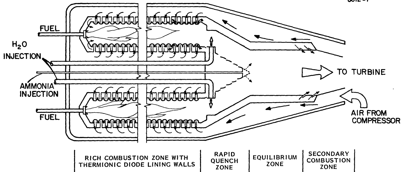
Figure 9. TAM Combustor Design Concept
