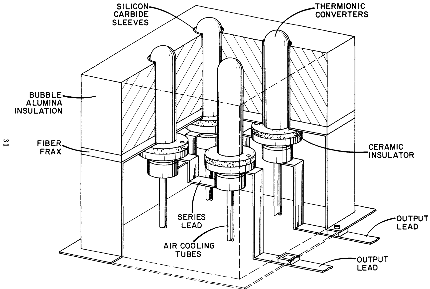
Figure 11. Four-Converter Array
