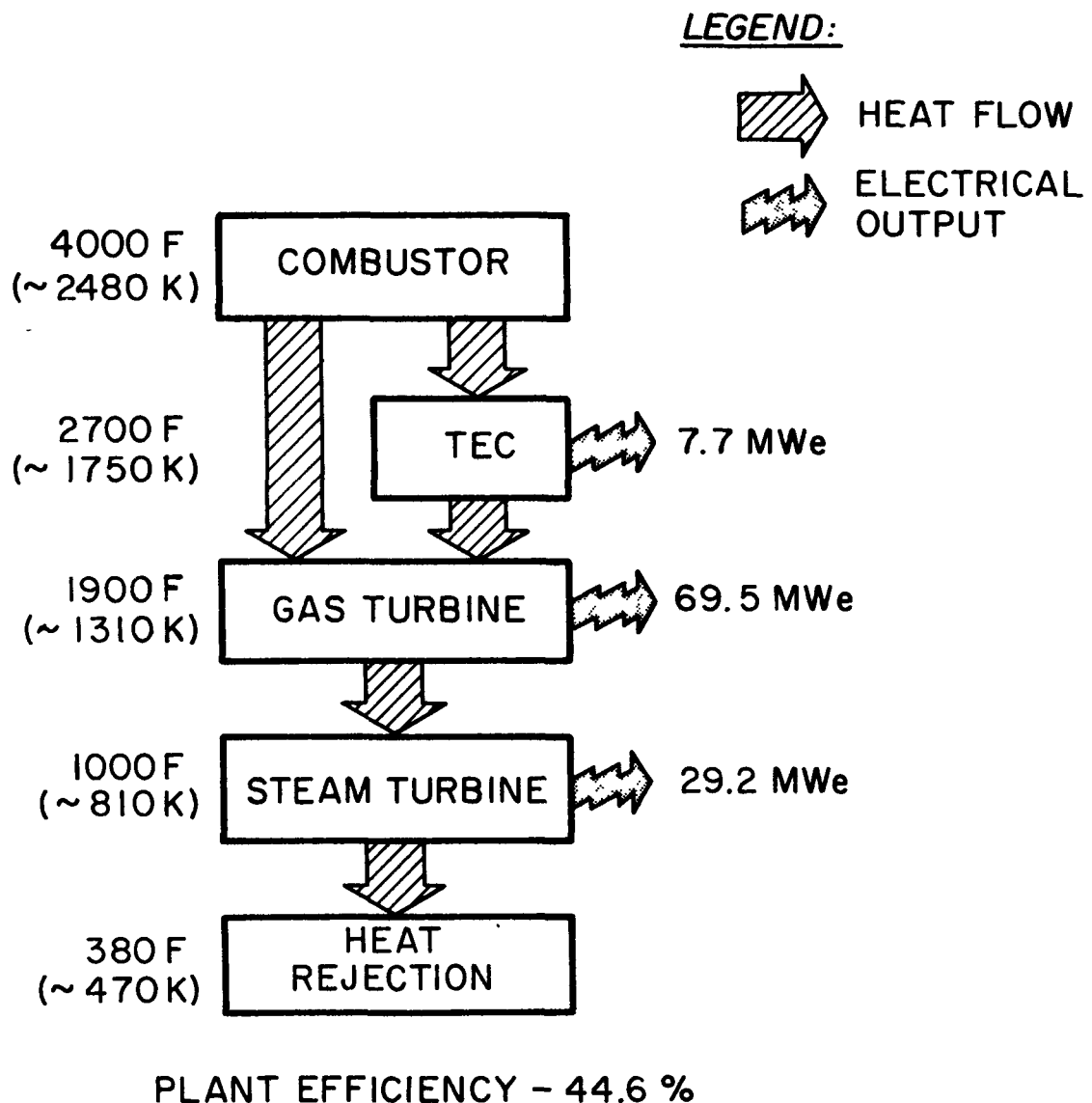
Figure 8. Block Diagram of TAM Combustor Combined Cycle System
