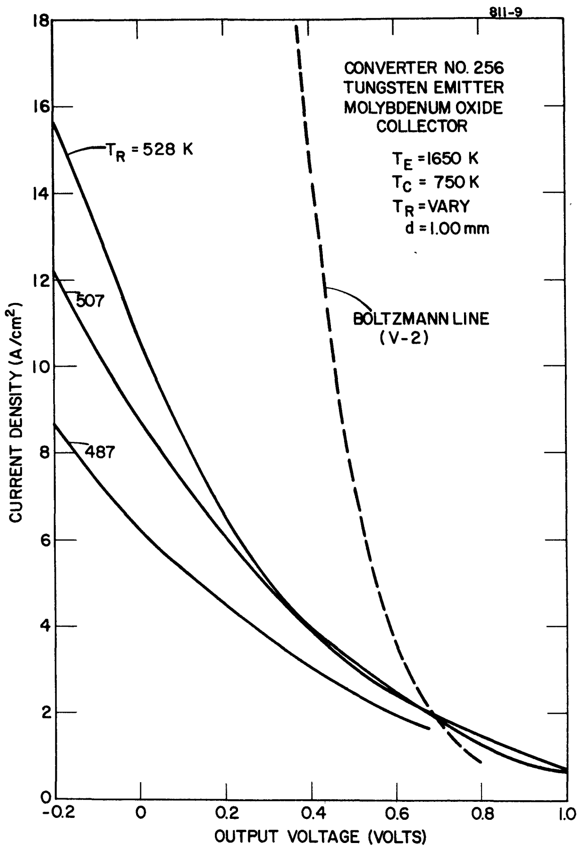
Figure 19. Cesium Reservoir Temperature Family for Converter No. 256 ( T_E = 1650 \text{ K} , T_C = 750 \text{ K} , and d = 1.00 \text{ mm} )
