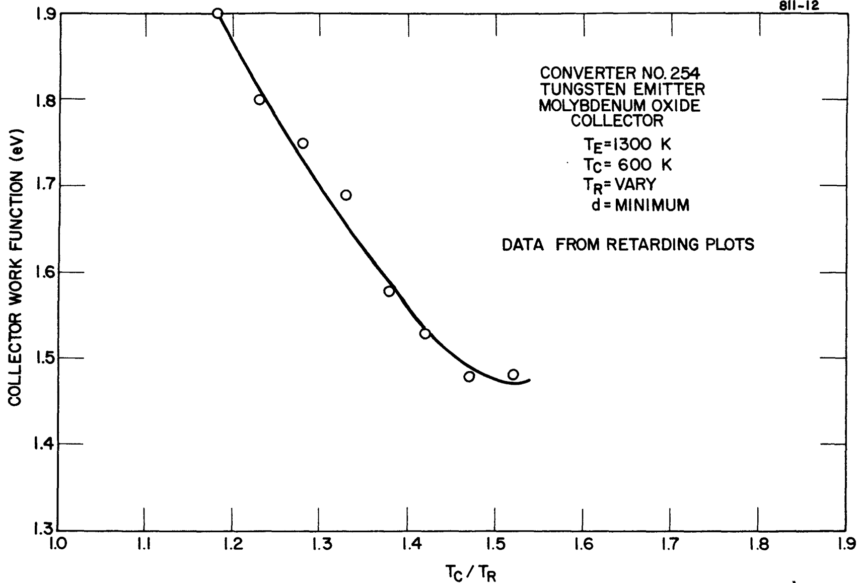
Figure 18. Collector Work Function Versus T_C/T_R for Converter No. 254
