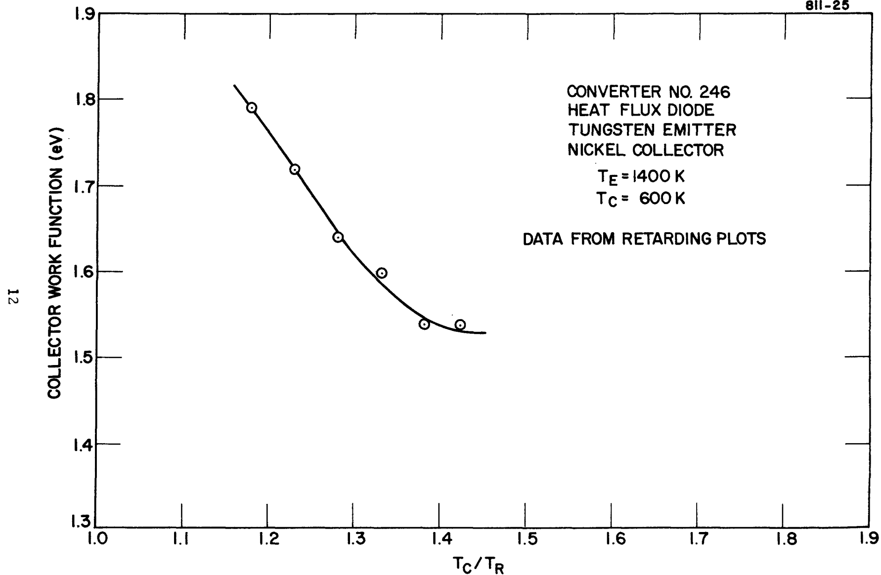
Figure 6. Collector Work Function Versus T_C/T_R for Converter No. 246
