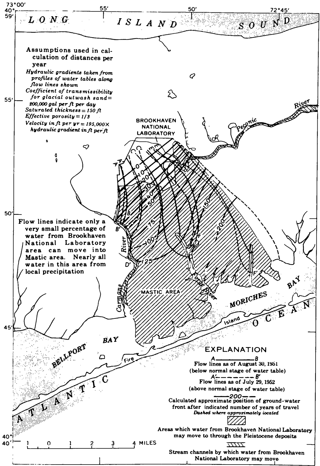
Figure 11. Direction and Time of Travel of Ground Water Laterally in Upper Pleistocene Deposits from the Brookhaven National Laboratory Area to Points of Discharge
