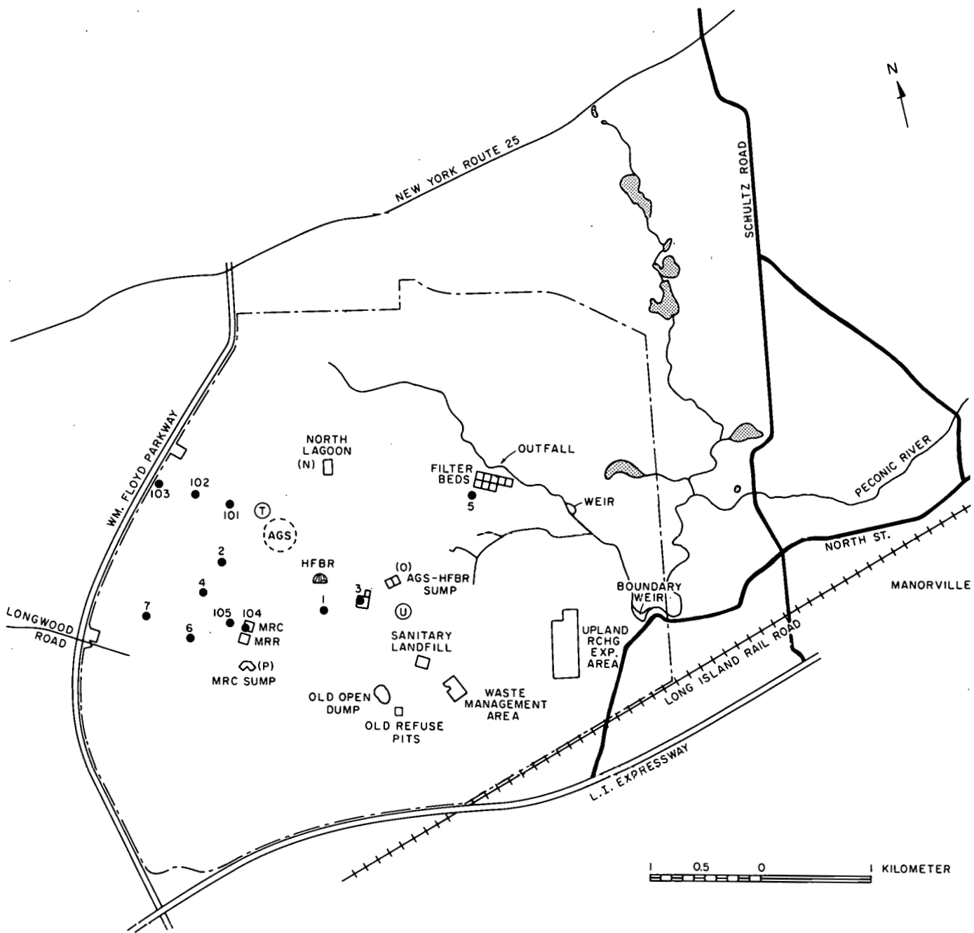
Figure 8. On-site Potable and Supply Wells
