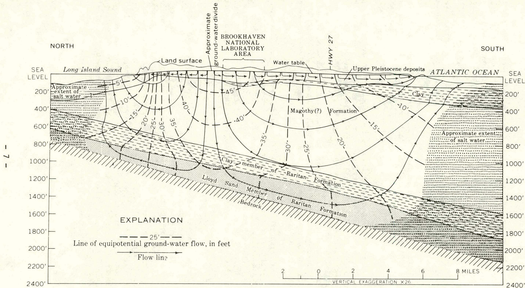
Figure 4. Schematic Ground-Water Flow Lines, Central Upton Area
