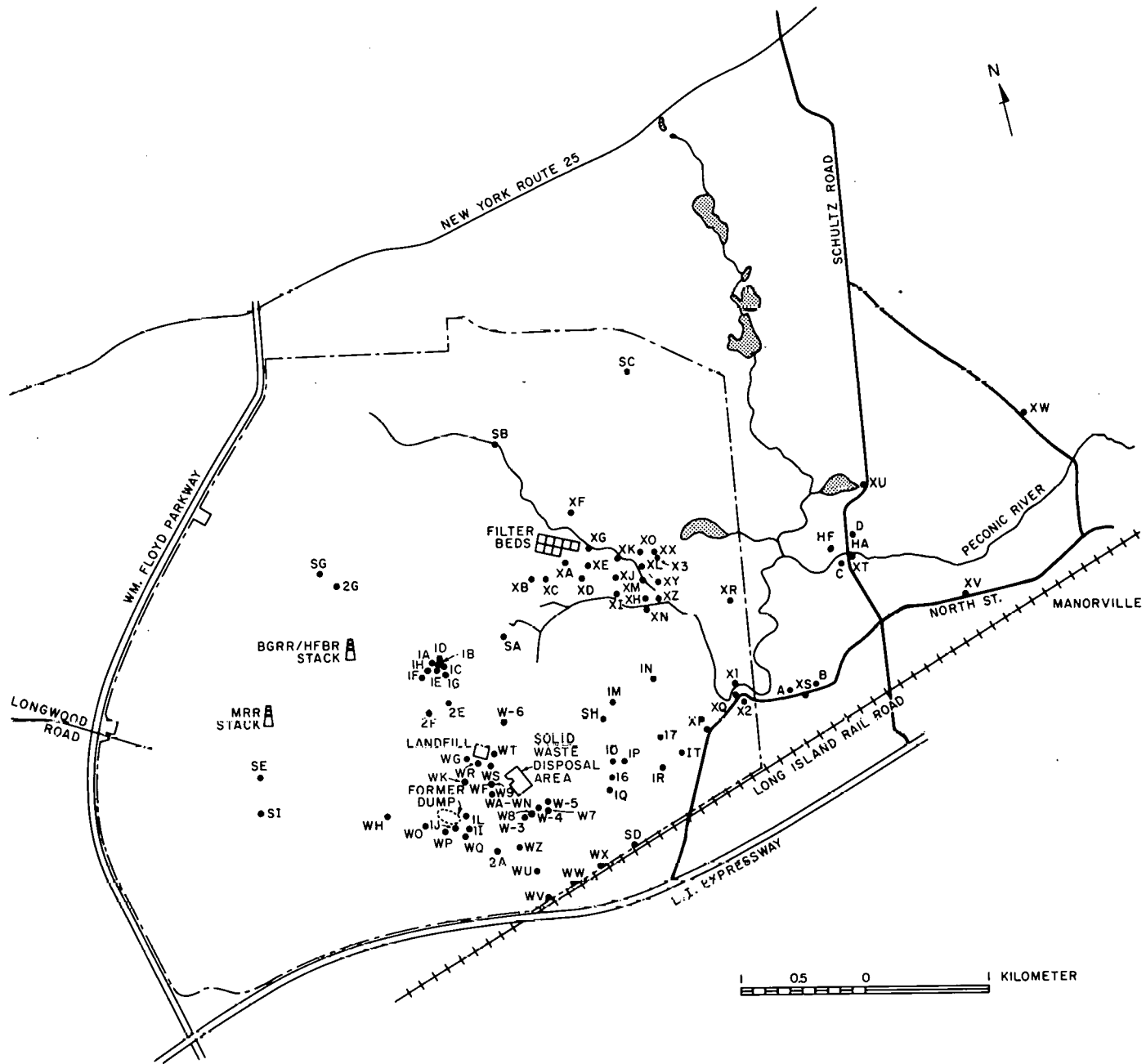
Figure 9. Location of Groundwater Surveillance Wells
