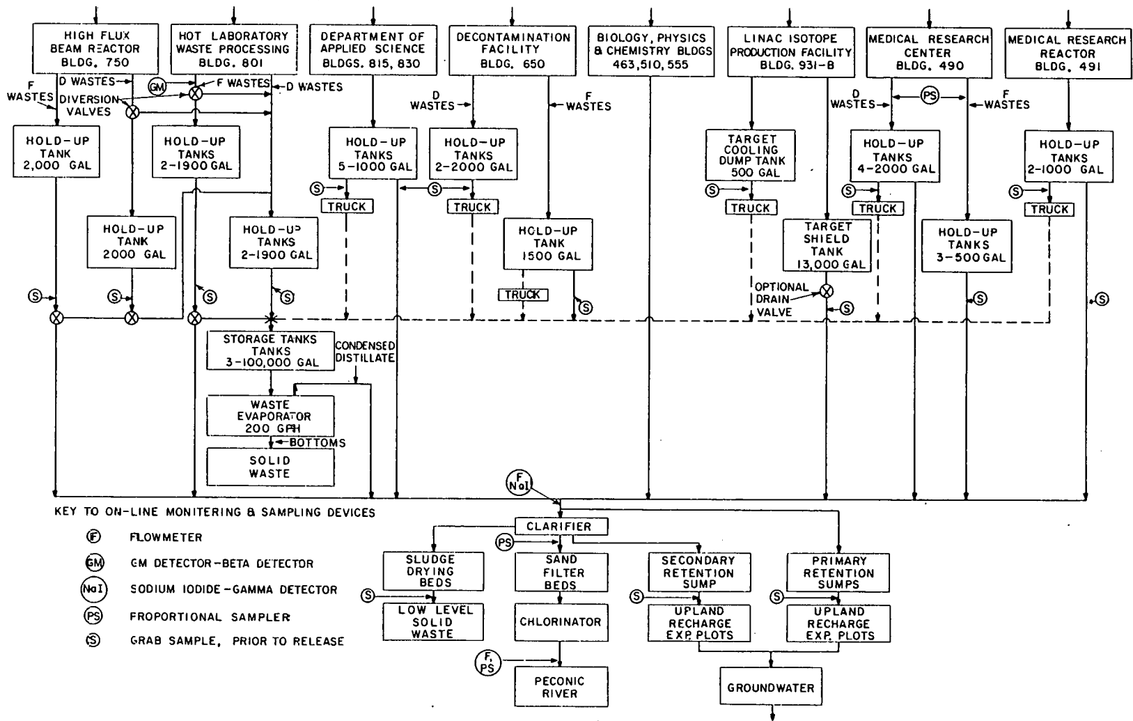
Figure 5. BNL Liquid Effluent Systems
