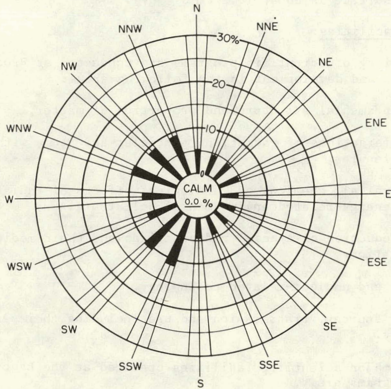
Figure 3. Annual Wind Rose. The Wind Rose also Represents the Period 1973-1979
