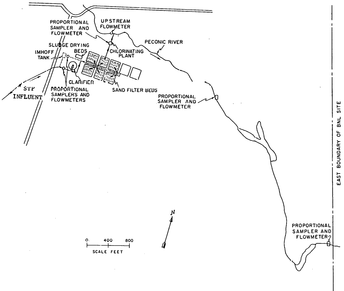
Figure 6. Sewage Treatment Plant
