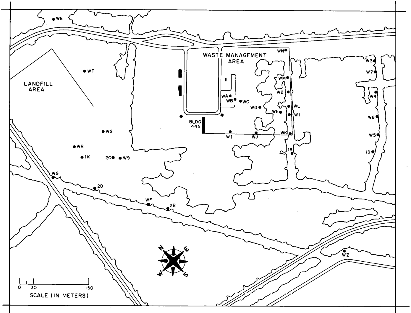
Figure 10. Landfill and Waste Management Area Surveillance Wells
