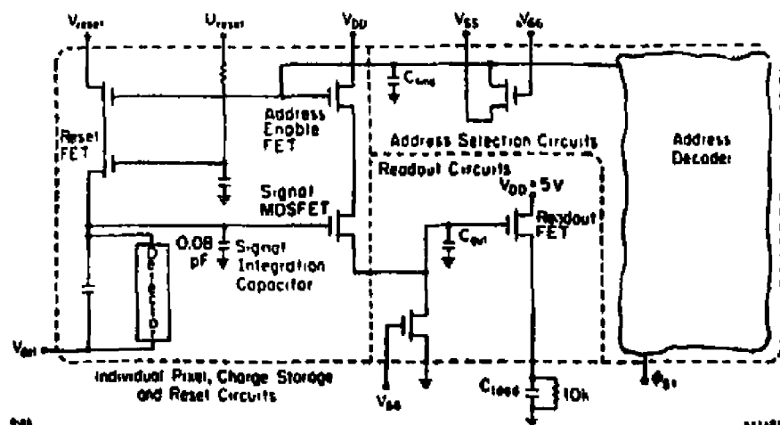
Fig. 2: Schematic drawing of the readout electronics of the 10 x 64 readout array.
