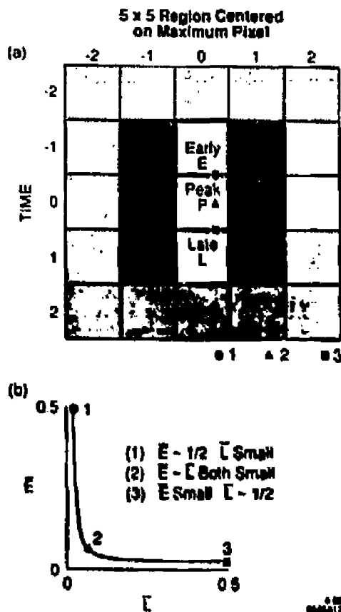
Fig. 6: (a) A schematic of a 5 \times 5 pixel region centered on a particle hit; and (b) a schematic plot of the E versus L planes indicating the result of various hypothetical incident positions of a particle within the central pixel.
