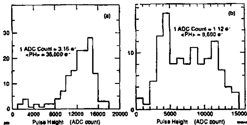
Fig. 5: (a) The pulse height spectrum of the alpha data; and (b) the pulse height spectrum of the beta data.
