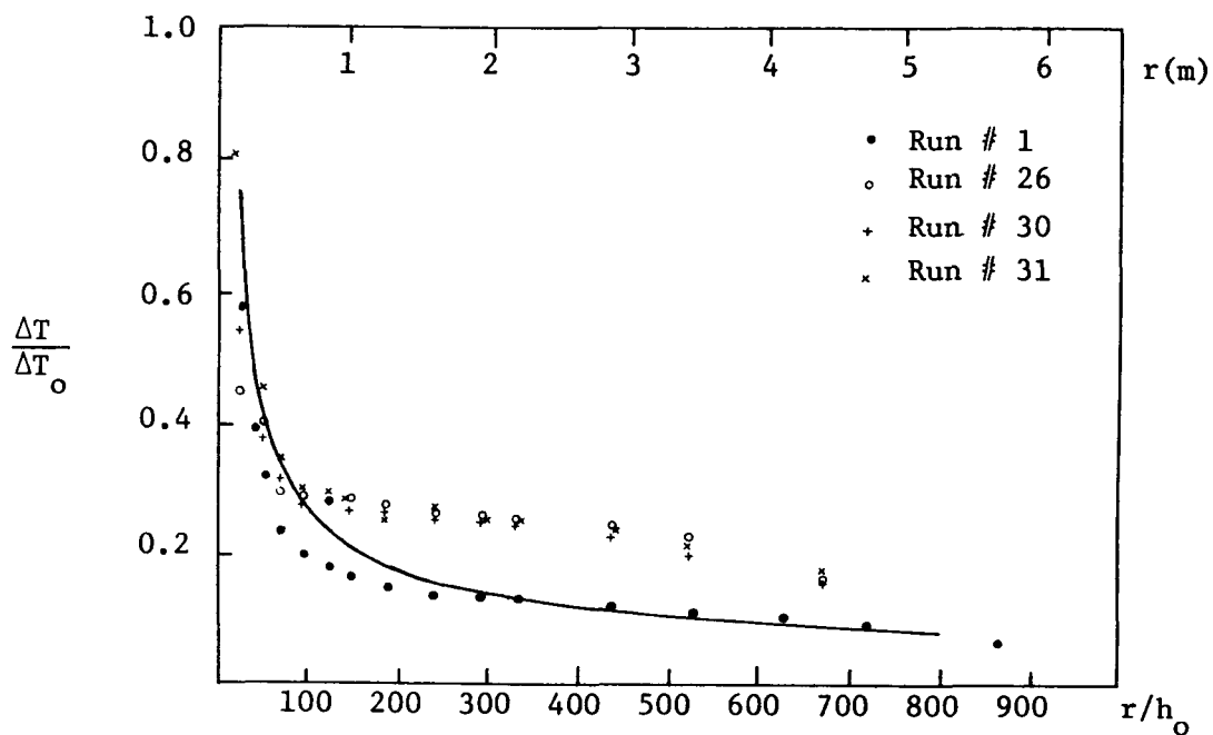
Figure 7.10a Temperature vs. Distance, Experimental Comparison to Model
