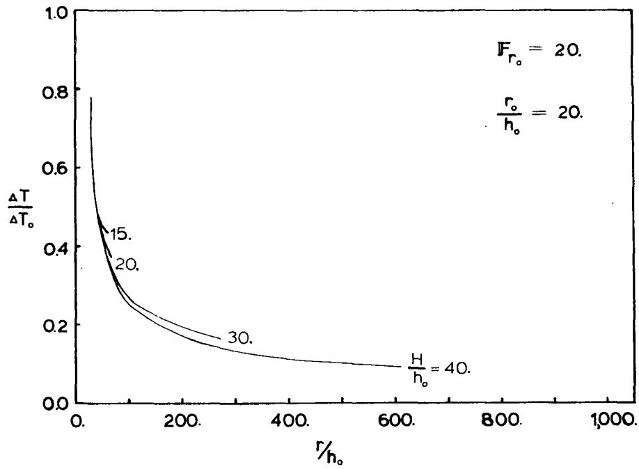
Figure 7.4a Temperature vs. Distance, Varying H/h_0 .
