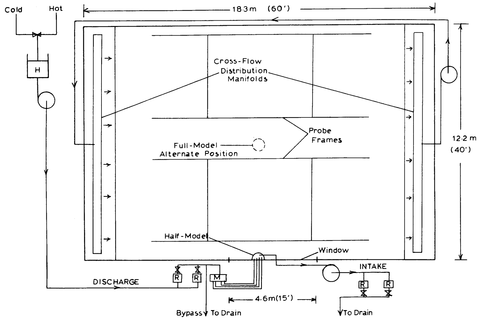
Figure 3.3 Schematic Diagram of the Experimental Setup.
