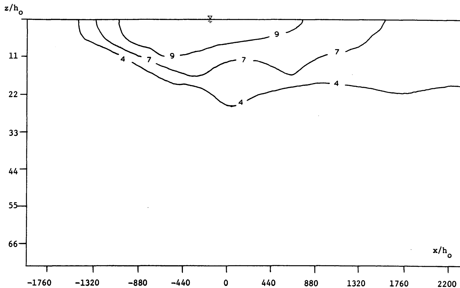
Figure A.3.17 Longitudinal Transect A-A at y = 2.25\text{m} , Run #22.
