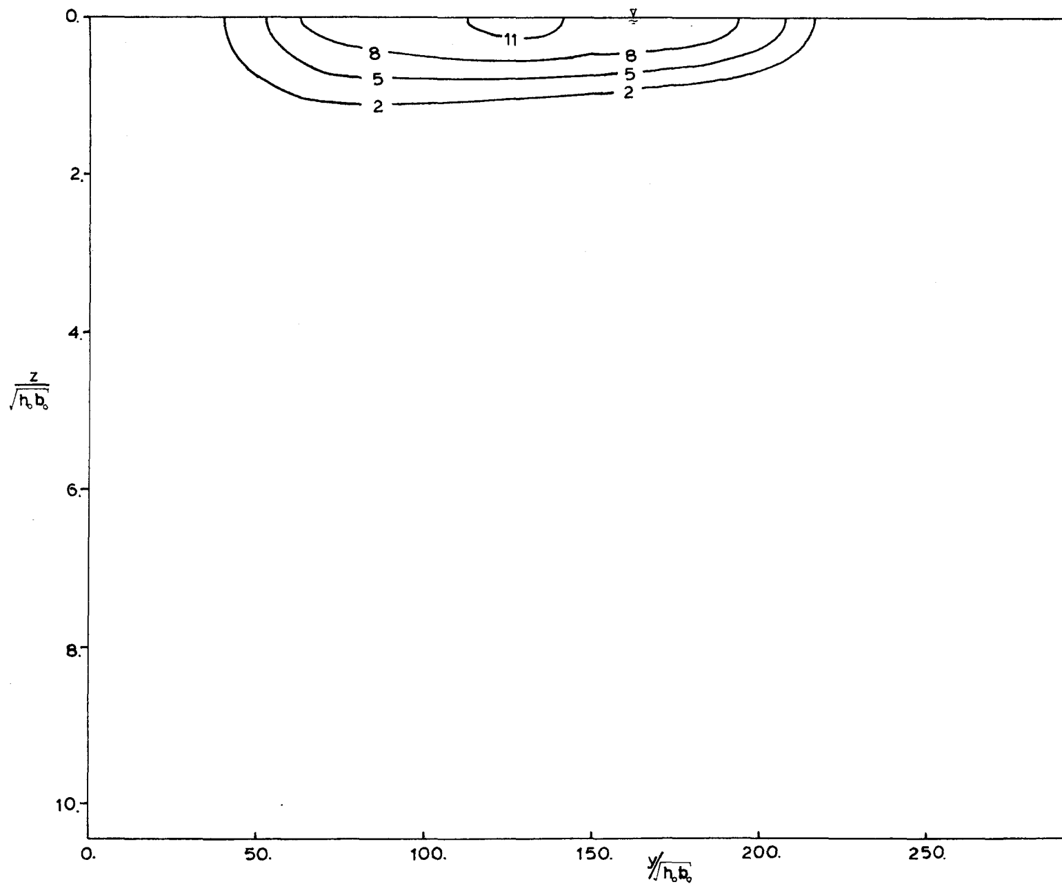
Figure A.3.12 Lateral Transect B-B at x = -5.5\text{m} , Run #20.
