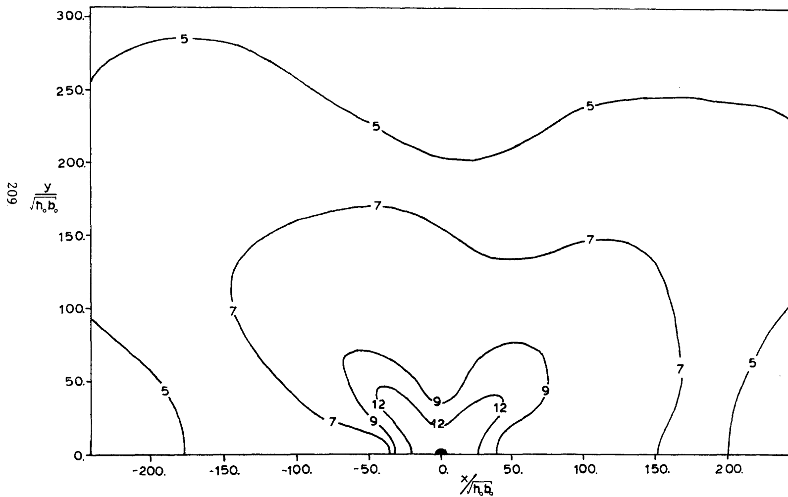
Figure A.2.10 Plan View. Run #13.
