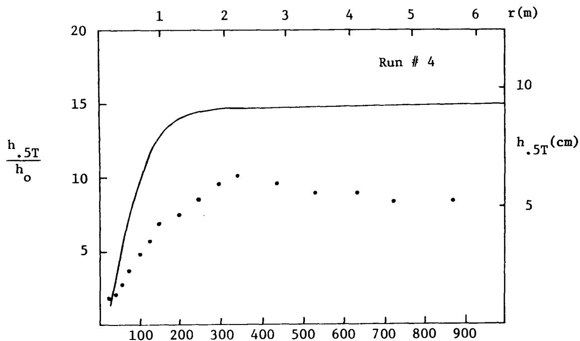
Figure 7.13b Half-Temperature Depth vs. Distance, Experimental Comparison to Model
