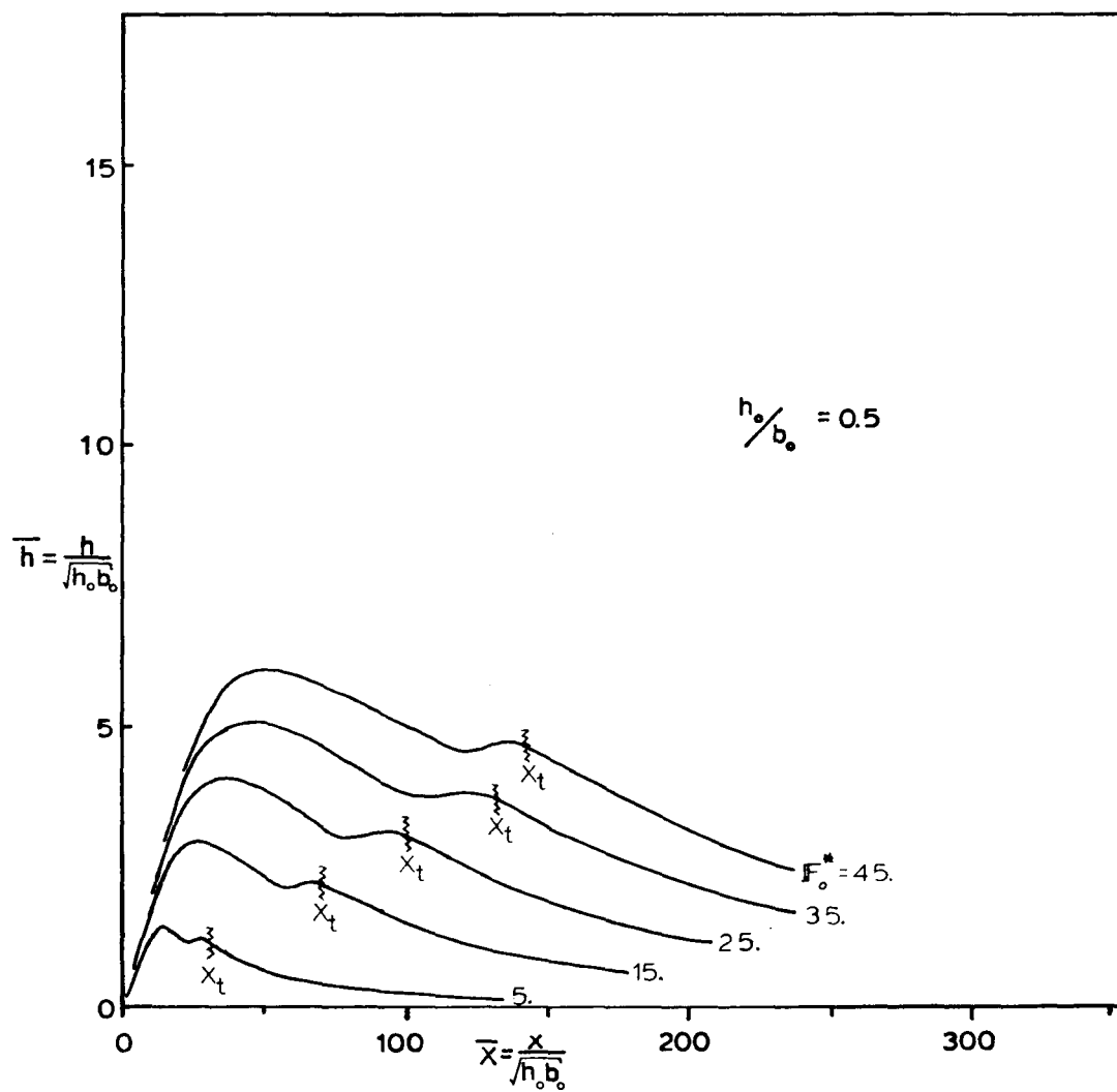
Figure 8.6 Interface Jet Depth vs. Distance, Varying F_o^*
