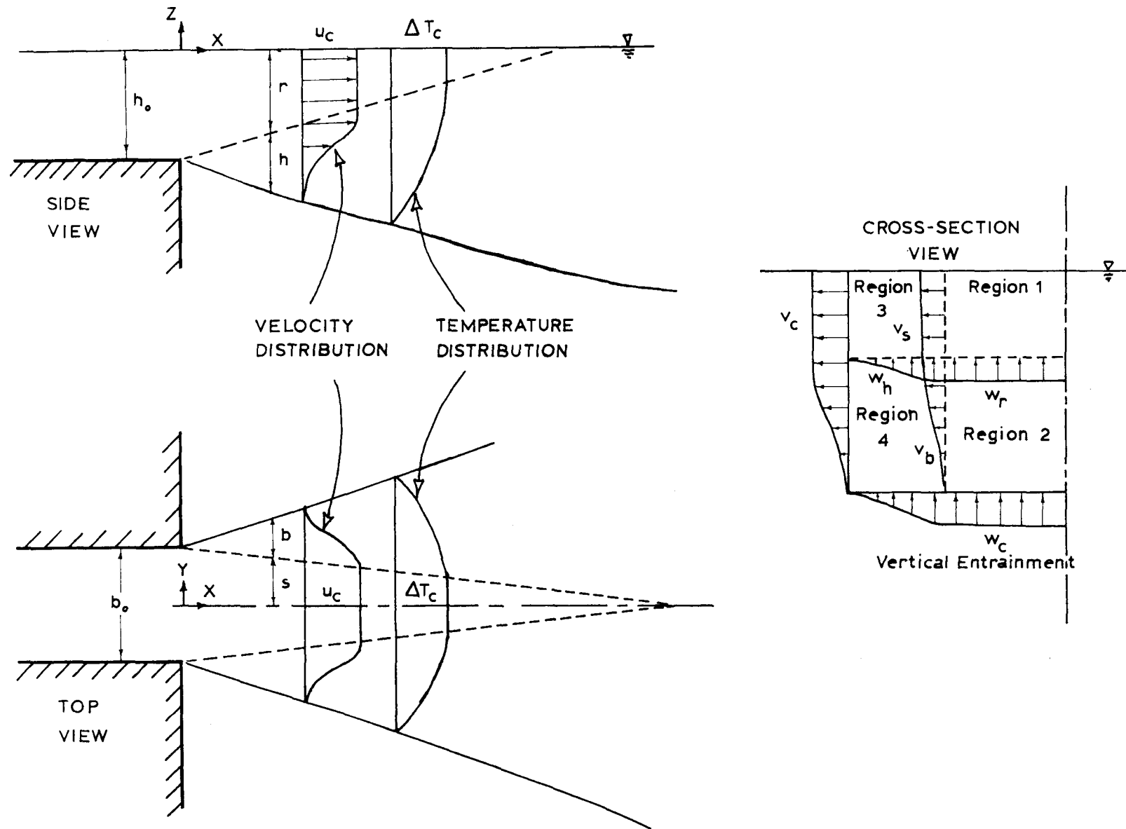
Figure 8.2 Detailed Jet Structure in Zone of Flow Establishment
