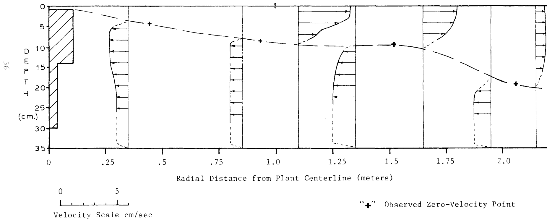
Figure 4.6 Mean Velocity Measurement Example [Exp #51]
