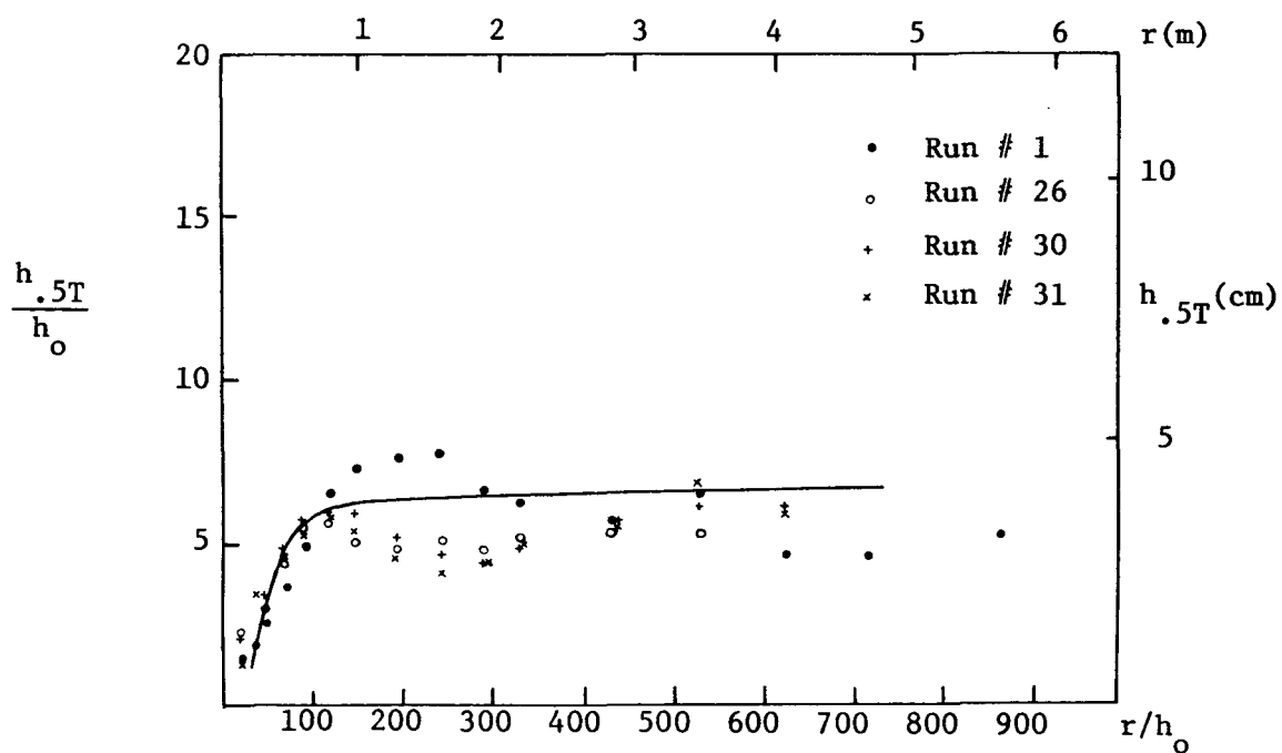
Figure 7.10b Half-Temperature Depth vs. Distance, Experimental Comparison to Model
