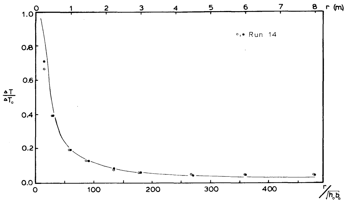
Figure 8.14 a Temperature vs. Distance, Experimental Comparison to Model
