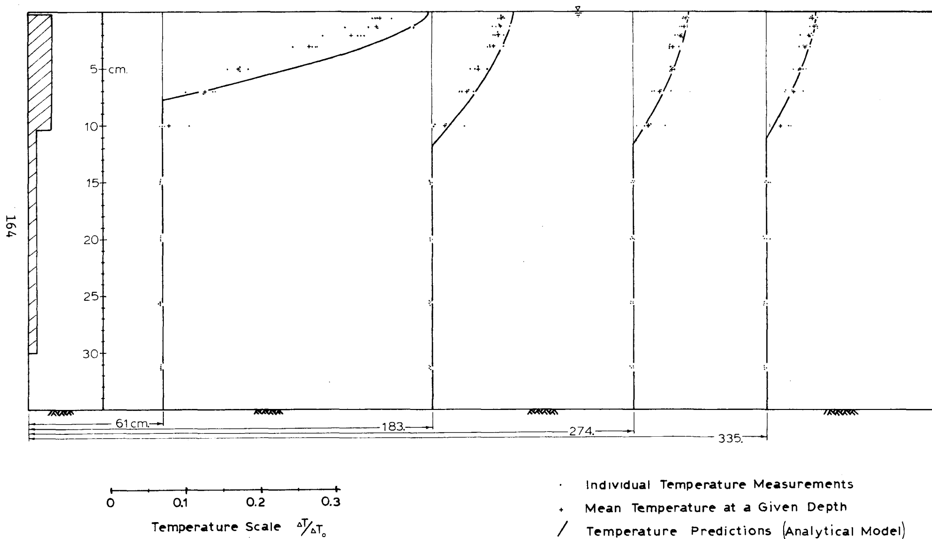
Figure 8.13 Temperature Profile Comparison Between Analytical Model and Data (Experiment # 37; Stagnant, Separate Jet Discharge).
