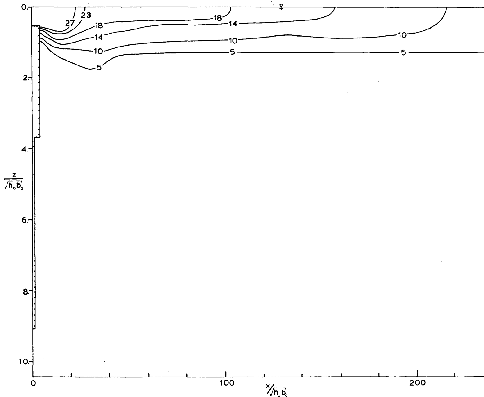
Figure A.2.3 Centerline Section Jet #2. Run #10.
