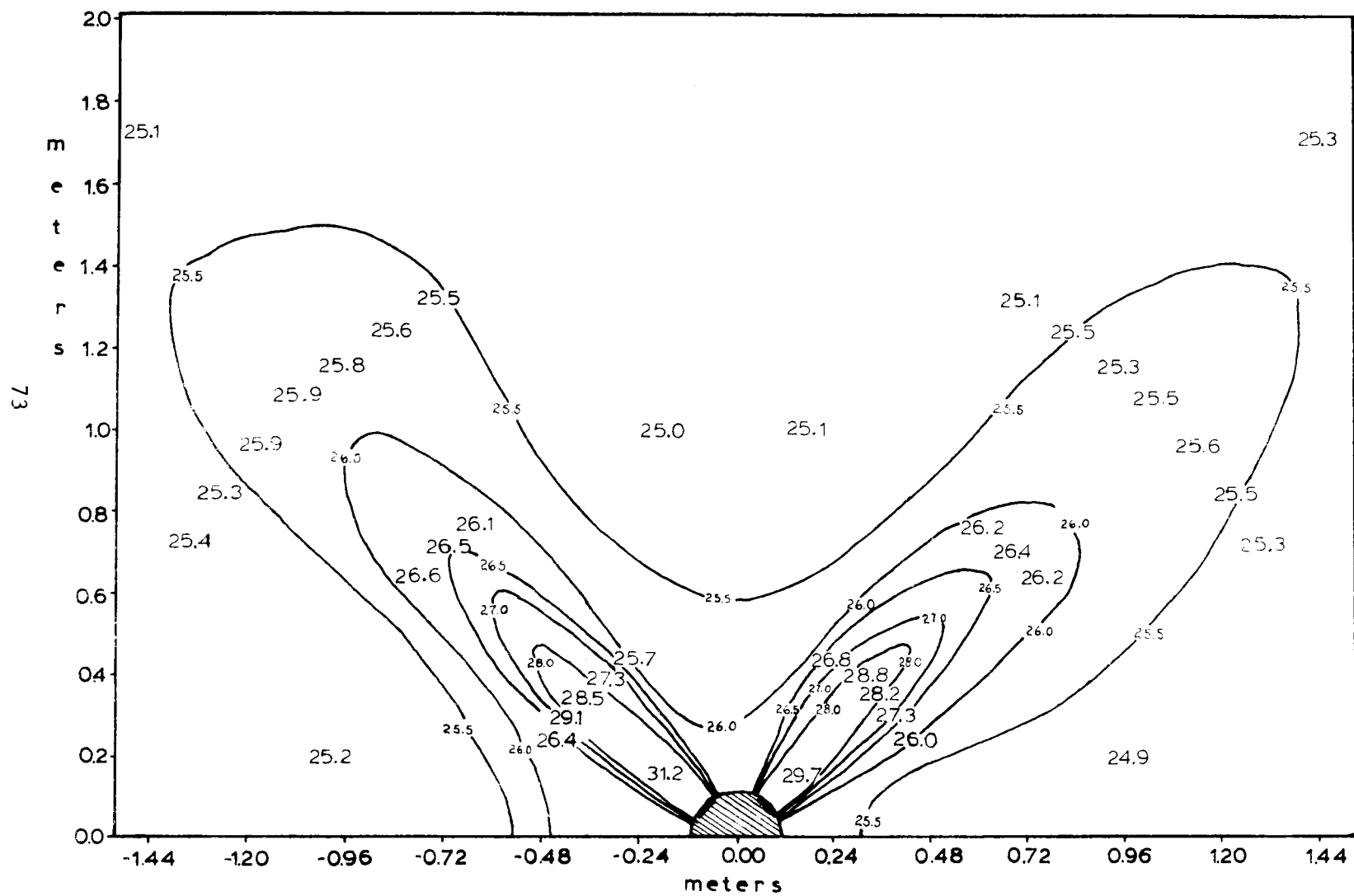
Figure 5.4 Typical Plan View of Surface Isotherms, Stagnant Experiment with Separate Jet Discharge (Exp. #11)
