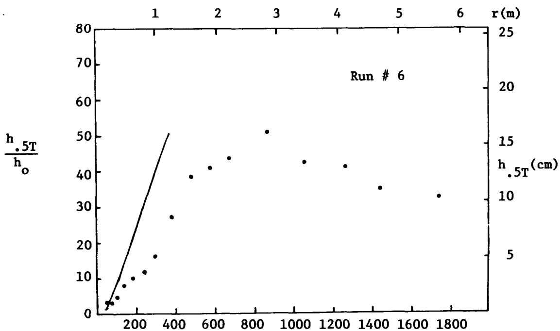
Figure 7.18b Half-Temperature Depth vs. Distance, Experimental Comparison to Model
