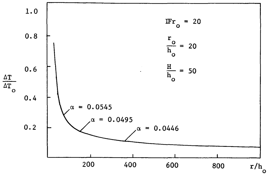
Figure 7.5a Temperature vs. Distance, Varying \alpha
