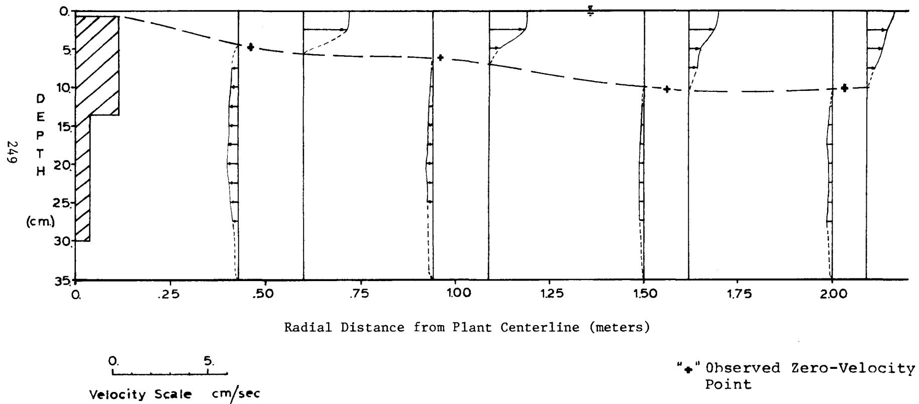
Figure B.1 Photographic Velocity Measurements Exp #60
