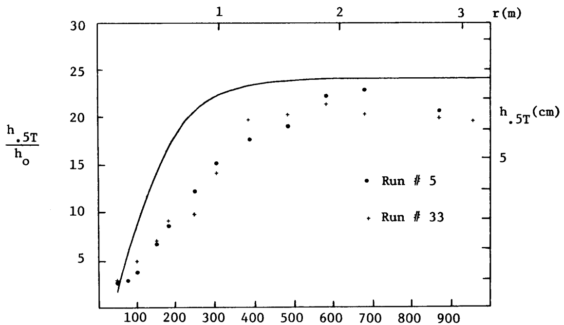
Figure 7.14b Half-Temperature Depth vs. Distance, Experimental Comparison to Model
