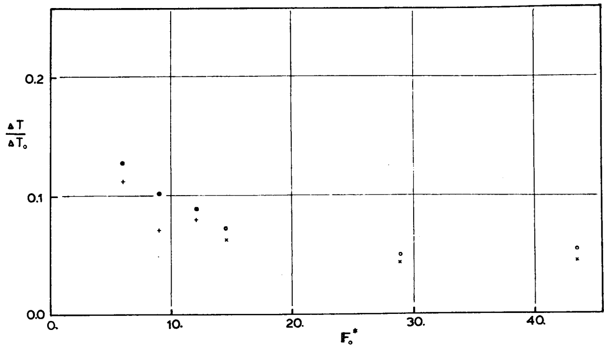
Figure 5.9a Comparison of Jet Centerline and Lateral Return Flow Surface Temperature Data at X = 4.0m .
