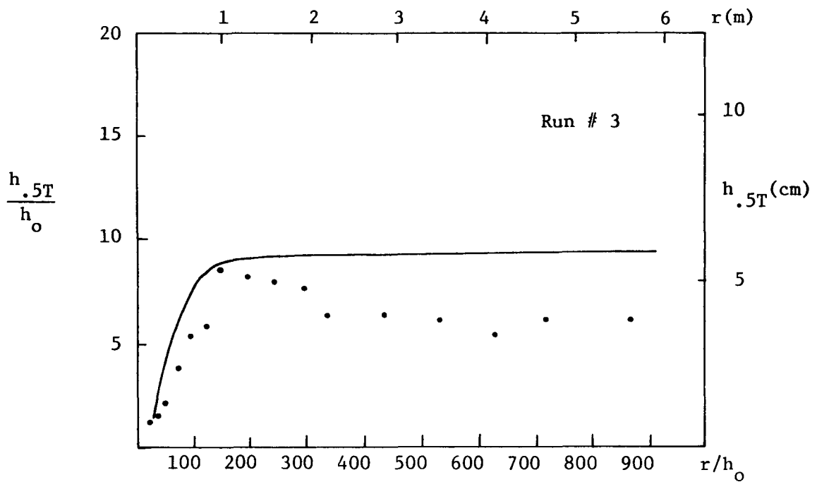
Figure 7.12b Half-Temperature Depth vs. Distance, Experimental Comparison to Model
