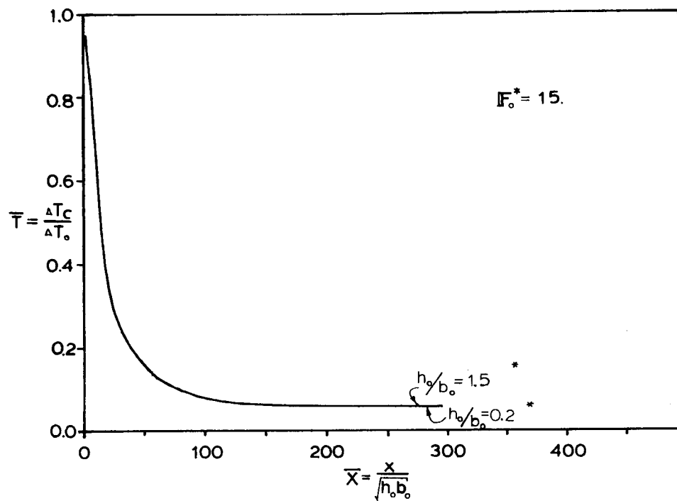
Figure 8.5a Centerline Temperature vs. Distance Varying h_o/b_o
