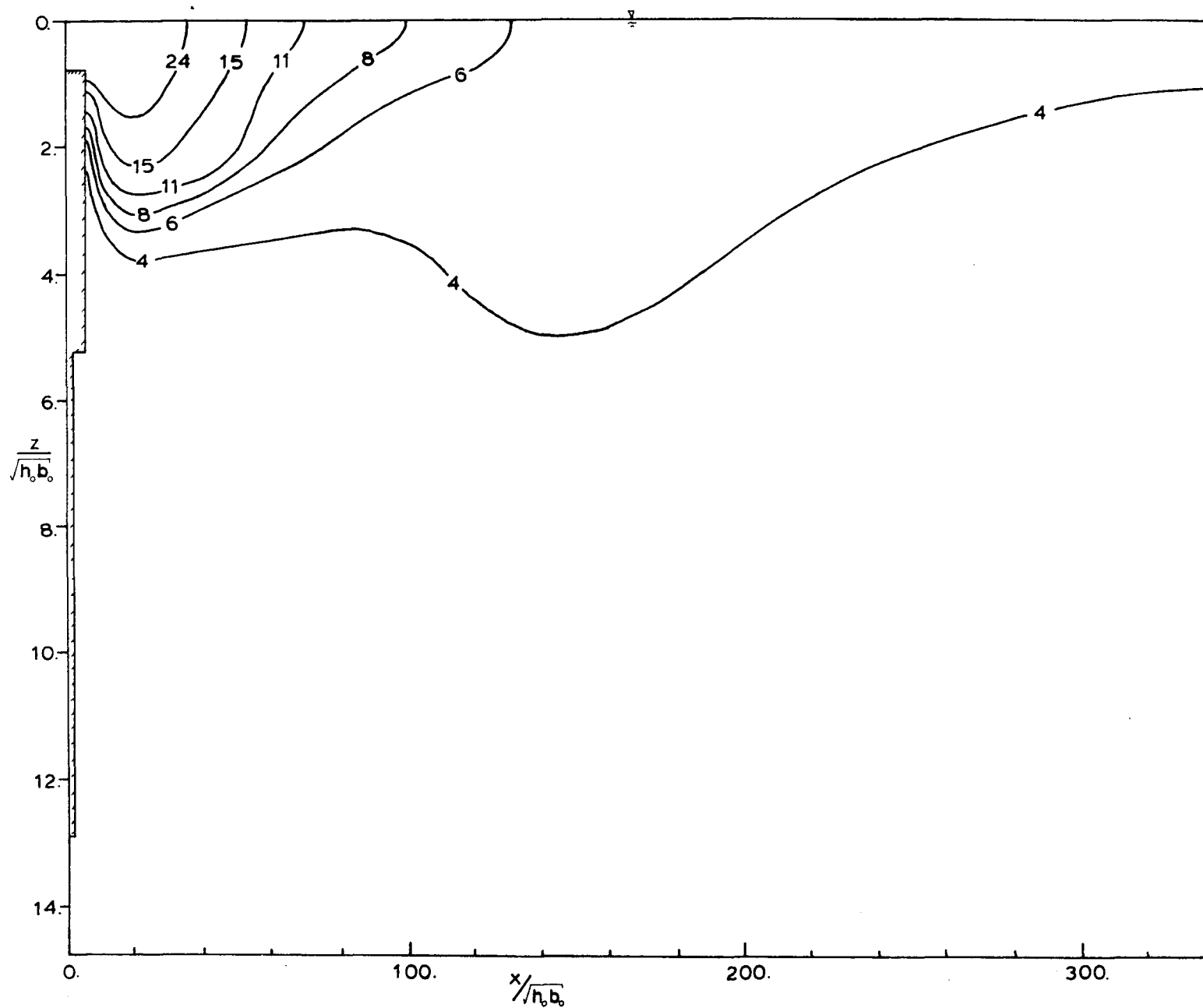
Figure A.2.14 Centerline Section of Jet #1. Run #14.
