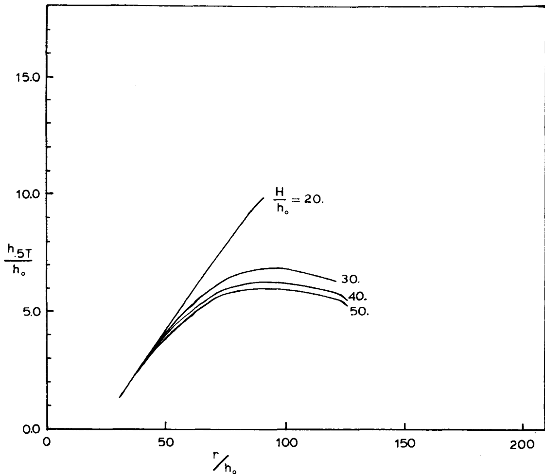
Figure 7.8 Half Temperature Depth vs. Distance, Varying H/h_o ; Radial Interface Jet.
