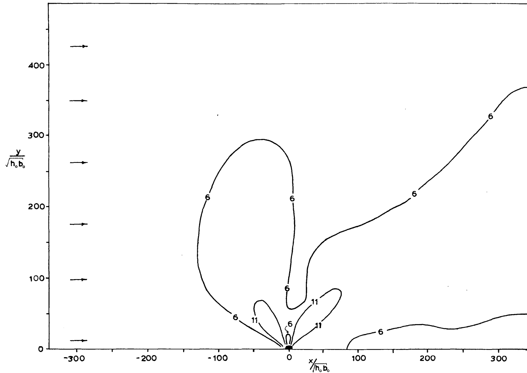
Figure A.3.1 Plan View of Run #17, Separate Jet Discharge.
