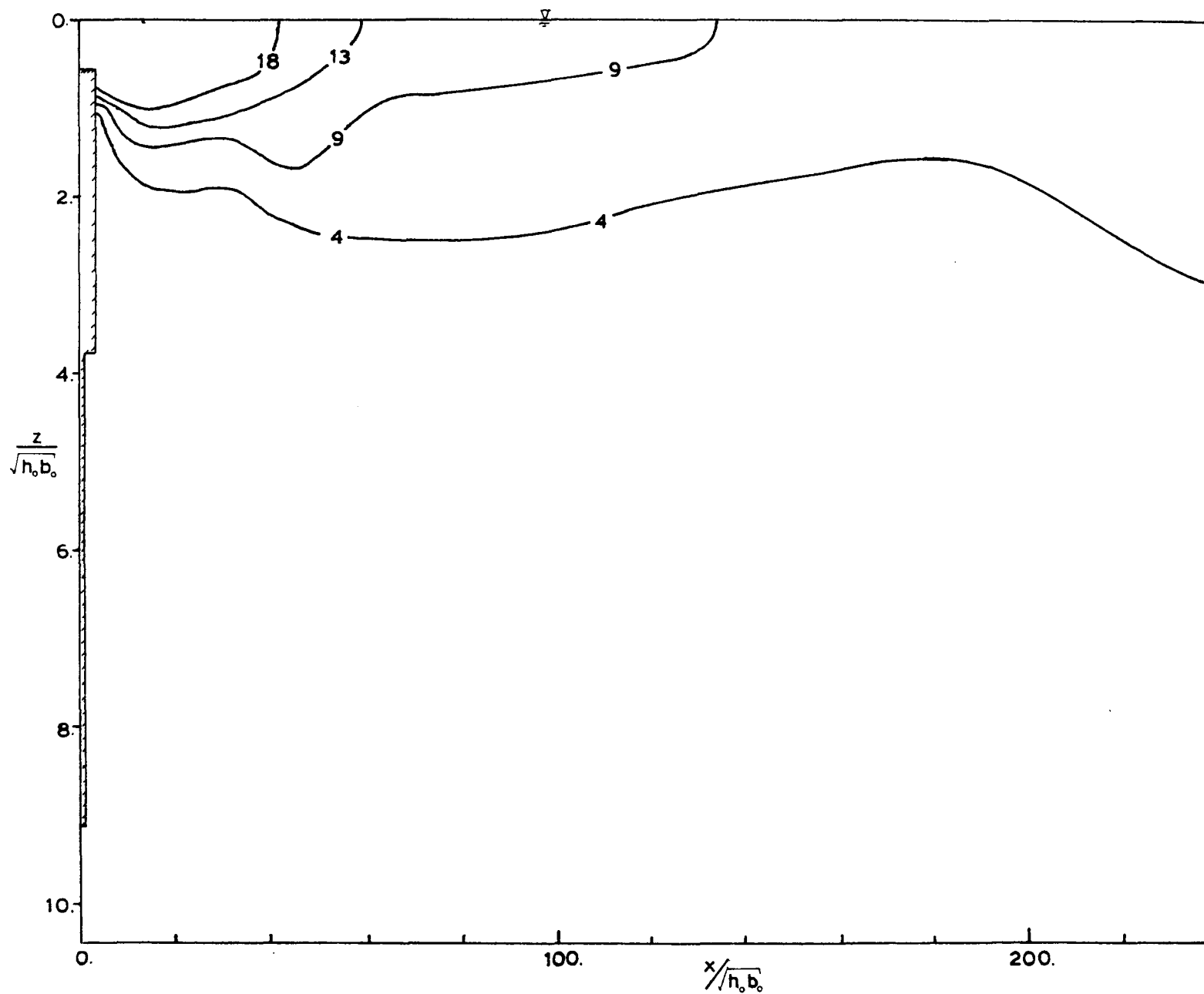
Figure A.2.6 Centerline Section of Jet #2. Run #11.
