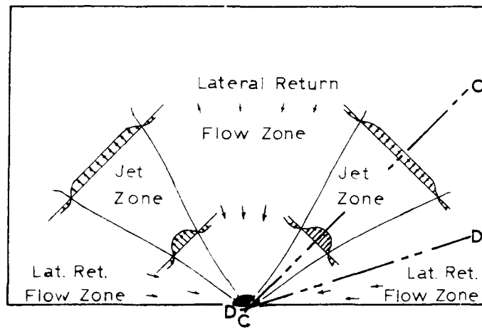
Figure 5.1 Flow Zones for Separate Jet Configuration
