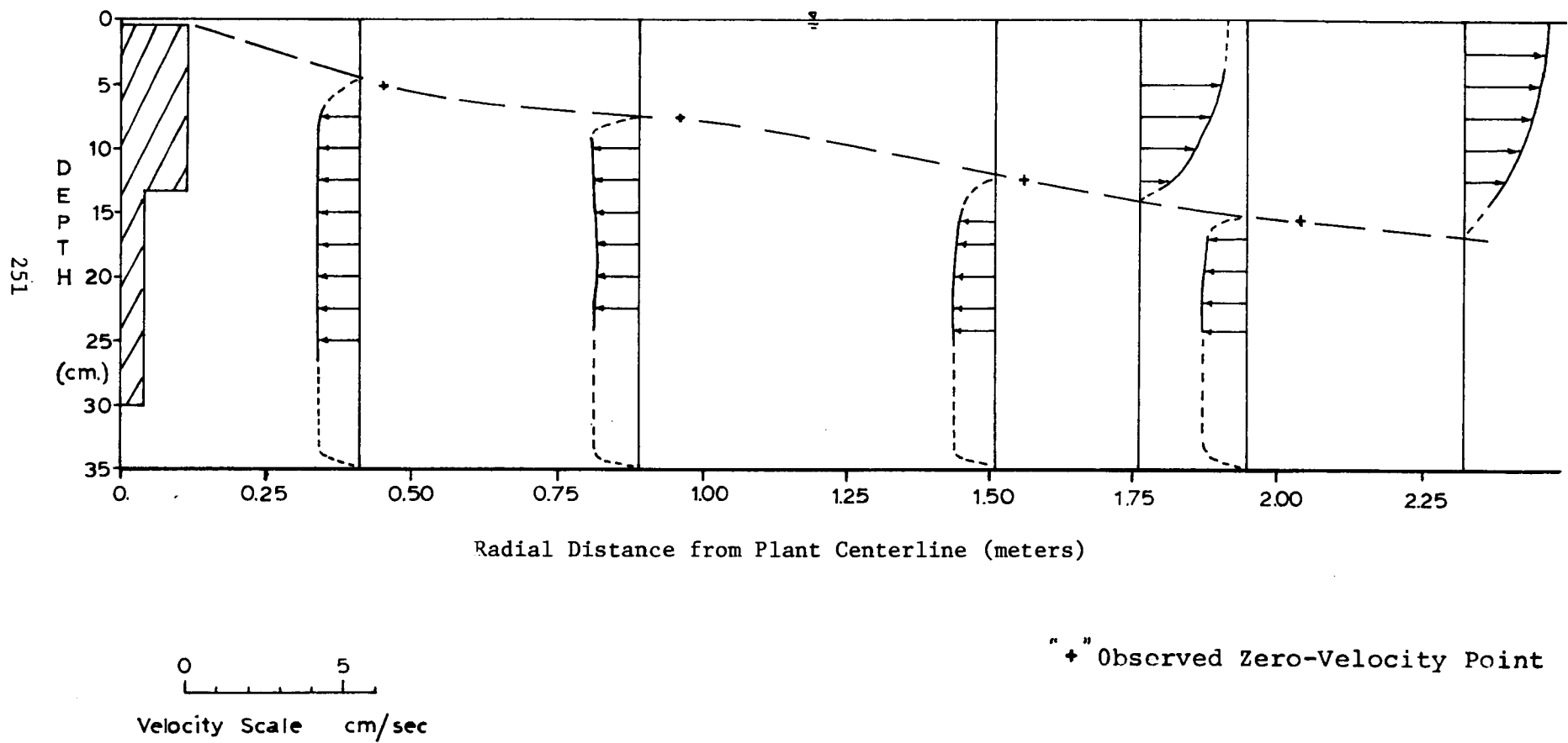
Figure B.3 Photographic Velocity Measurements, Exp #56
