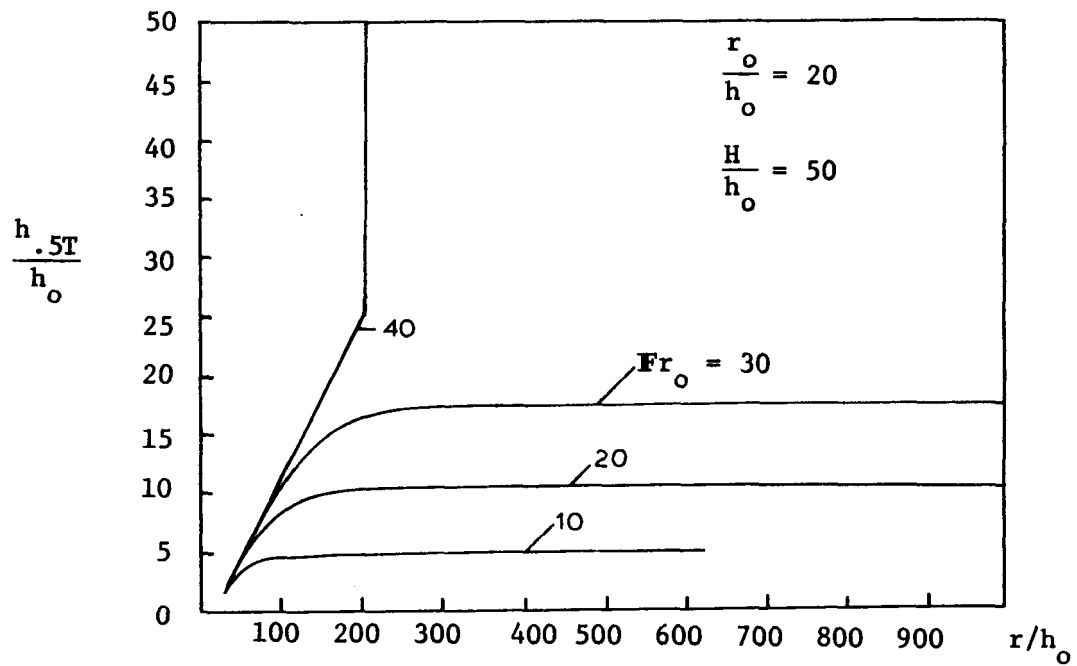
Figure 7.2b Half-Temperature Depth vs. Distance, Varying Fr_o
