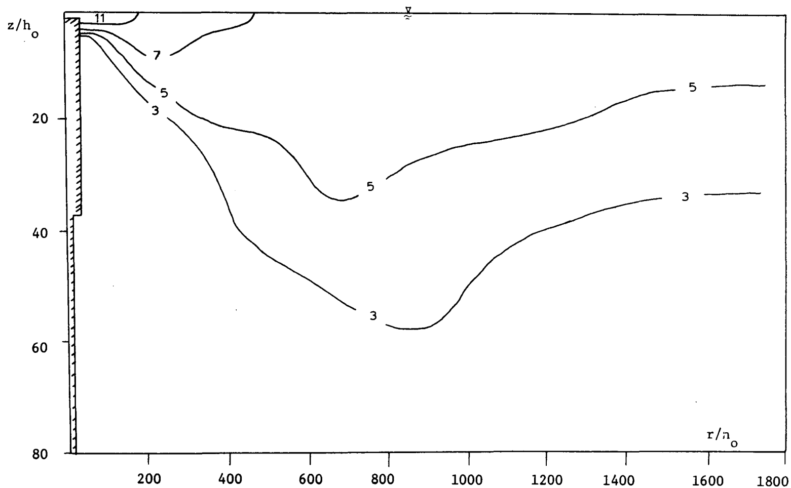
Figure A.1.6 Radially Averaged Cross-Section. Run # 6
