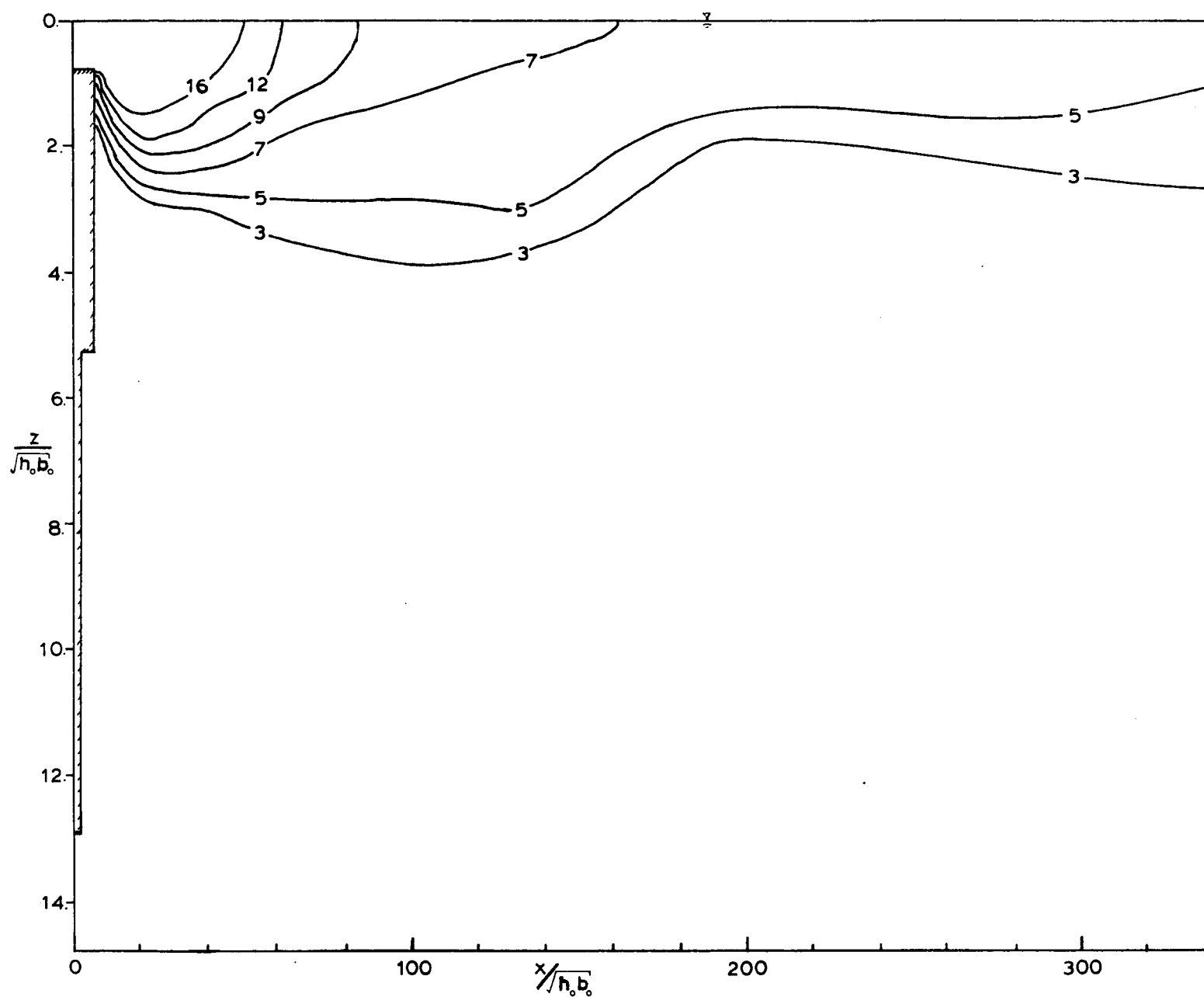
Figure A.2.12 Centerline Section of Jet #2. Run #13.
