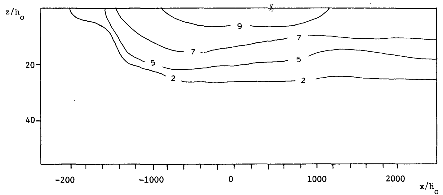
Figure A.3.29 Longitudinal Transect A-A at y = 2.25 m, Run #34.
