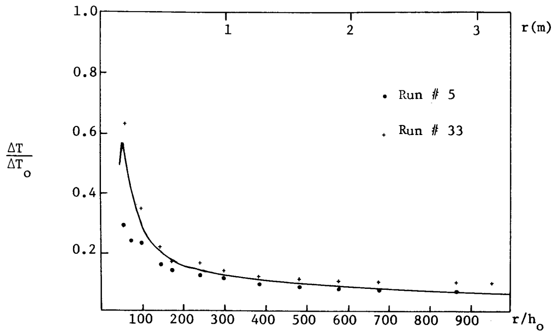
Figure 7.14a Temperature vs. Distance, Experimental Comparison to Model
