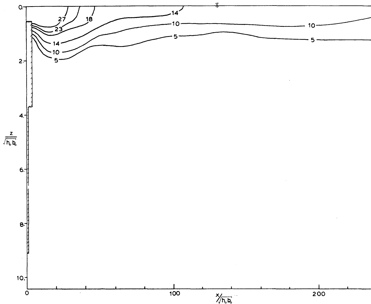
Figure A.2.2 Centerline Section Jet #1. Run #10.
