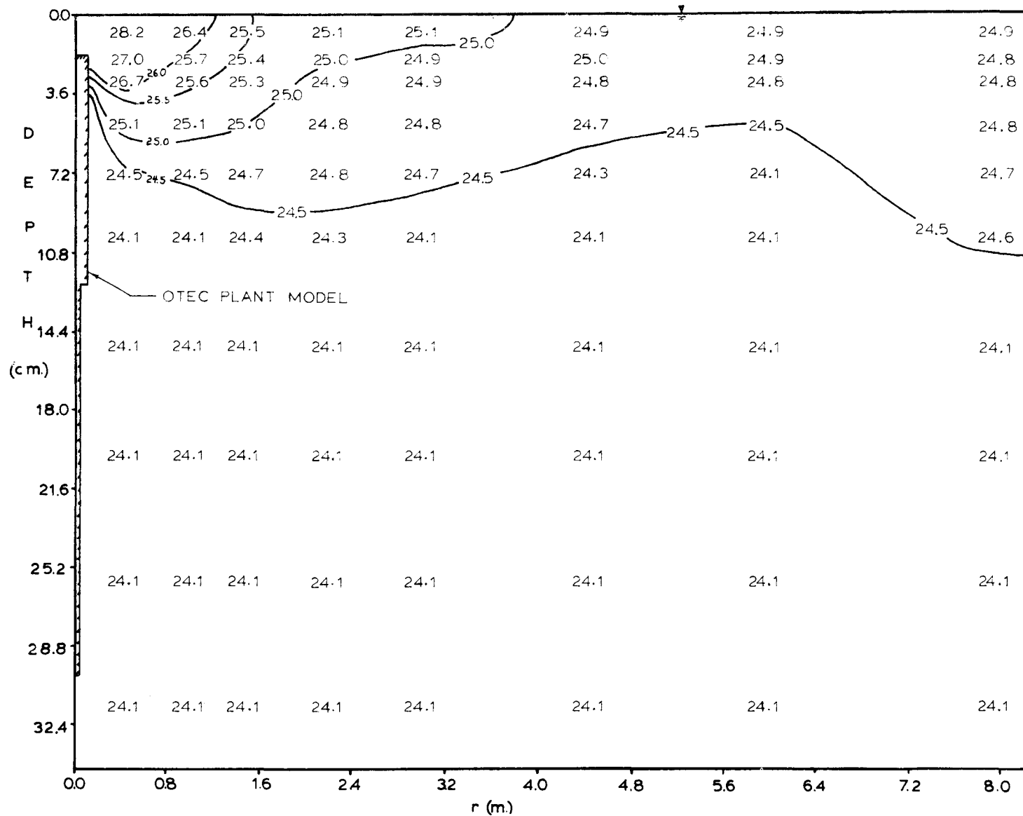
Figure 5.2 Centerline Temperature (°C) Transect Through the Right Jet, Experiment 11.
