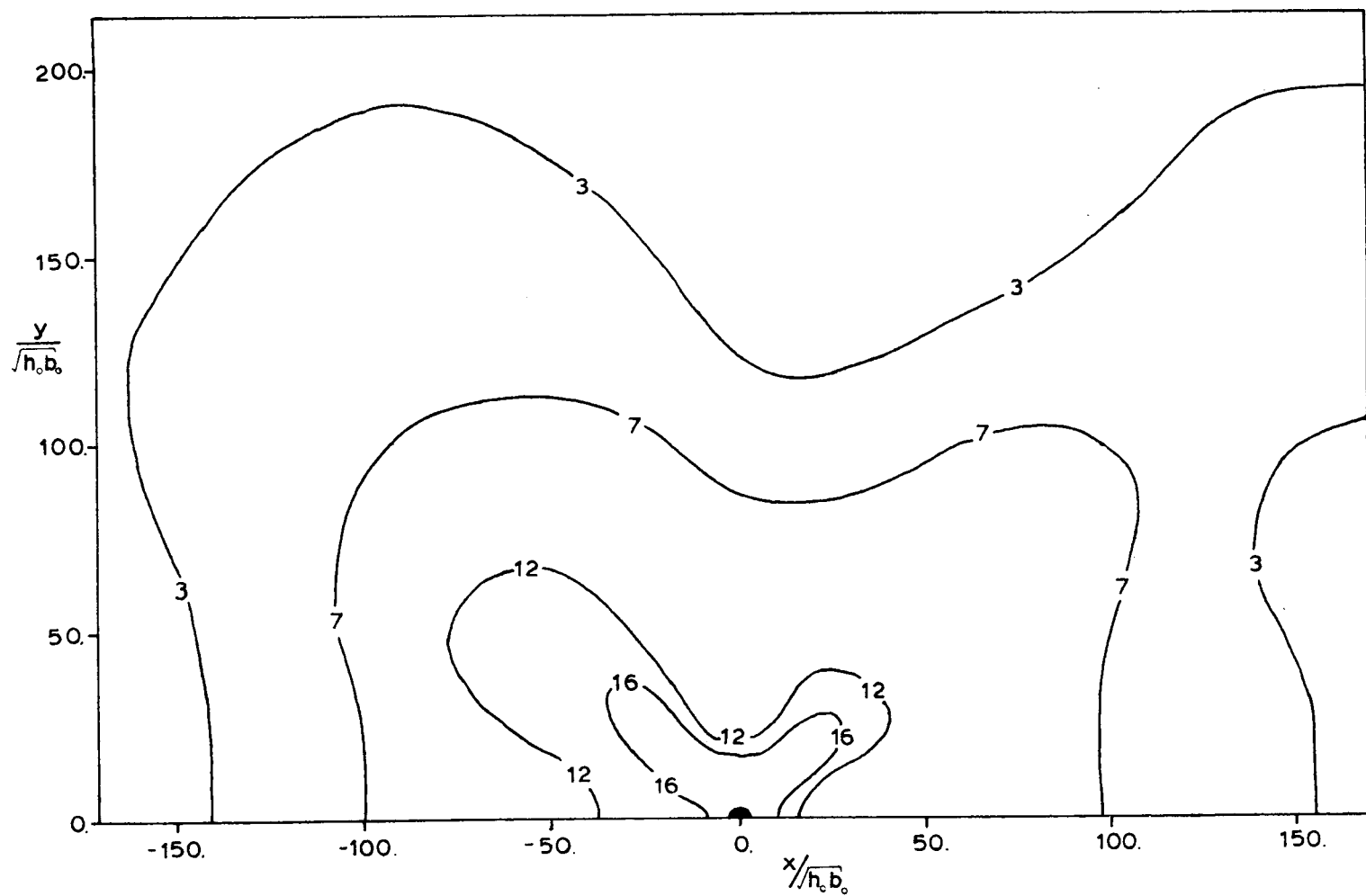
Figure A.2.7 Plan View. Run #12.
