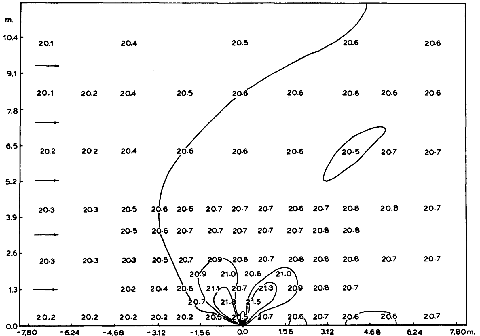
Figure 6.2 Typical Plan View of Surface Isotherms, Cross-Flow Experiment #18 Separate Jet Discharge, Half Model
