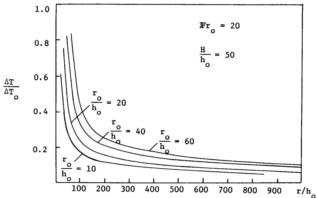
Figure 7.3a Temperature vs. Distance, Varying r_o/h_o
