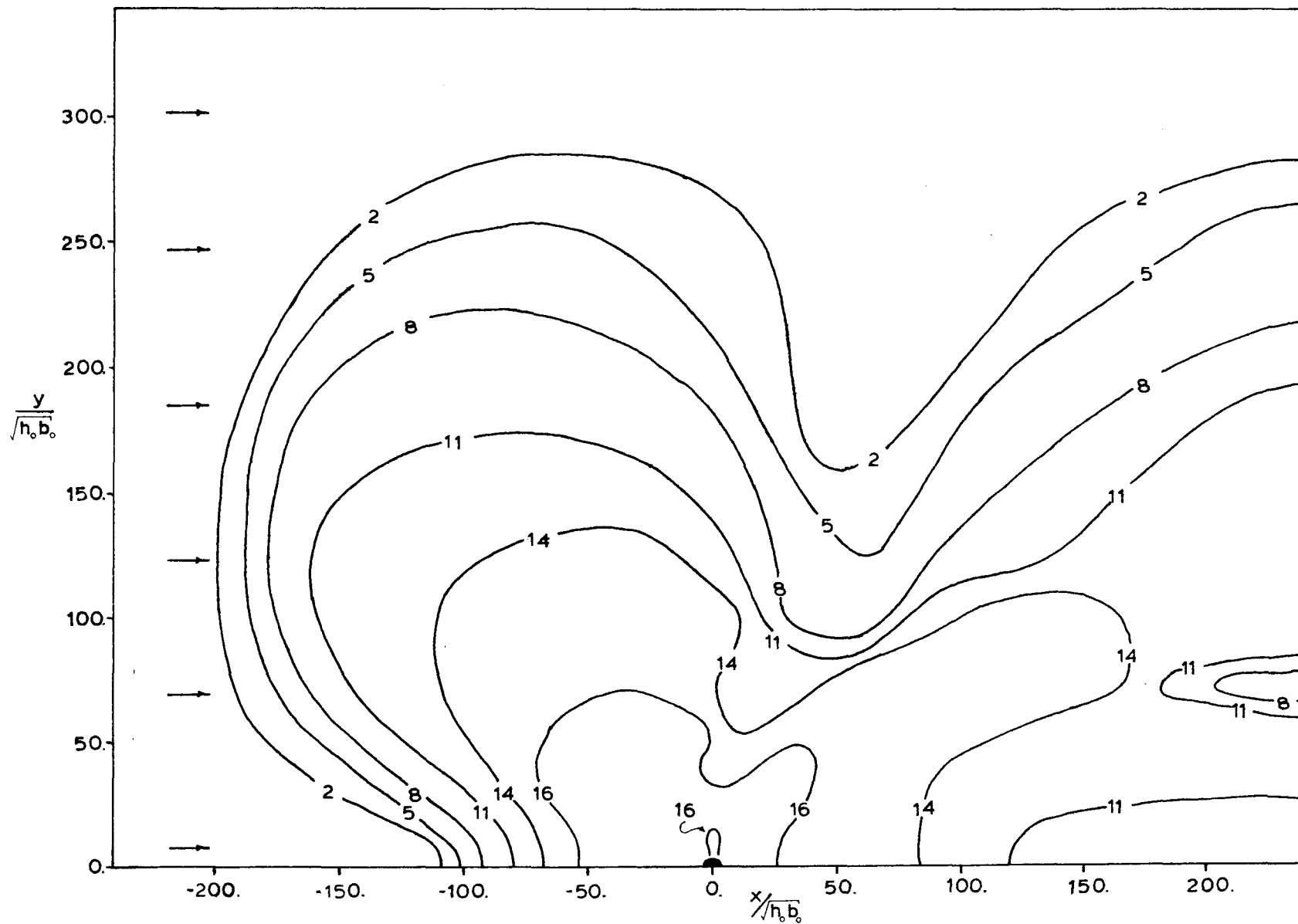
Figure A.3.10 Plan View of Run #20, Separate Jet Discharge.
