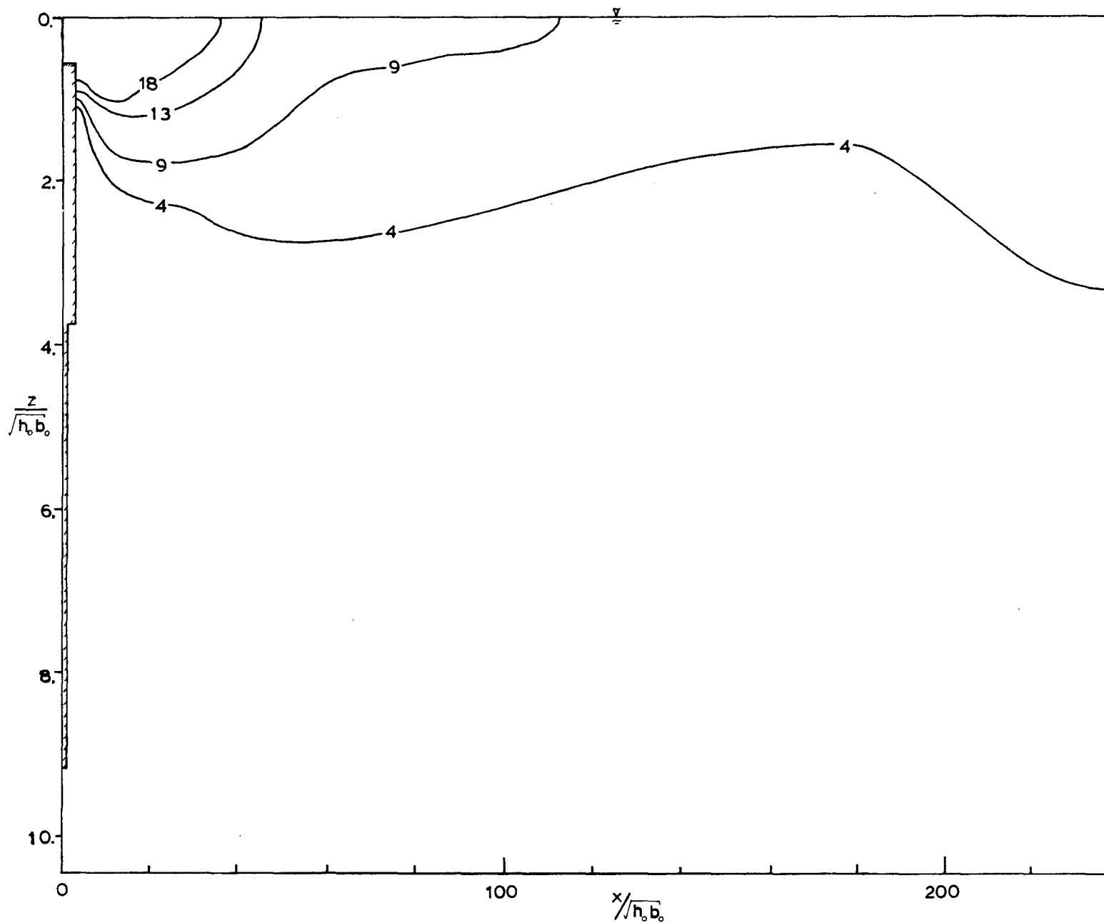
Figure A.2.5 Centerline Section of Jet #1. Run #11.
