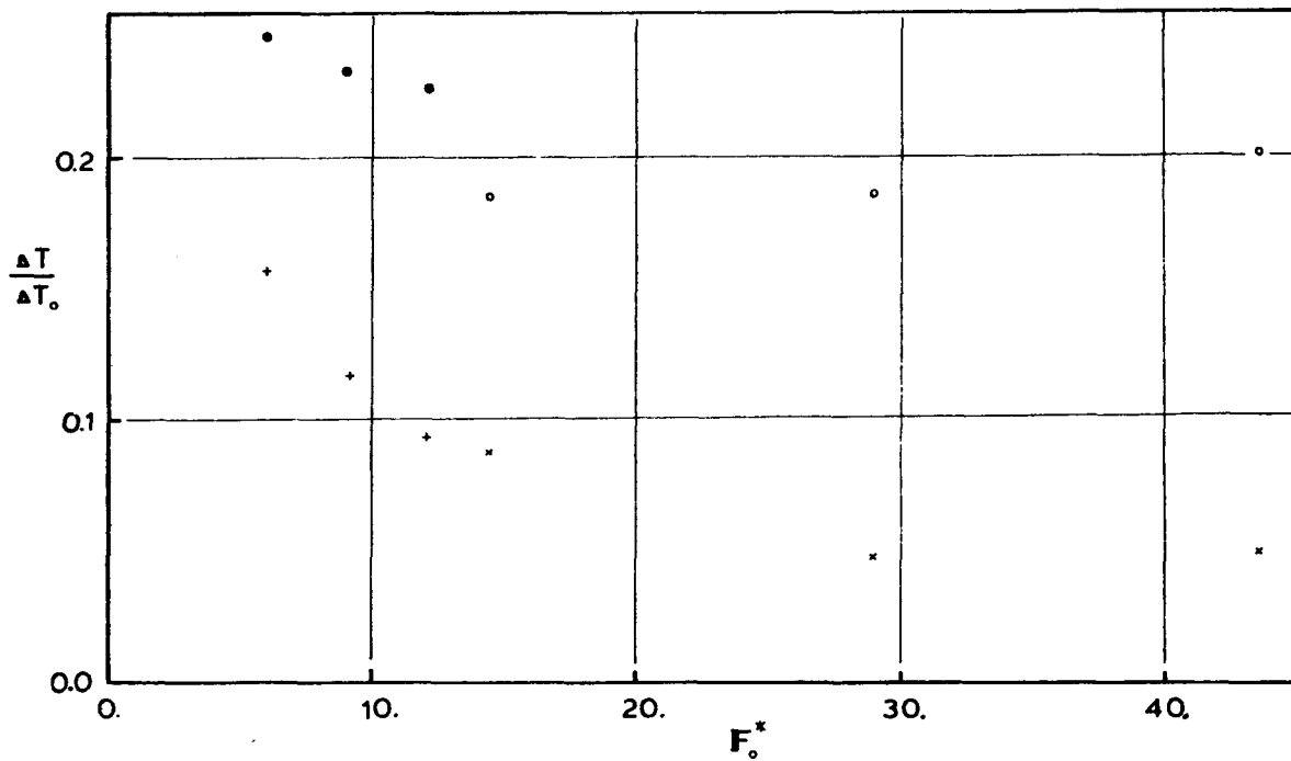
Figure 5.8a Comparison of Jet Centerline and Lateral Return Flow Surface Temperature Data at X = 1.0m .
