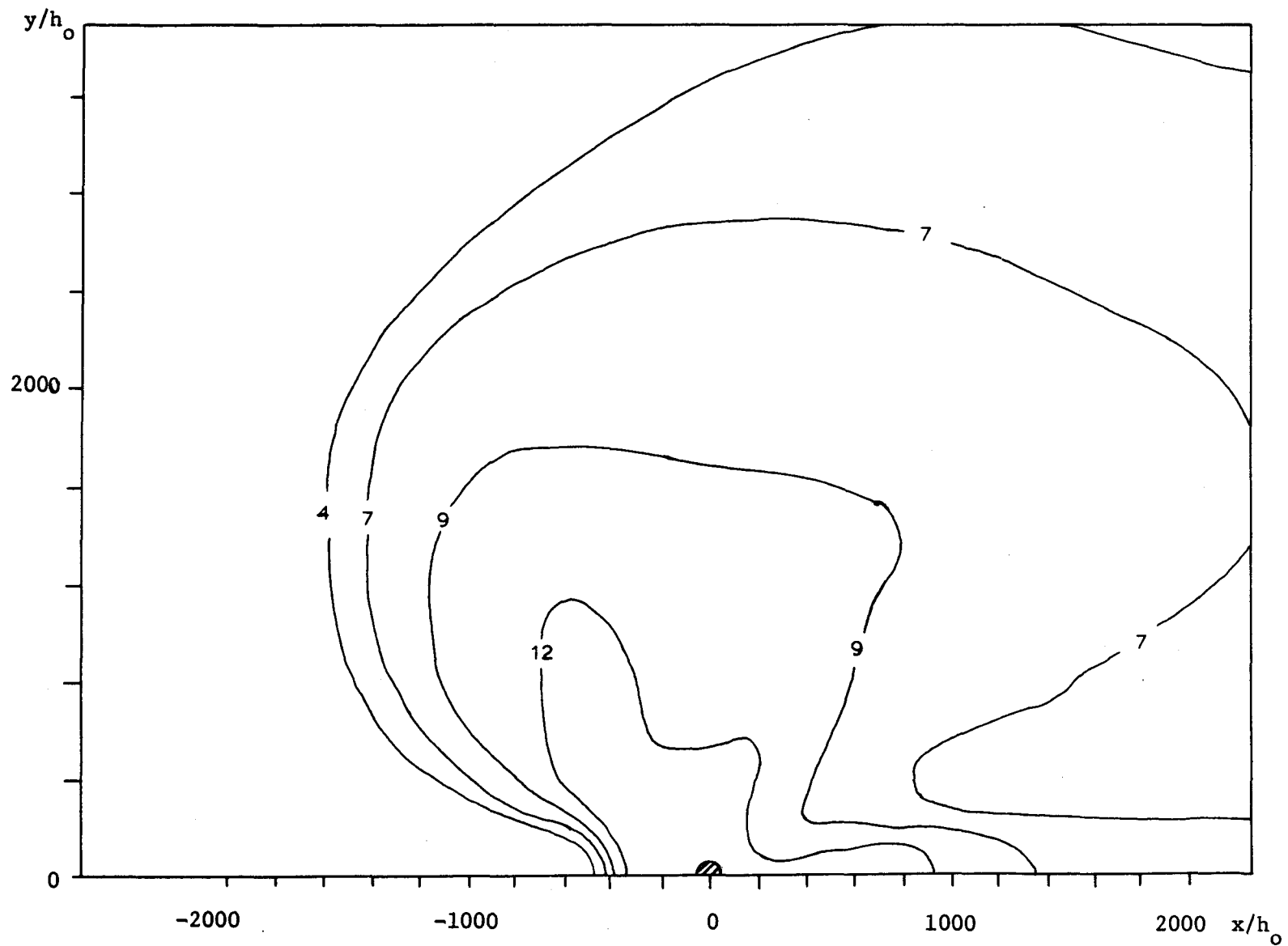
Figure A.3.16 Surface Plan, Run #22.
