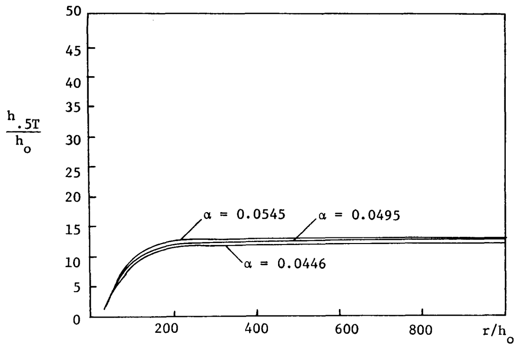
Figure 7.5b Half-Temperature Depth vs. Distance, Varying \alpha
