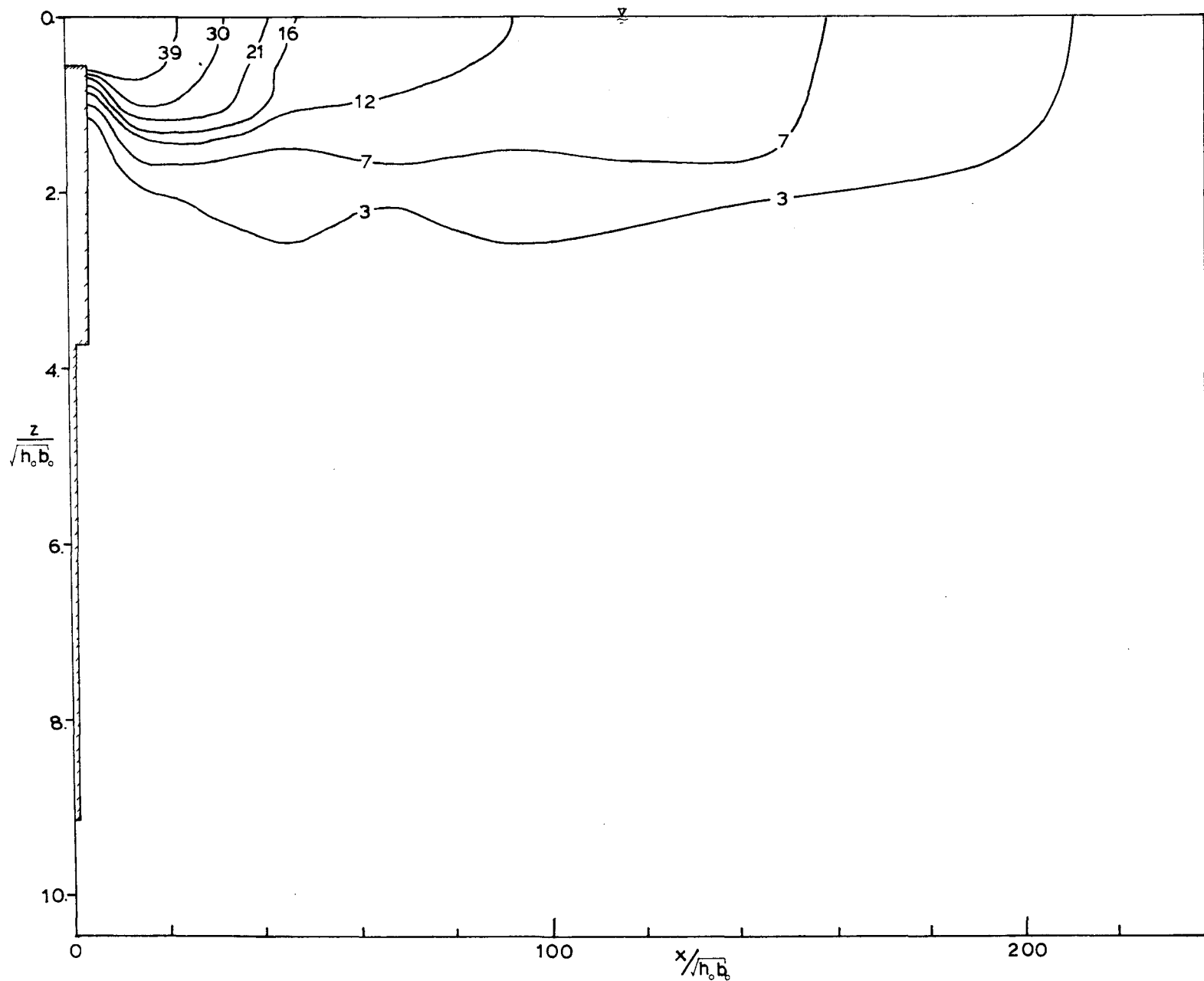
Figure A.2.9 Centerline Section of Jet #2. Run #12.
