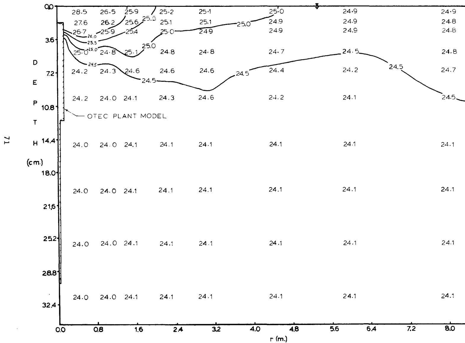
Figure 5.3 Centerline Temperature Transect Through the Left Jet, Experiment 11.
