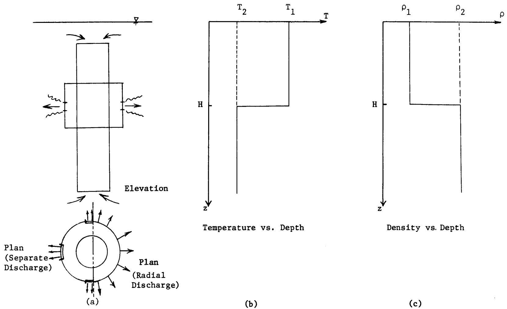
Figure 2.1 Schematization of OTEC Plant and Ambient Stratification Conditions
