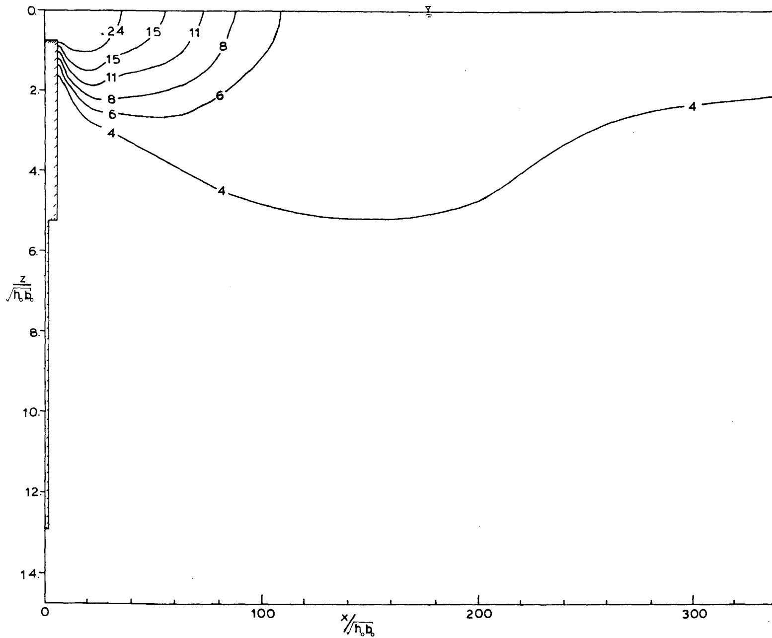
Figure A.2.15 Centerline Section of Jet #2. Run #14.
