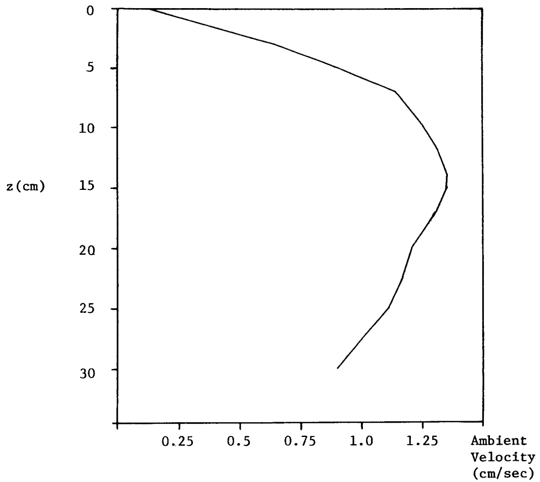
Figure 6.1 Typical Ambient Vertical Velocity Profile, Cross-Flow Experiment
