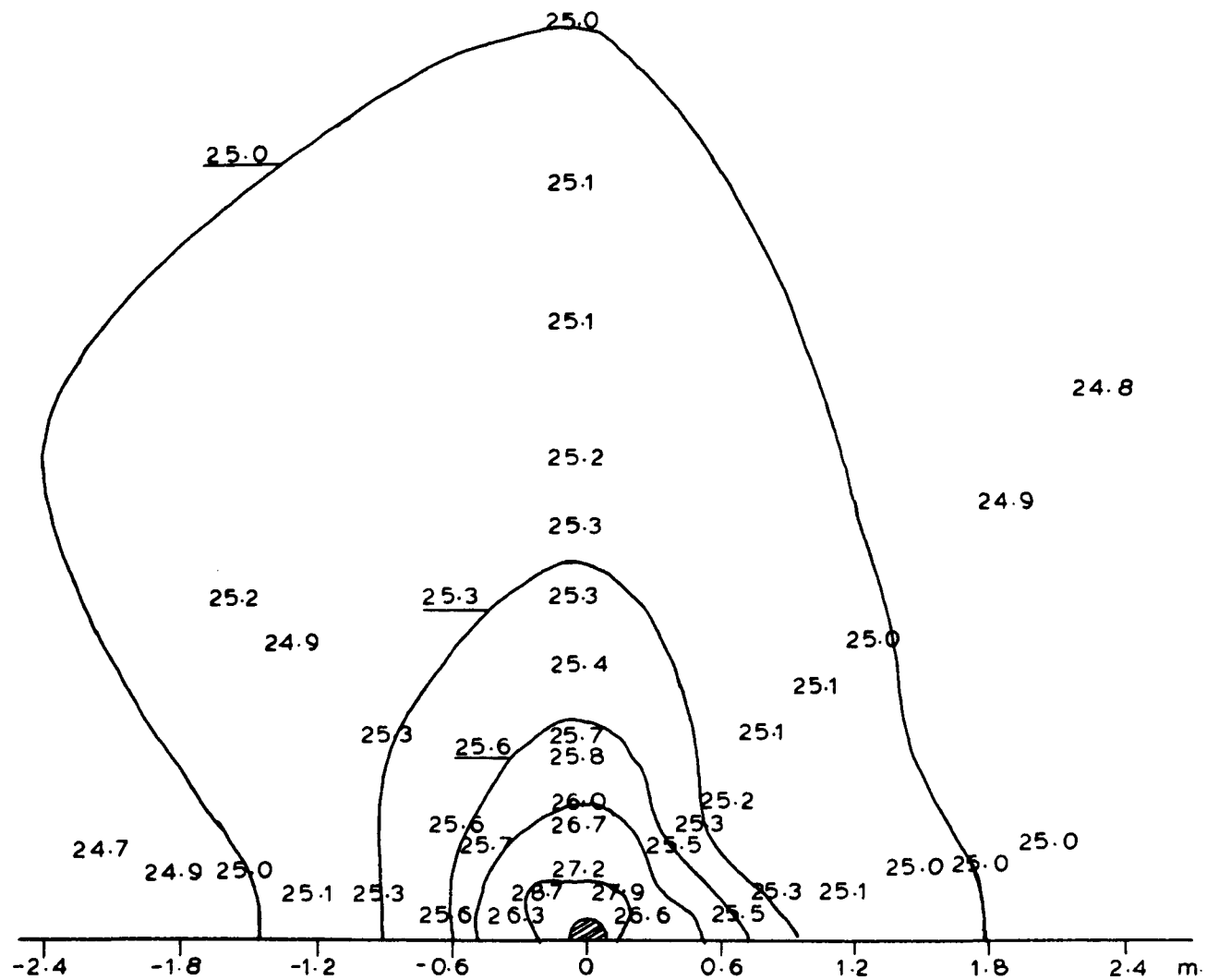
Figure 4.3 Typical Plan View of Surface Isotherms, Stagnant Experiment with Radial Discharge (Exp. No. 1)
