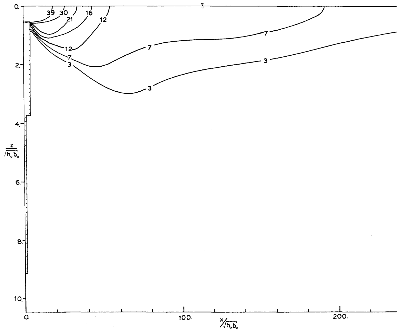
Figure A.2.8 Centerline Section Jet #1. Run #12.
