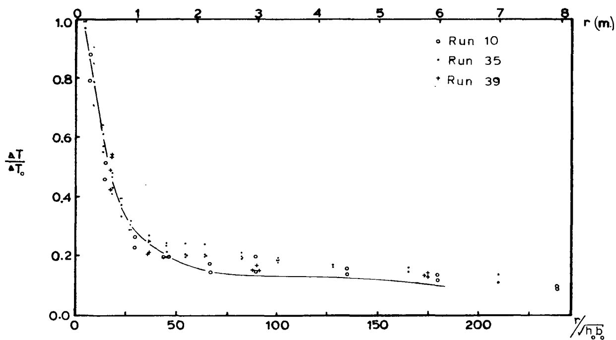
Figure 8.9a Temperature vs. Distance, Experimental Comparison to Model
