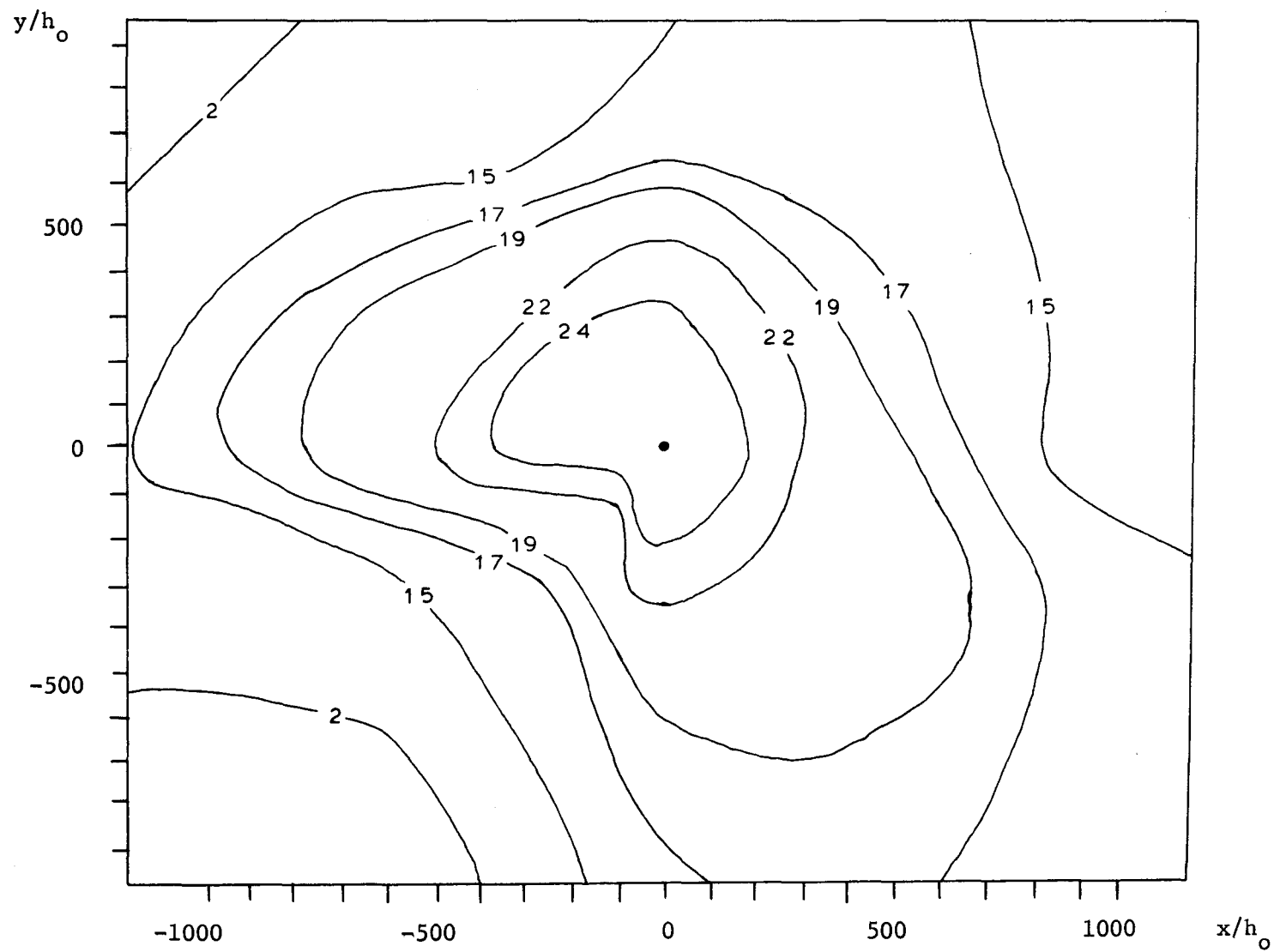
Figure A.3.25 Surface Plan, Run #32, Radial Jet Discharge.
