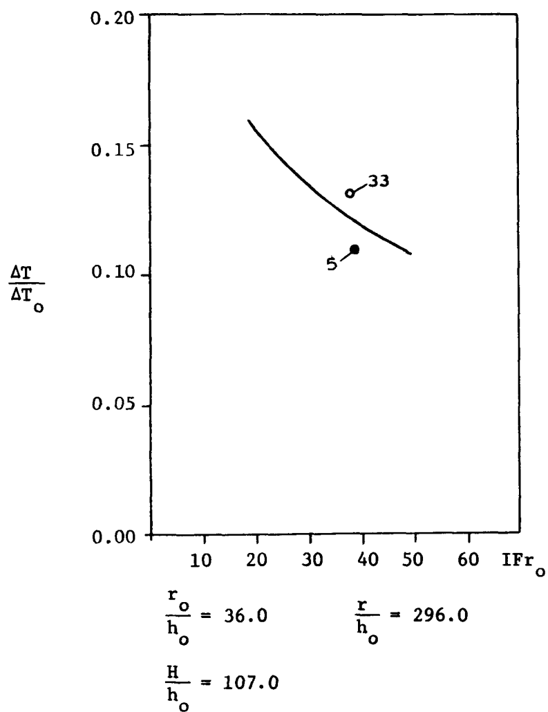
Figure 7.17a Normalized Temperature Difference vs. Discharge Densimetric Froude Number at a Radial Distance of \frac{r}{h_o} = 296.0
