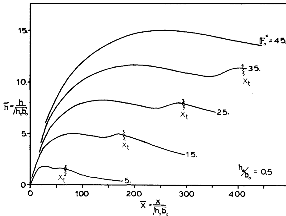
Figure 8.4b Jet Depth vs. Distance, Varying F_o^*
