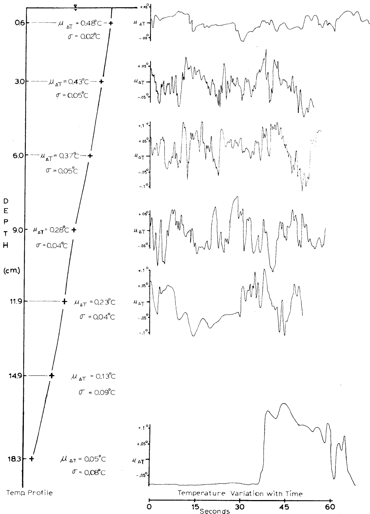
Figure C.4 Experiment #58 @ r = 2.13m
