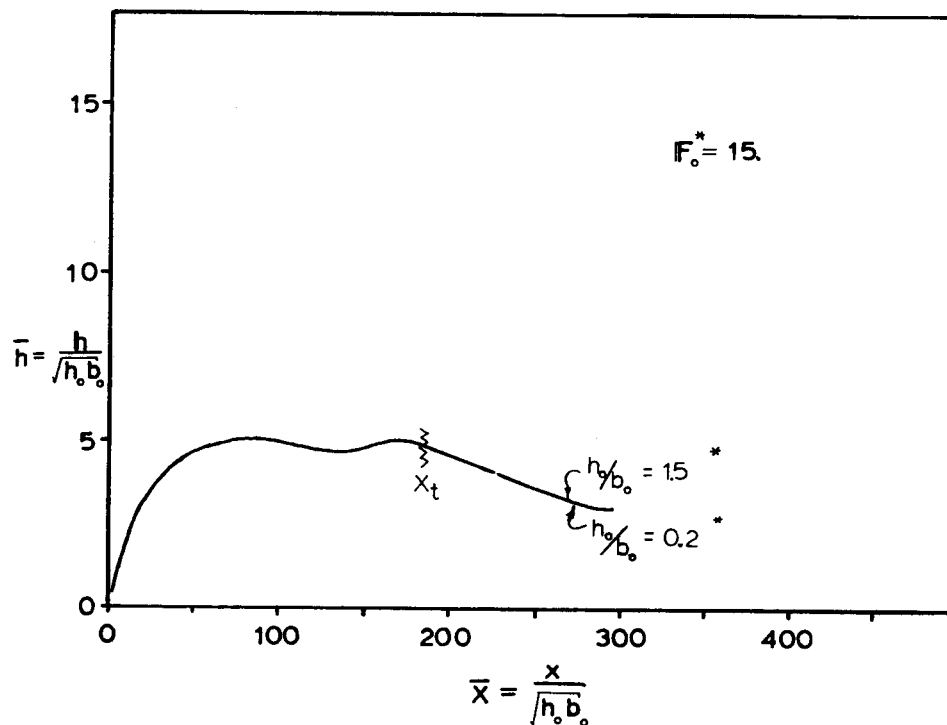
Figure 8.5b Jet Depth vs. Distance, Varying h_o/b_o
