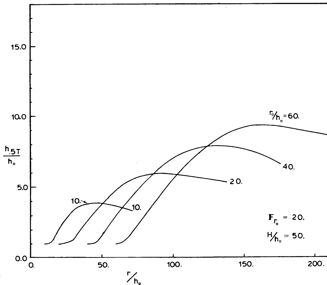
Figure 7.7 Half Temperature Depth vs Distance, Varying r_o/h_o ; Radial Interface Jet
