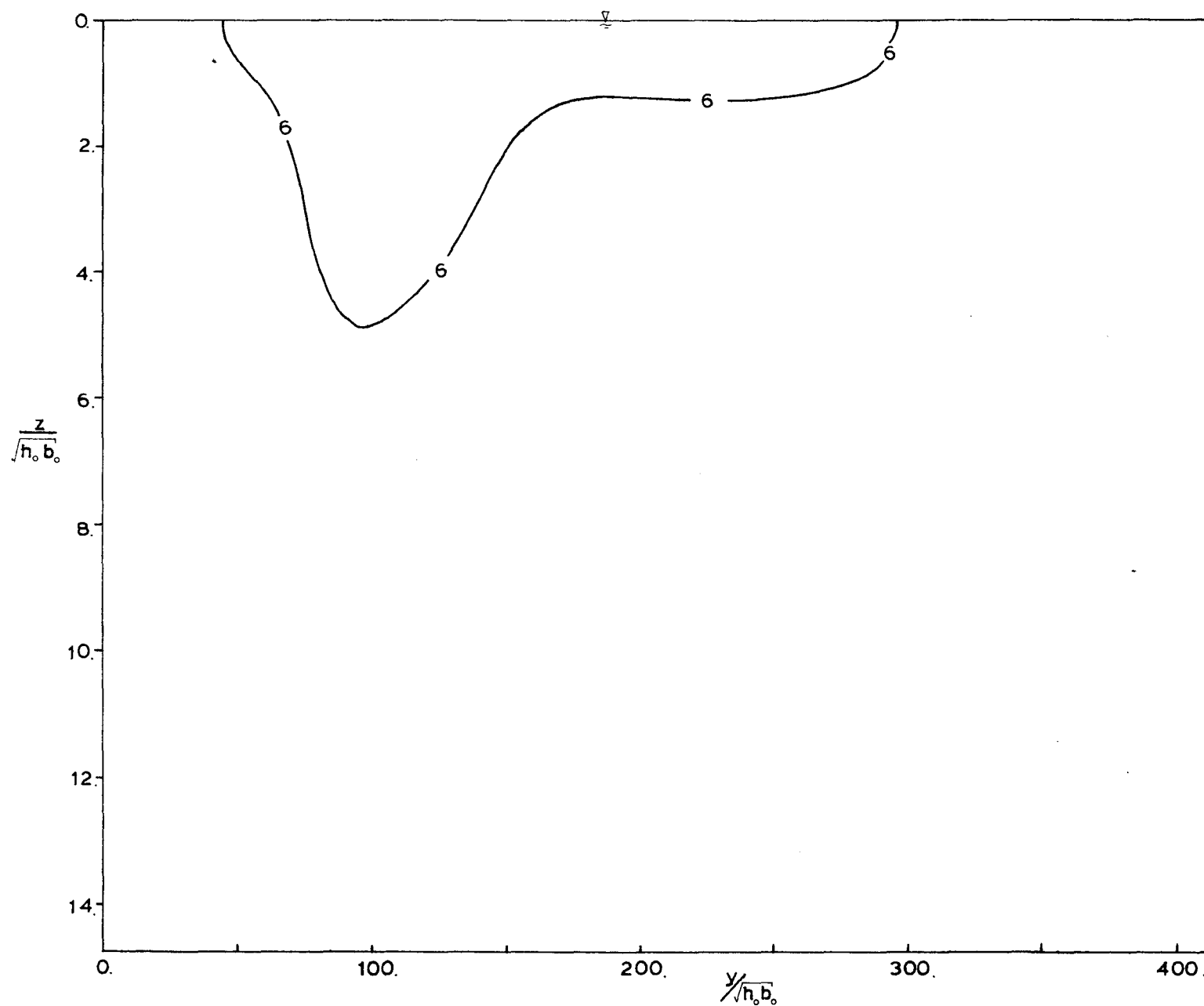
Figure A.3.3 Lateral Transect B-B at x = -2 m. Run #17.
