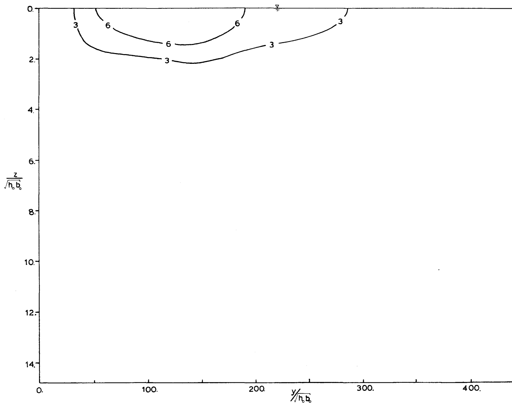
Figure A.3.9 Lateral Transect B-B at x = -4\text{m} , Run #19.
