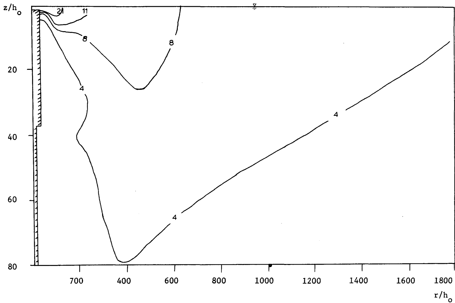
Figure A.1.7 Radially Averaged Cross-Section. Run # 8
