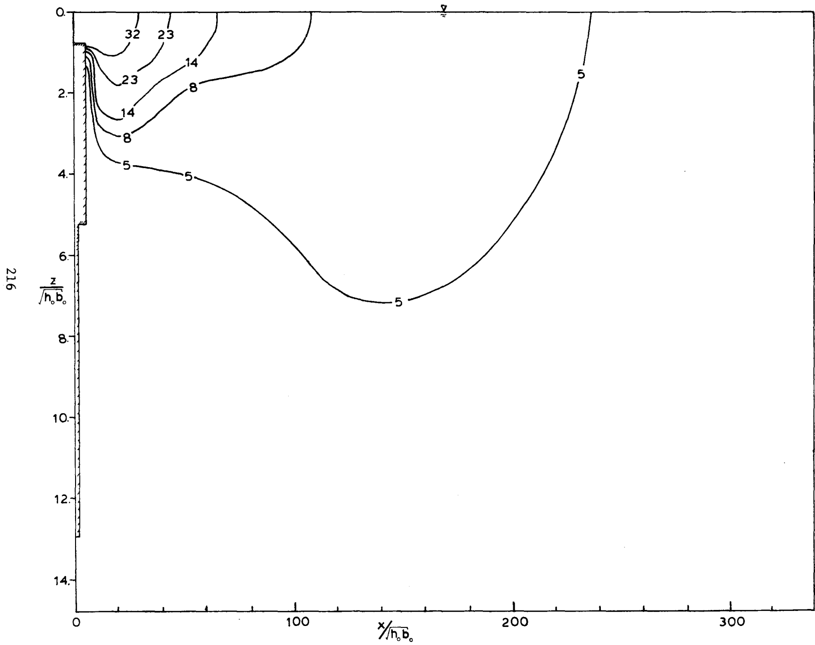
Figure A.2.17 Centerline Section of Jet #1. Run #15.
