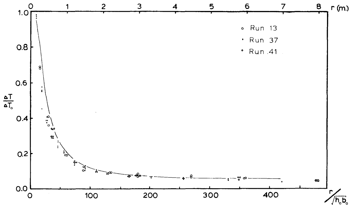
Figure 8.12a Temperature vs. Distance, Experimental Comparison to Model
