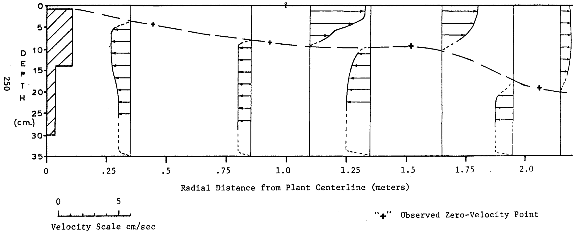
Figure B.2 Photographic Velocity Measurement Exp #51
