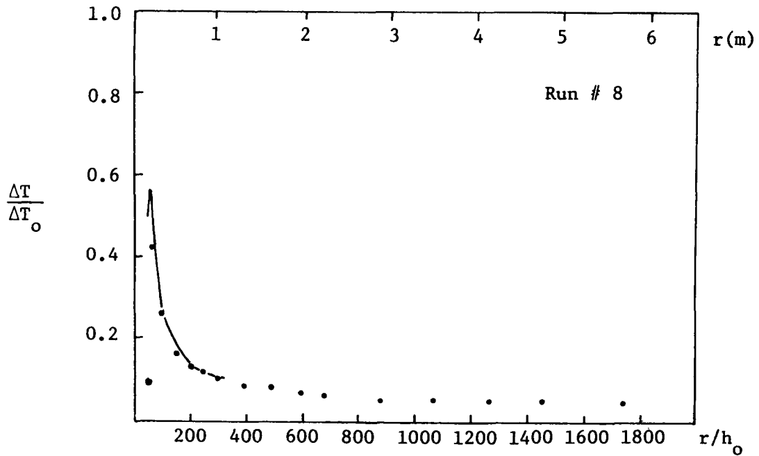
Figure 7.19a Temperature vs. Distance, Experimental Comparison to Model
