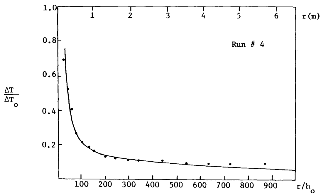
Figure 7.13a Temperature vs. Distance, Experimental Comparison to Model
