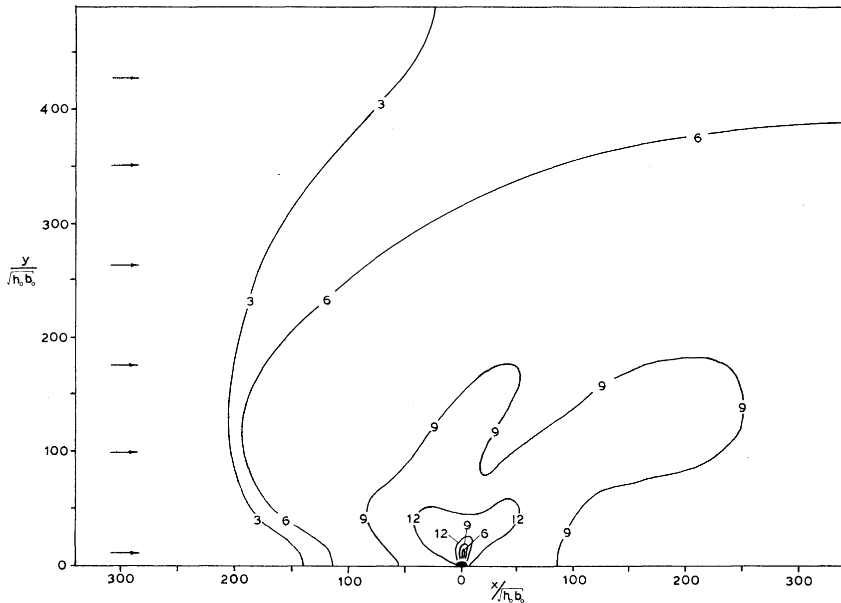
Figure A.3.7 Plan View of Run #19, Separate Jet Discharge
