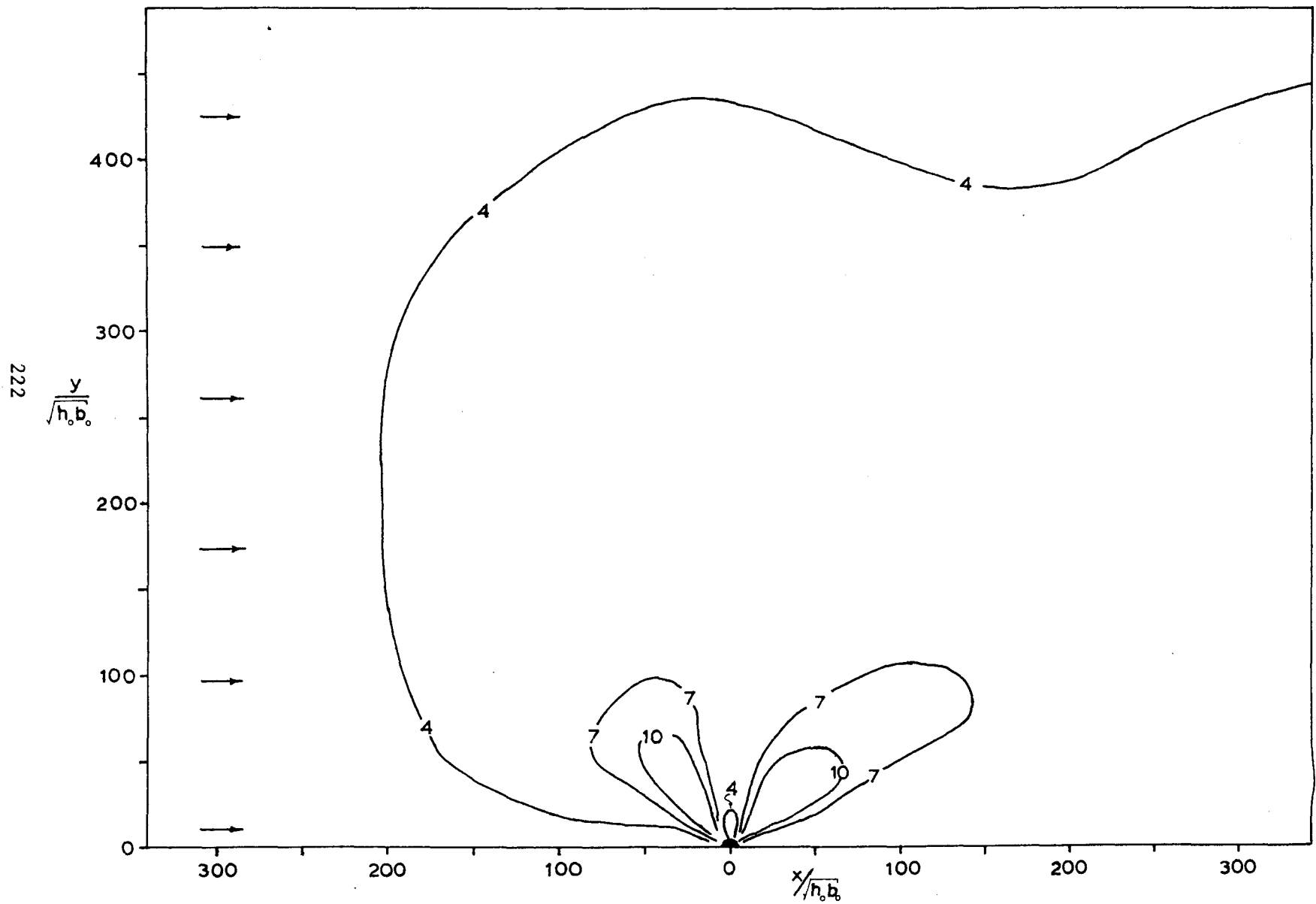
Figure A.3.4 Plan View. Run #18, Separate Jet Discharge
