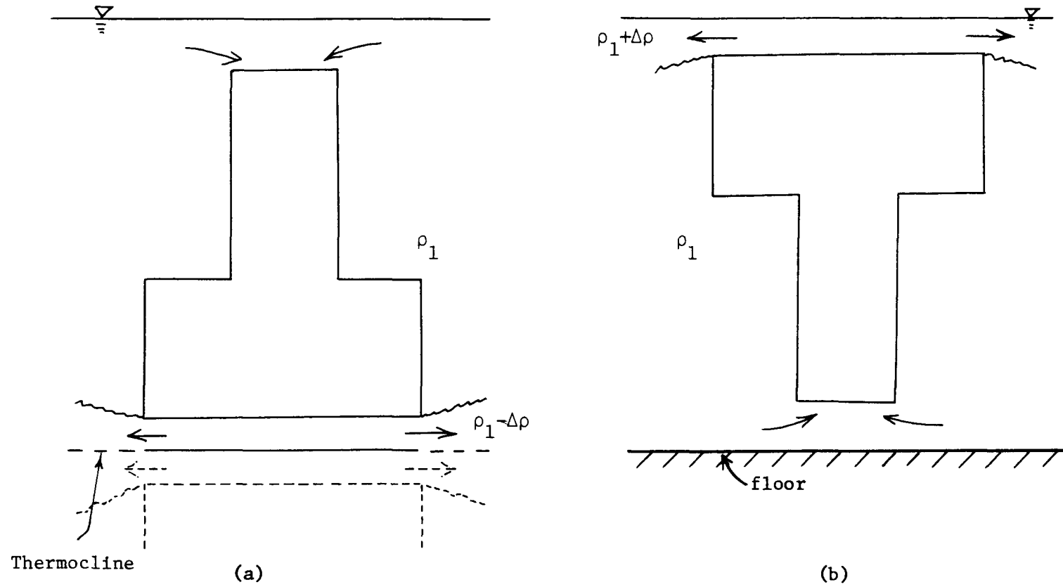
Figure 2.4 Schematization of the Upper Ocean Layer (a) and the Inverted Laboratory Model (b)
