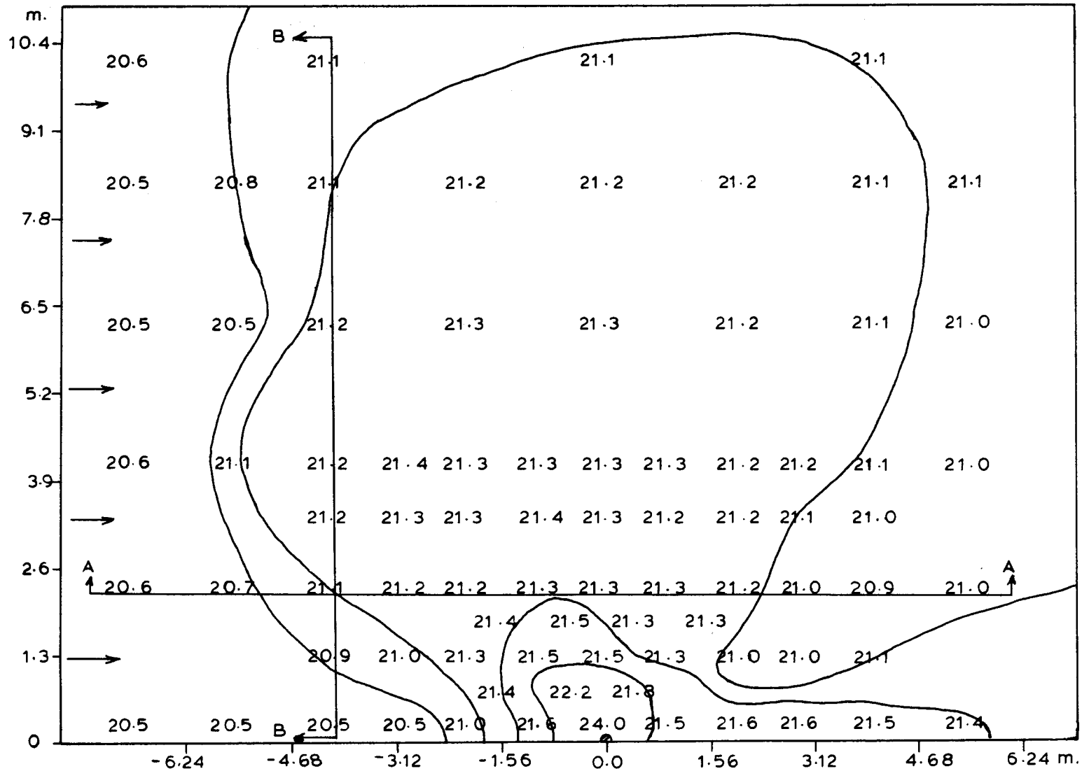
Figure 6.3 Typical Plan View of Surface Isotherms, Cross-Flow Experiment #21 Radial Discharge, Half Model
