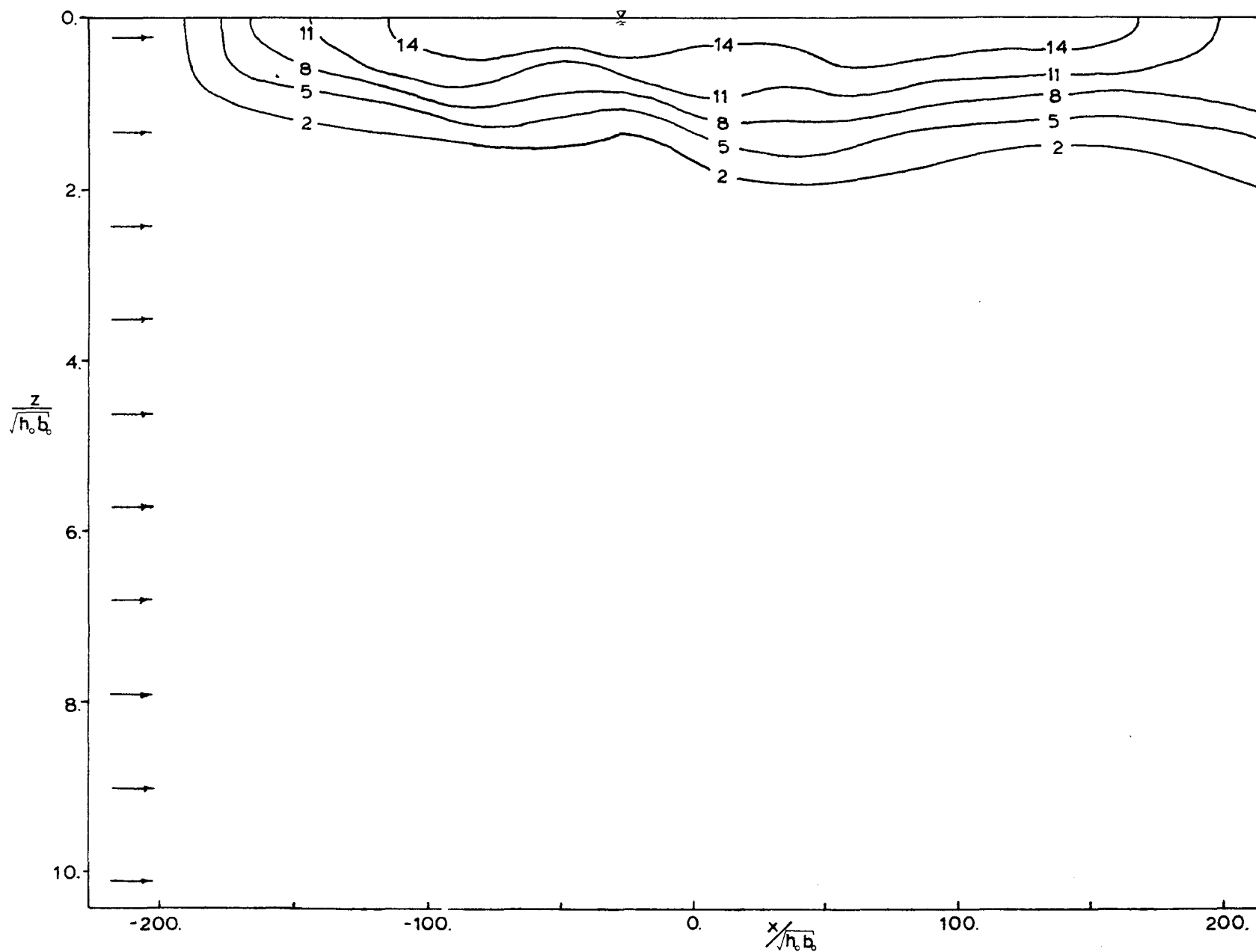
Figure A.3.11 Longitudinal Transect A-A at y = 2.25\text{m} , Run #20.
