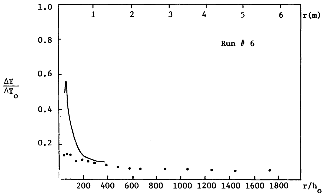
Figure 7.18a Temperature vs. Distance, Experimental Comparison to Model
