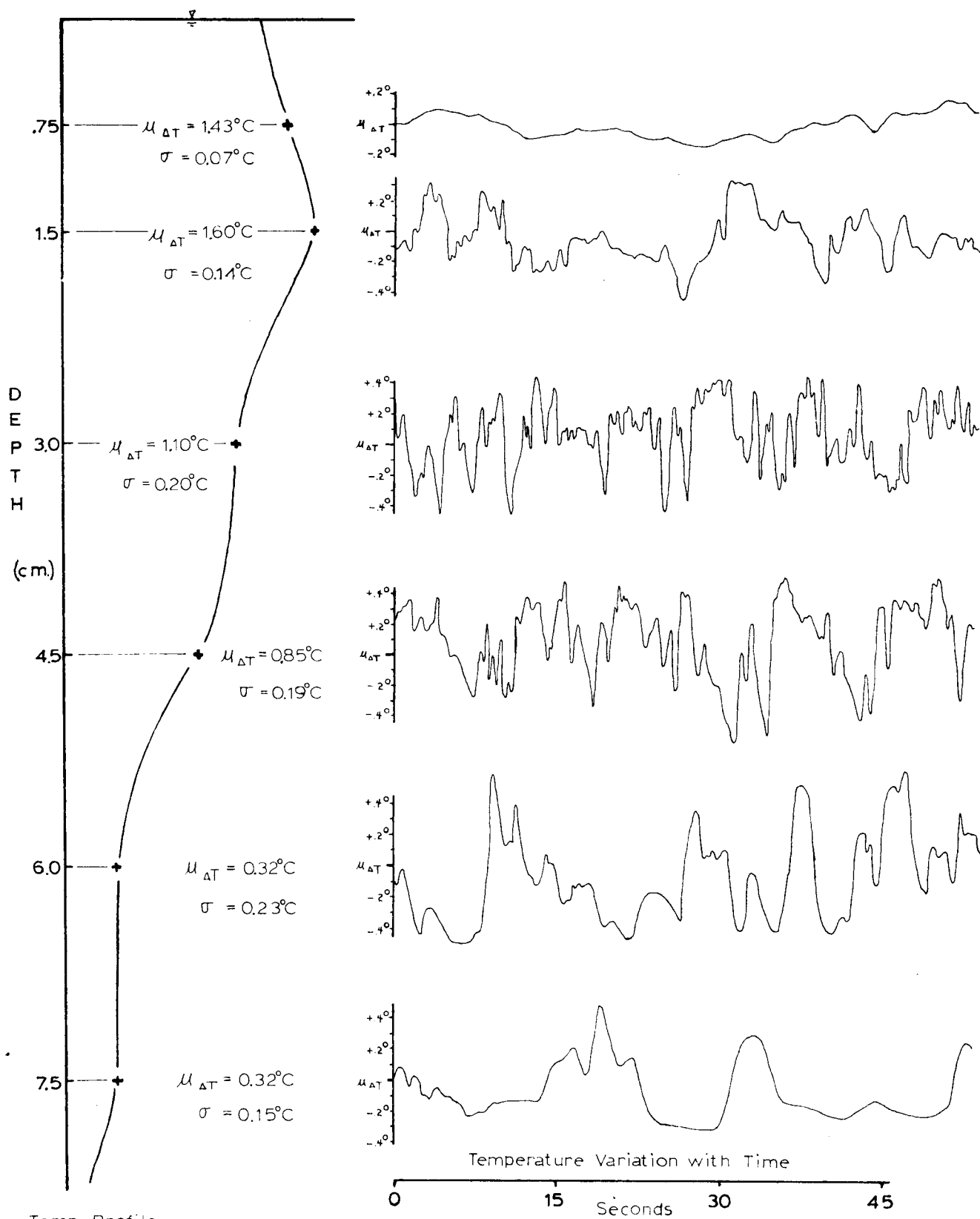
Figure C.1 Experiment #60 @ r = 0.91m
