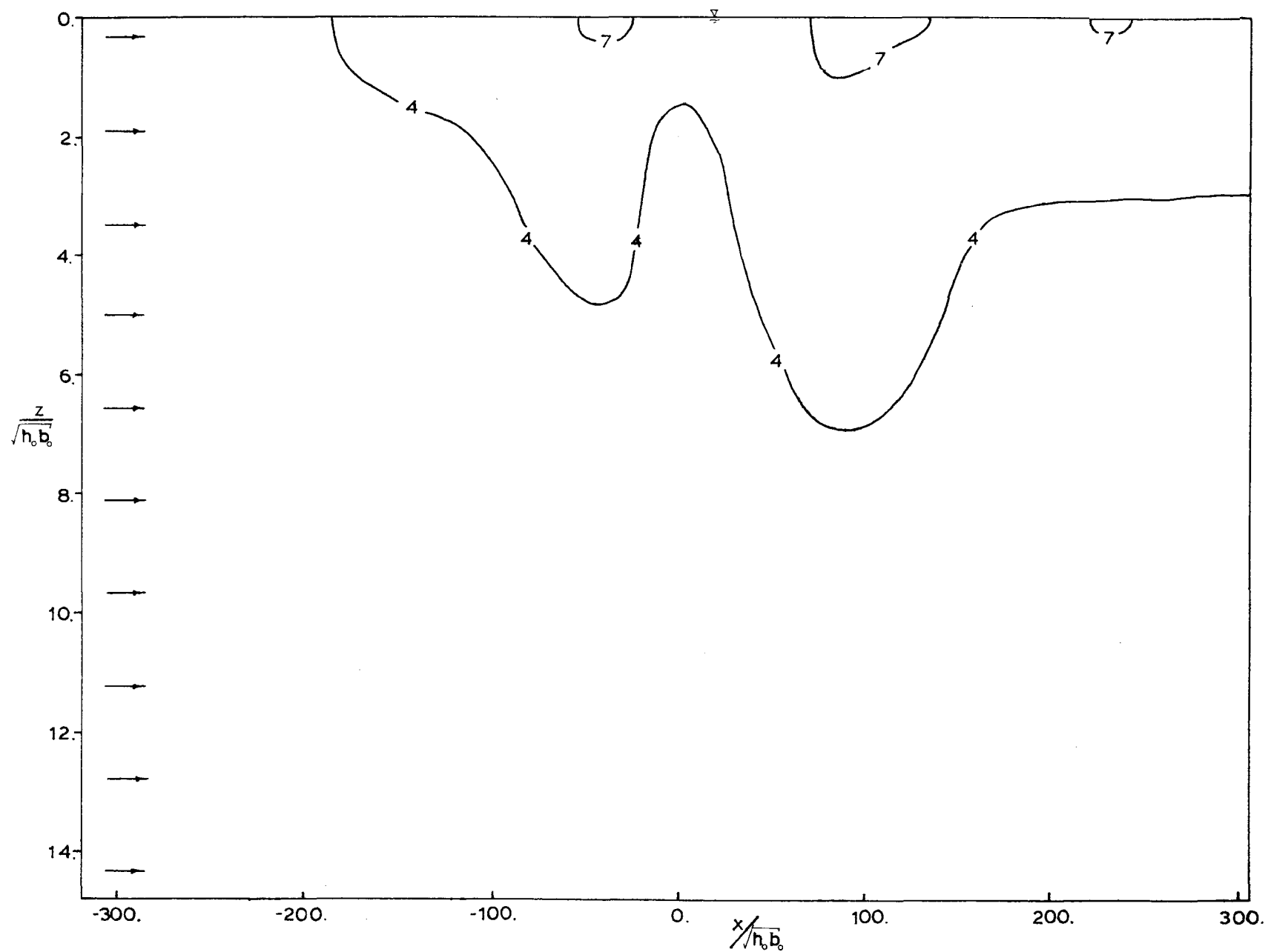
Figure A.3.5 Longitudinal Transect \Lambda - \Lambda . Run #18.
