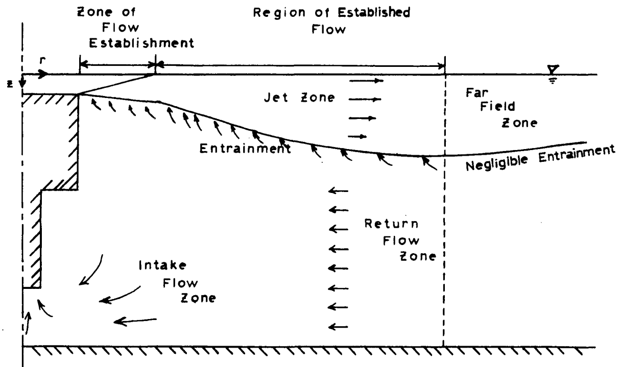
Figure 7.1 Schematic Diagram of the Induced External Flow Field.
