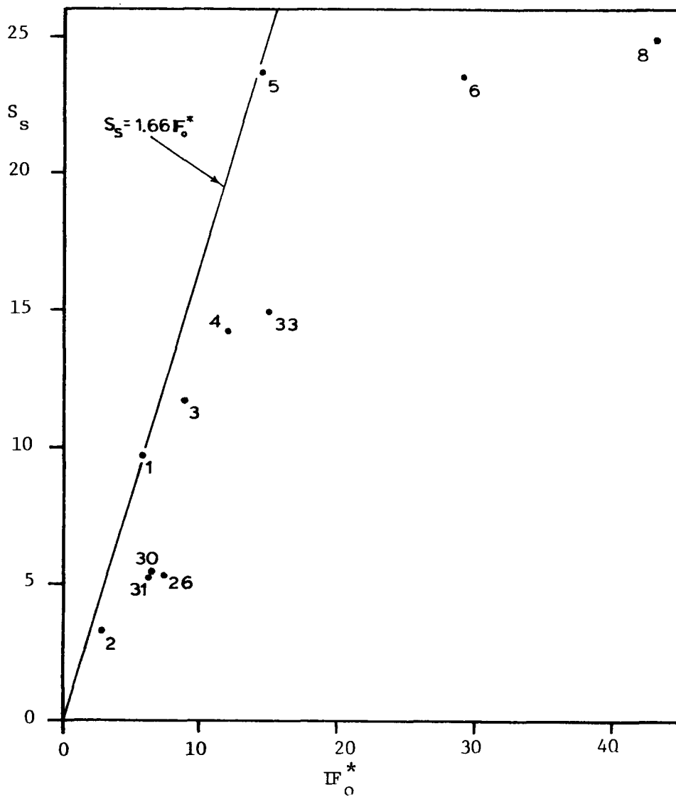
Figure 4.7 Stable Jet Dilution vs. Quarter Module "Port" Discharge Froude Number, Stagnant Experiments
