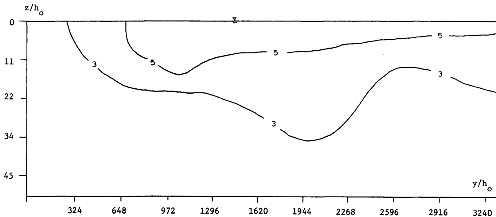
Figure A.3.15 Lateral Transect E-B at x = -4.0\text{m} , Run #21.
