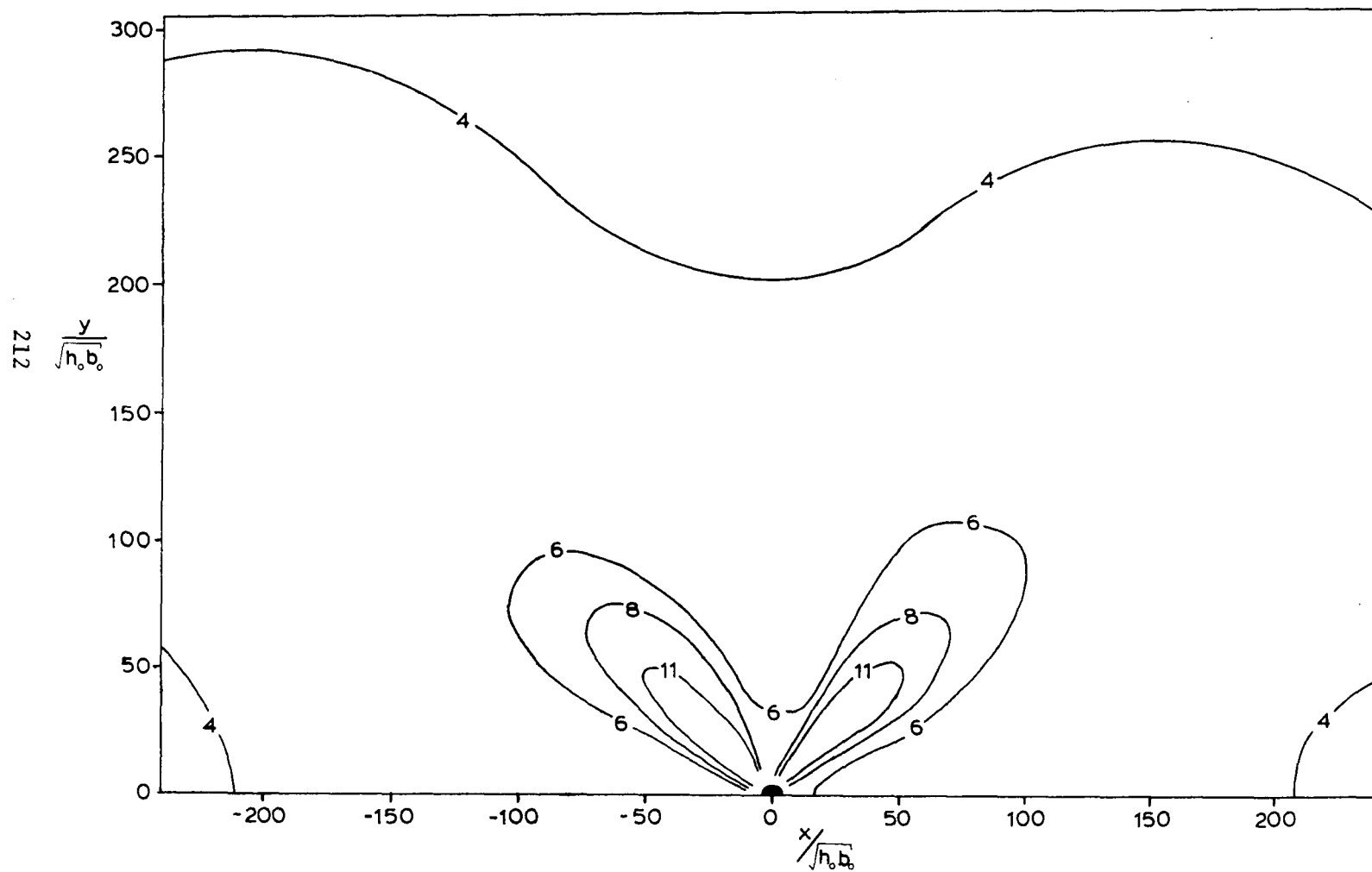
Figure A.2.13 Plan View. Run #14.
