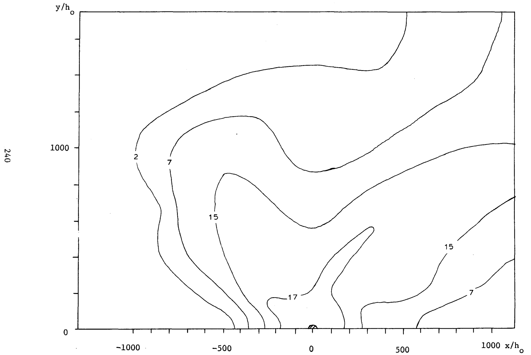
Figure A.3.22 Surface Plan, Run #24, Radial Discharge.
