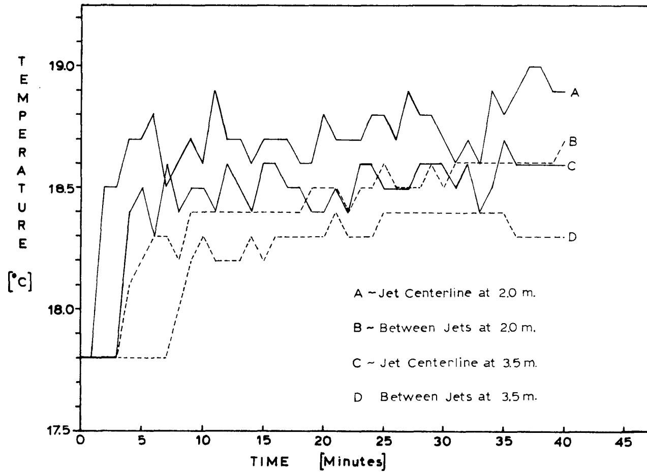
Figure 5.5 Steady-State Test for Stagnant Experiments with Separate Jet Discharge (Exp. #43)
