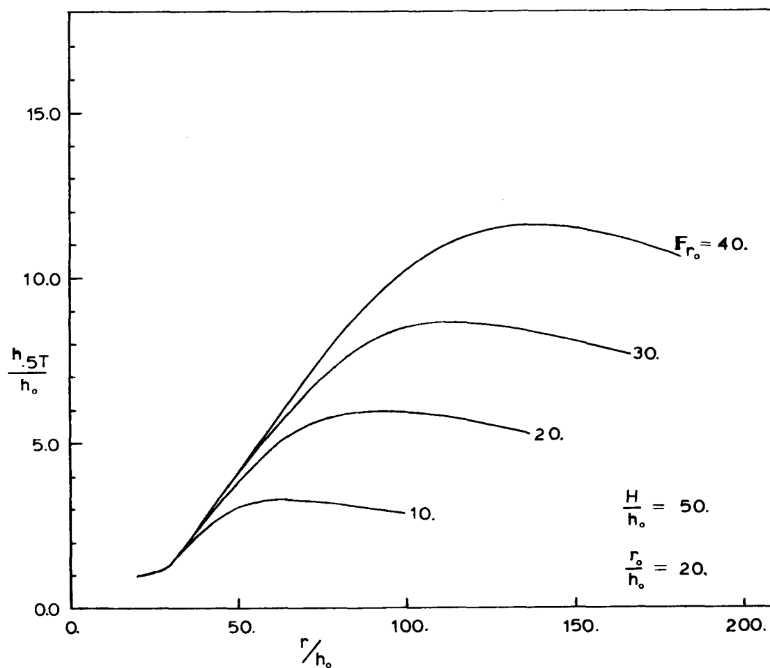
Figure 7.6 Half Temperature Depth vs. Distance, Varying F_{r_o} ; Radial Interface Jet.
