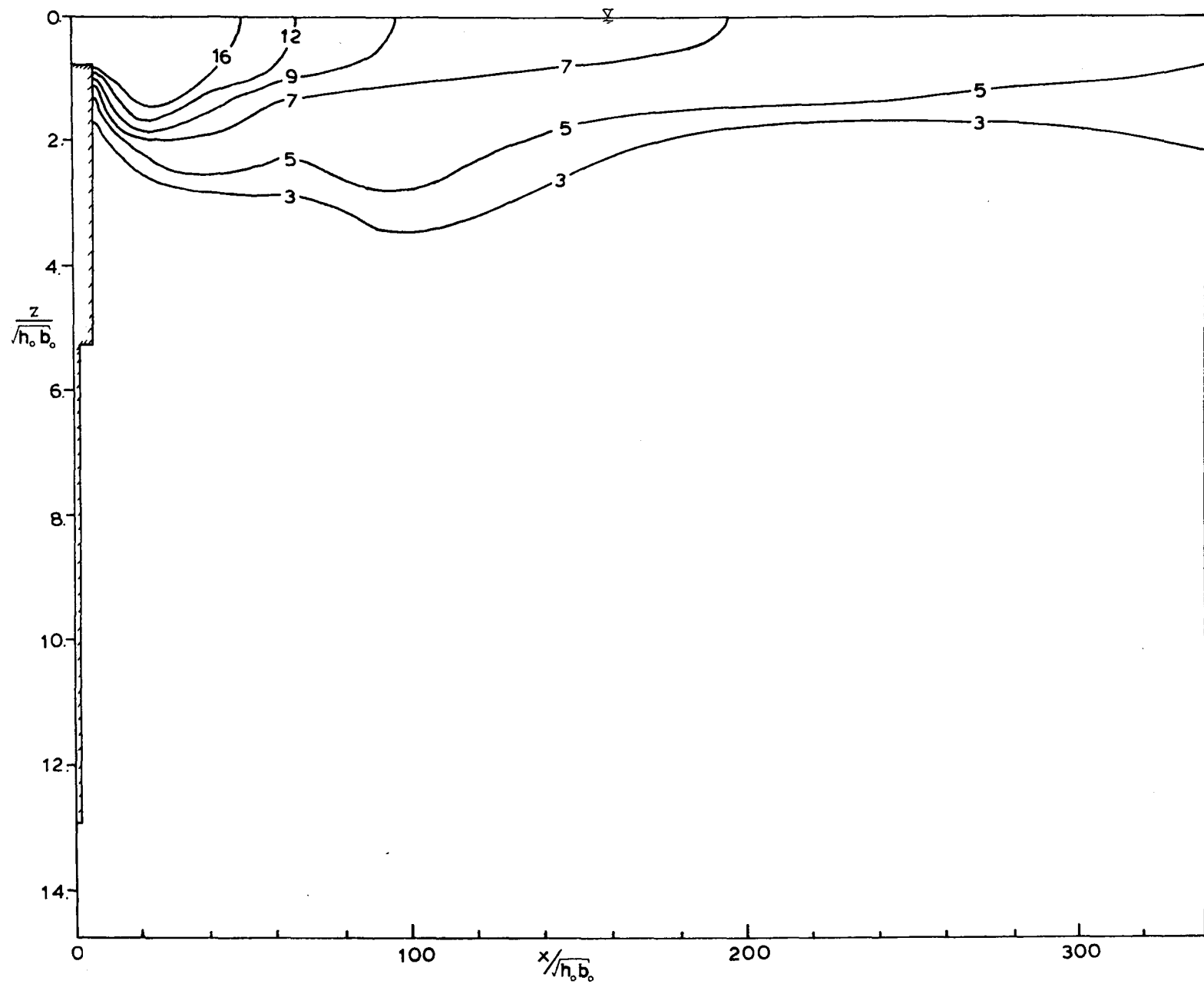
Figure A.2.11 Centerline Section of Jet #1. Run #13.
