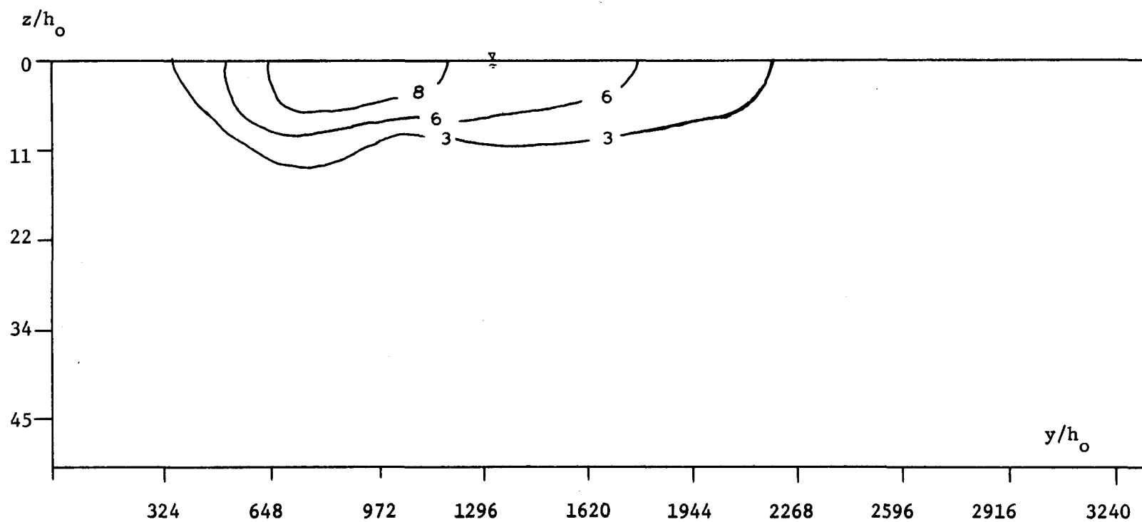
Figure A.3.21 Lateral Transect B-B at x = -4\text{m} , Run #23.
