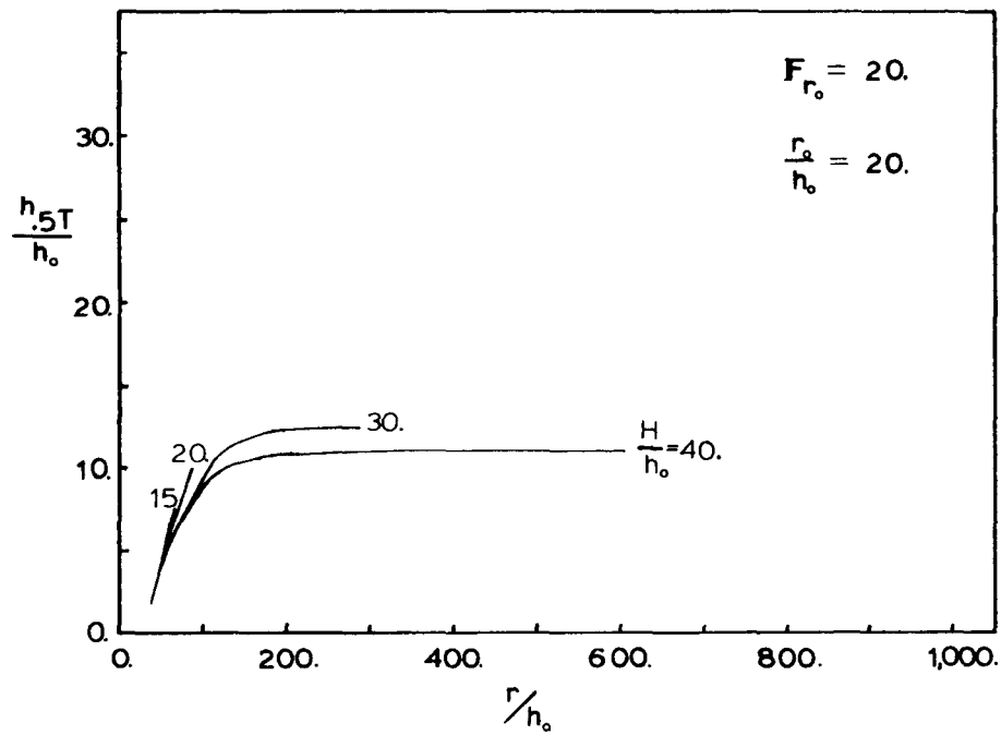
Figure 7.4b Half Temperature Depth vs. Distance, Varying H/h_0 .
