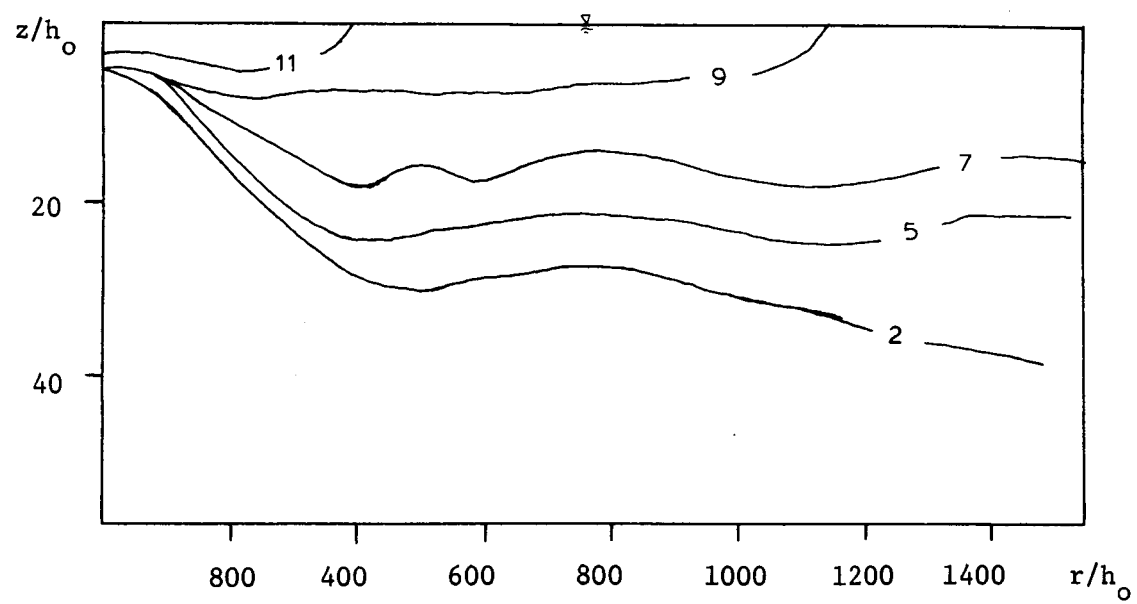
Figure A.1.9 Radially Averaged Cross-Section. Run # 33
