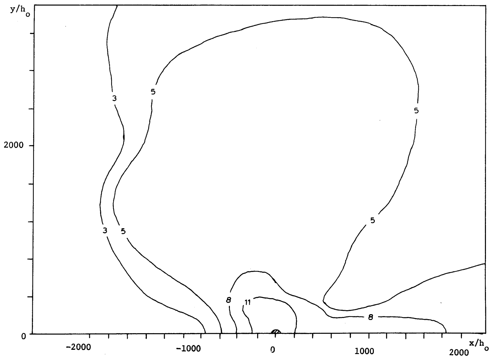
Figure A.3.13 Surface Plan, Run #21, Radial Jet Discharge
