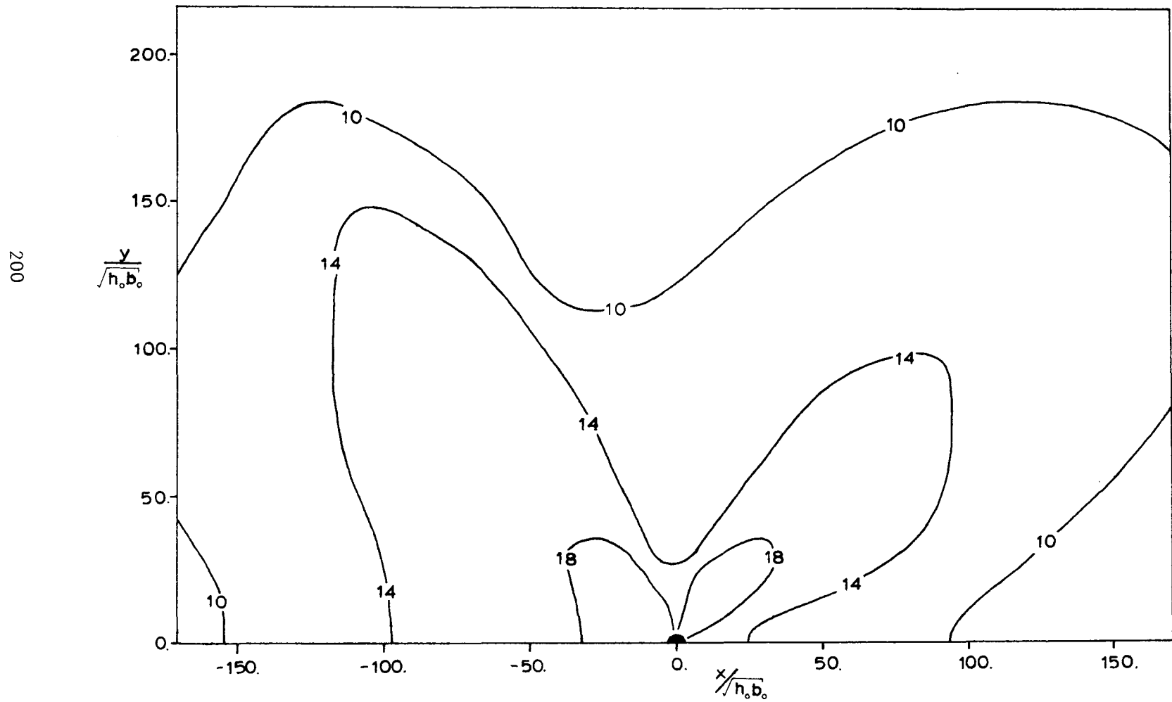
Figure A.2.1 Plan View. Run #10
