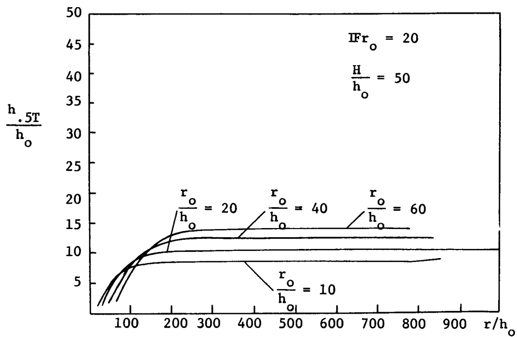
Figure 7.3b Half-Temperature Depth vs. Distance, Varying r_o/h_o
