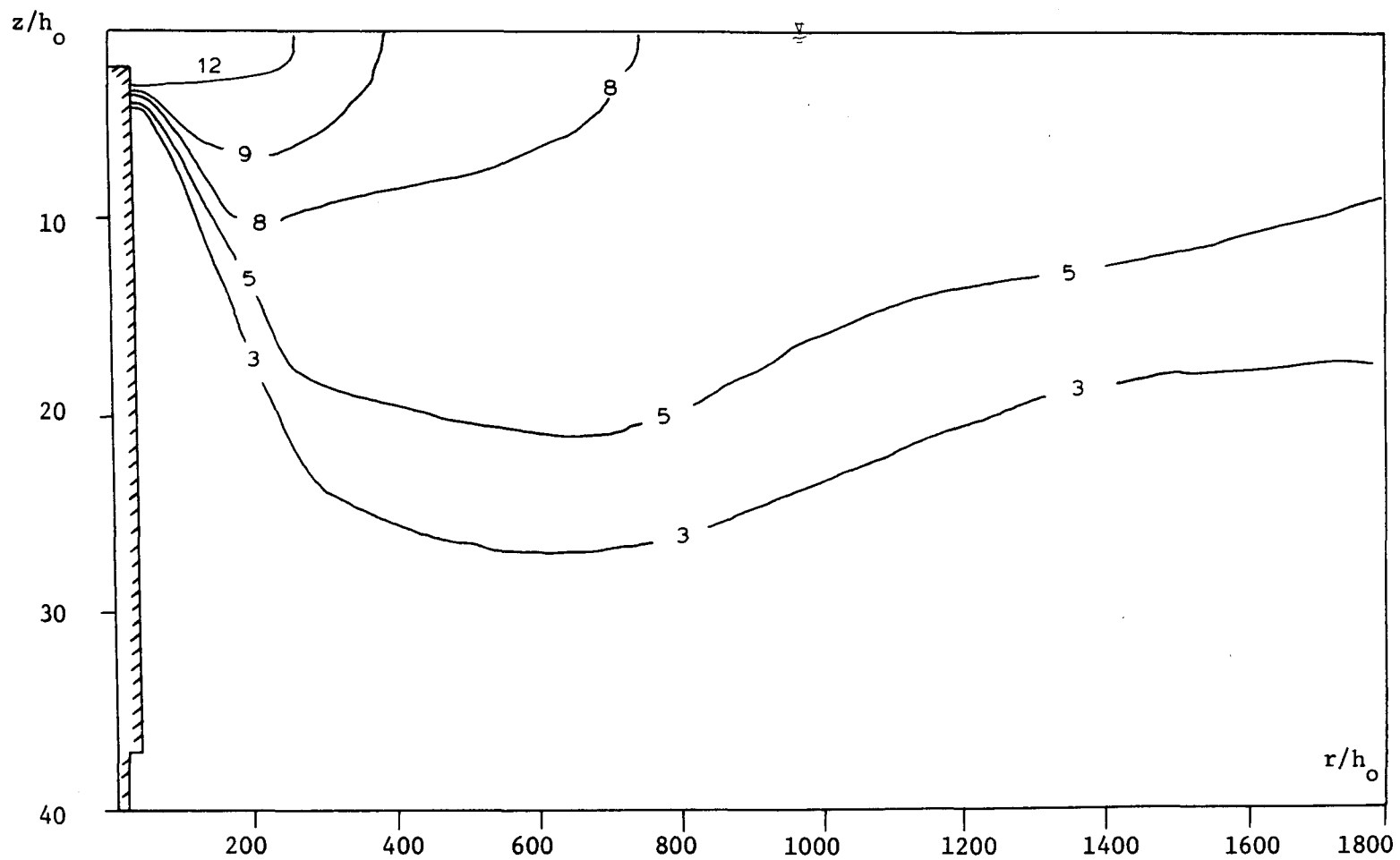
Figure A.1.5 Radially Averaged Cross-Section. Run # 5
