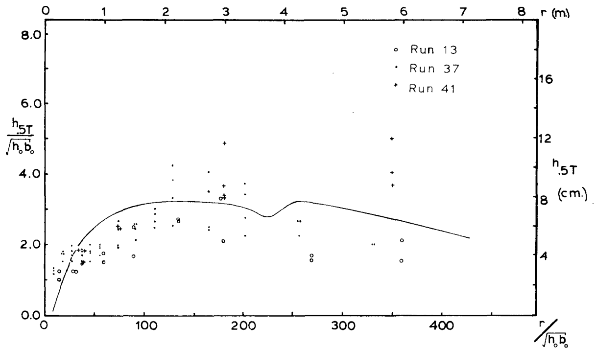
Figure 8.12b Half Temperature Depth vs. Distance, Experimental Comparison to Model
