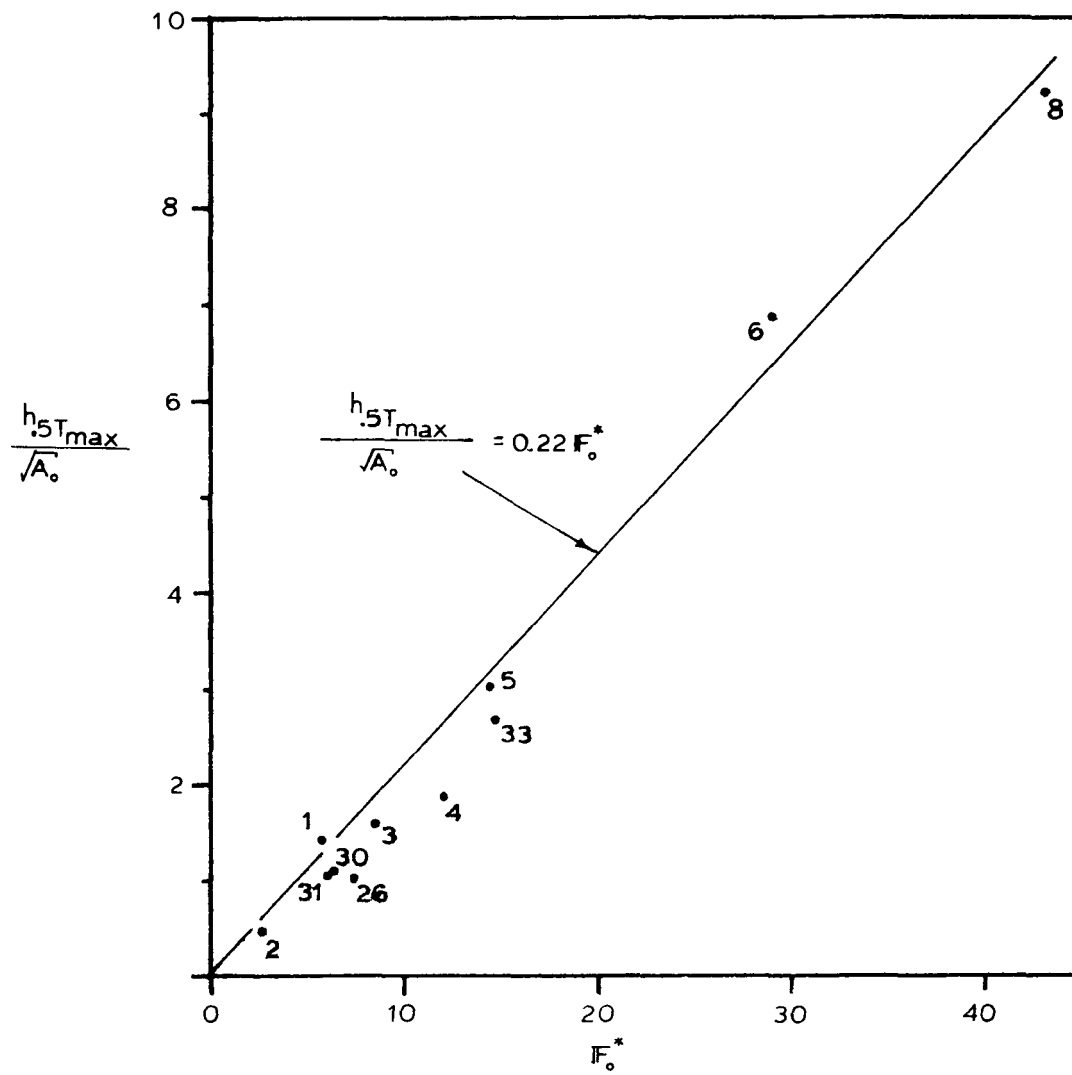
Figure 4.8 Normalized Maximum Half-Temperature Depth vs. Quarter Module "Port" Discharge Froude Number, Stagnant Experiments
