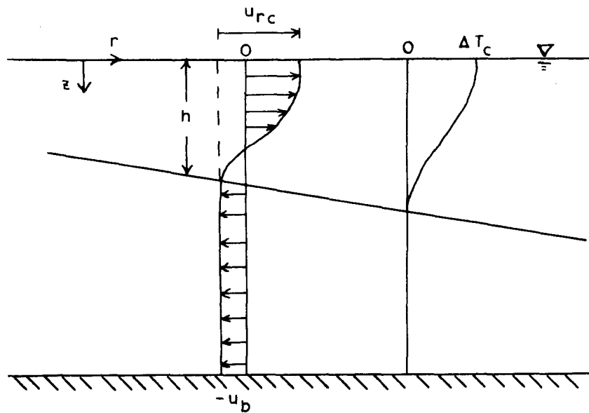
Figure D.1 Schematic Diagram of Surface Jet Vertical Velocity and Temperature Profiles.
