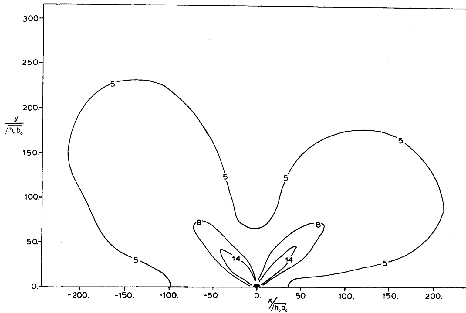
Figure A.2.16 Plan View. Run #15.
