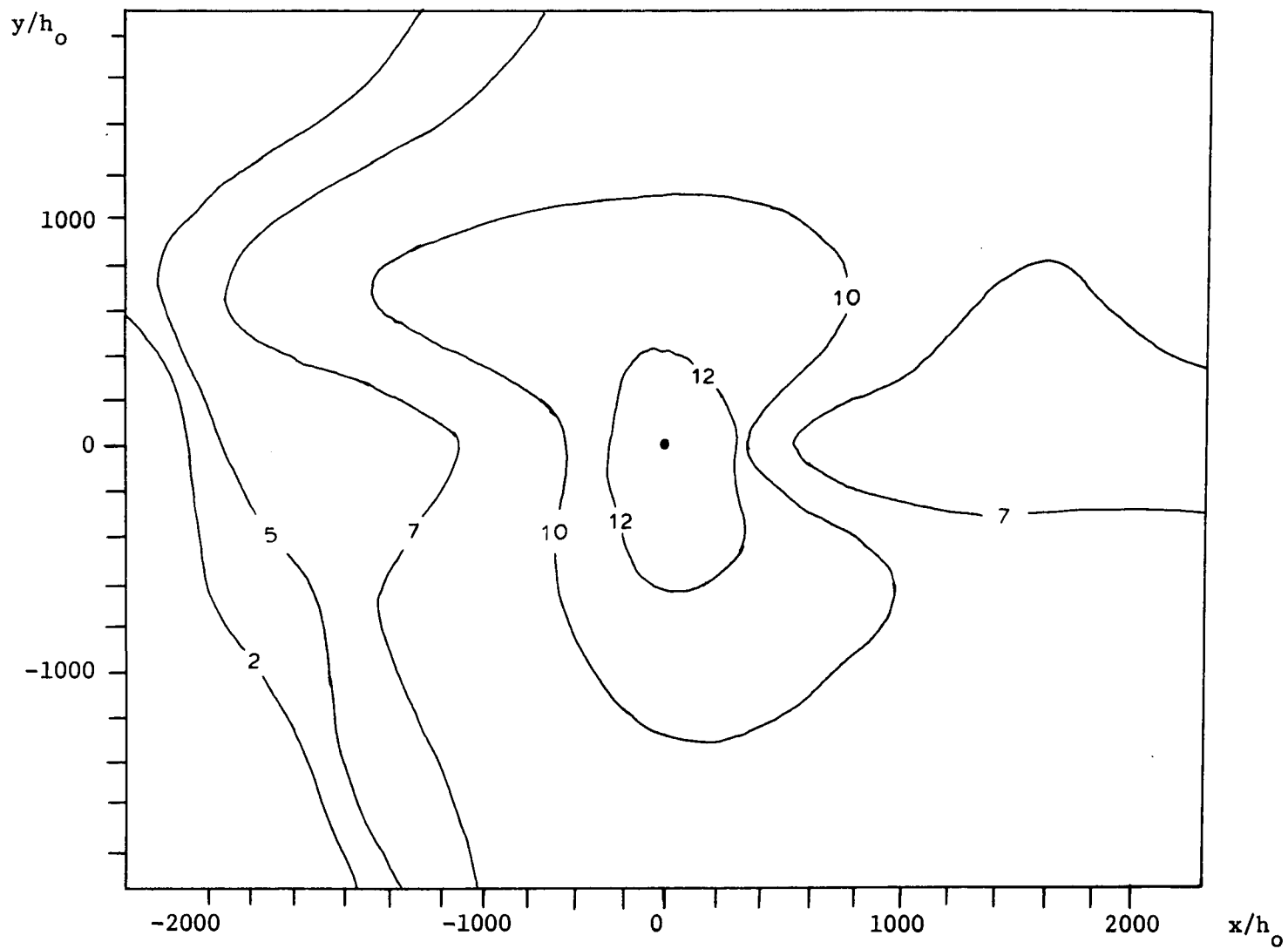
Figure A.3.28 Surface Plan, Run #34, Radial Jet Discharge.
