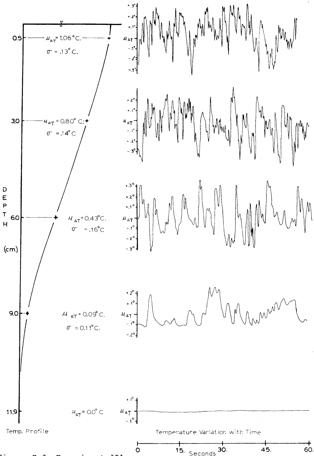
Figure C.3 Experiment #51 @ r = 0.91m
