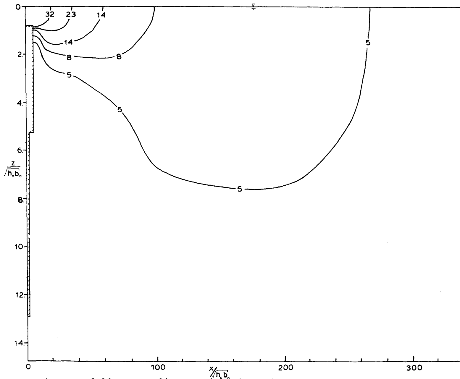
Figure A.2.18 Centerline Section of Jet #2. Run #15.
