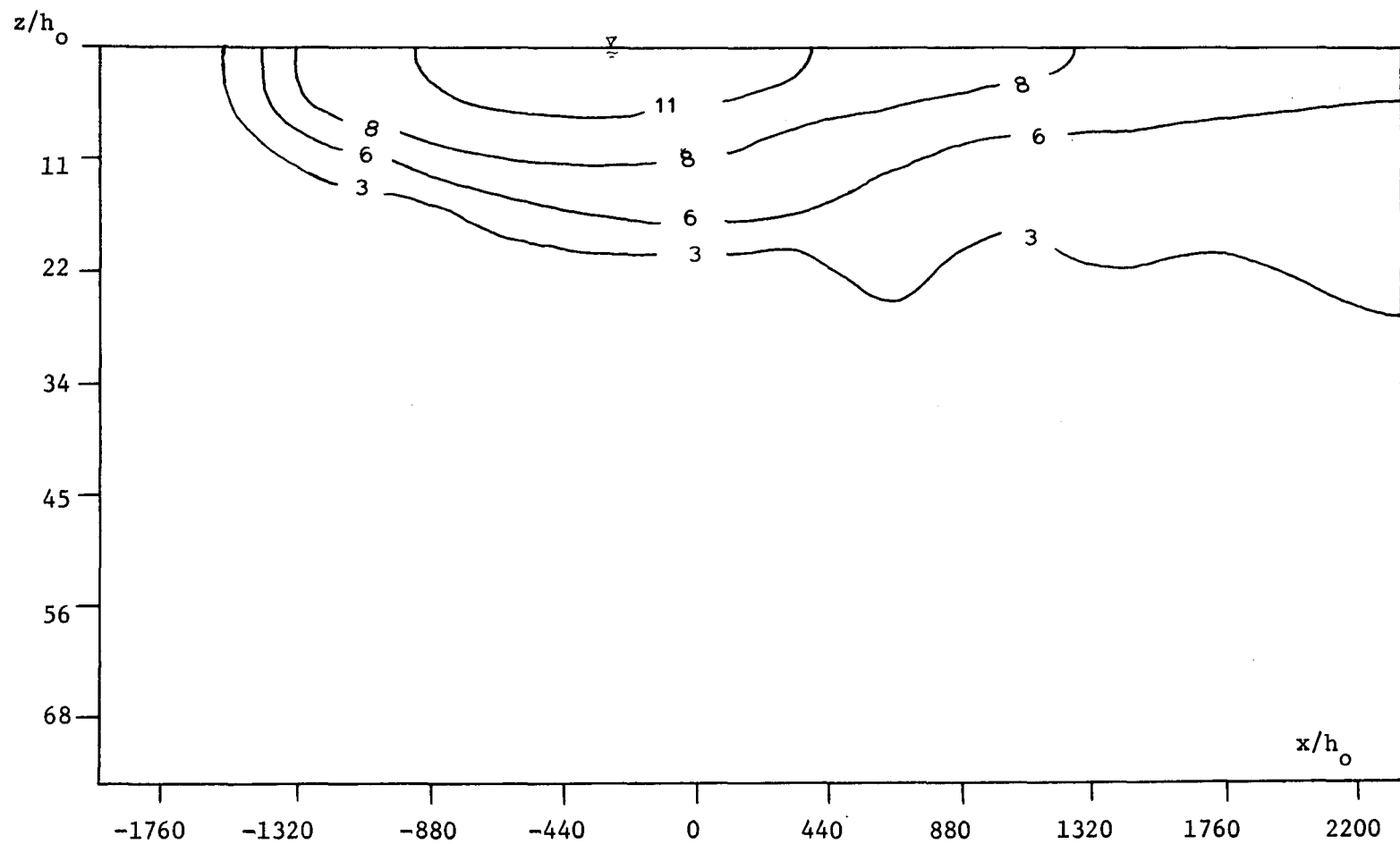
Figure A.3.20 Longitudinal Transect B-B at y = 2.25\text{m} , Run #23.
