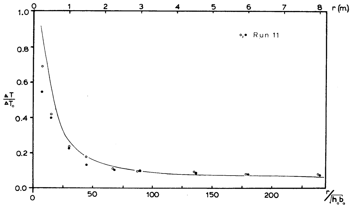
Figure 8.10a Temperature vs. Distance, Experimental Comparison to Model
