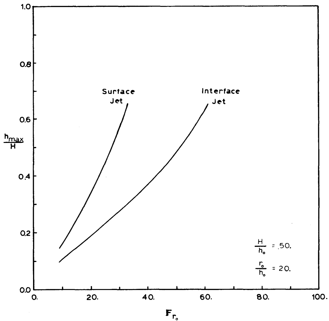
Figure 7.9 Normalized Maximum Jet Thickness vs. Discharge Densimetric Froude Number for Surface Jet and Interface Jet
