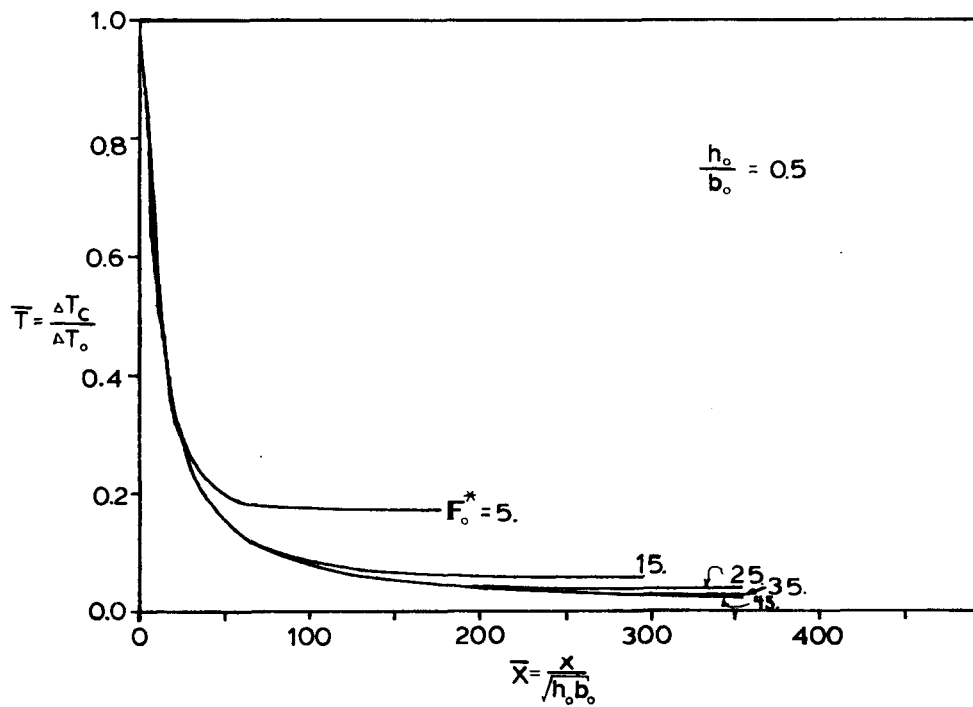
Figure 8.4a Centerline Temperature vs. Distance, Varying F_o^*
