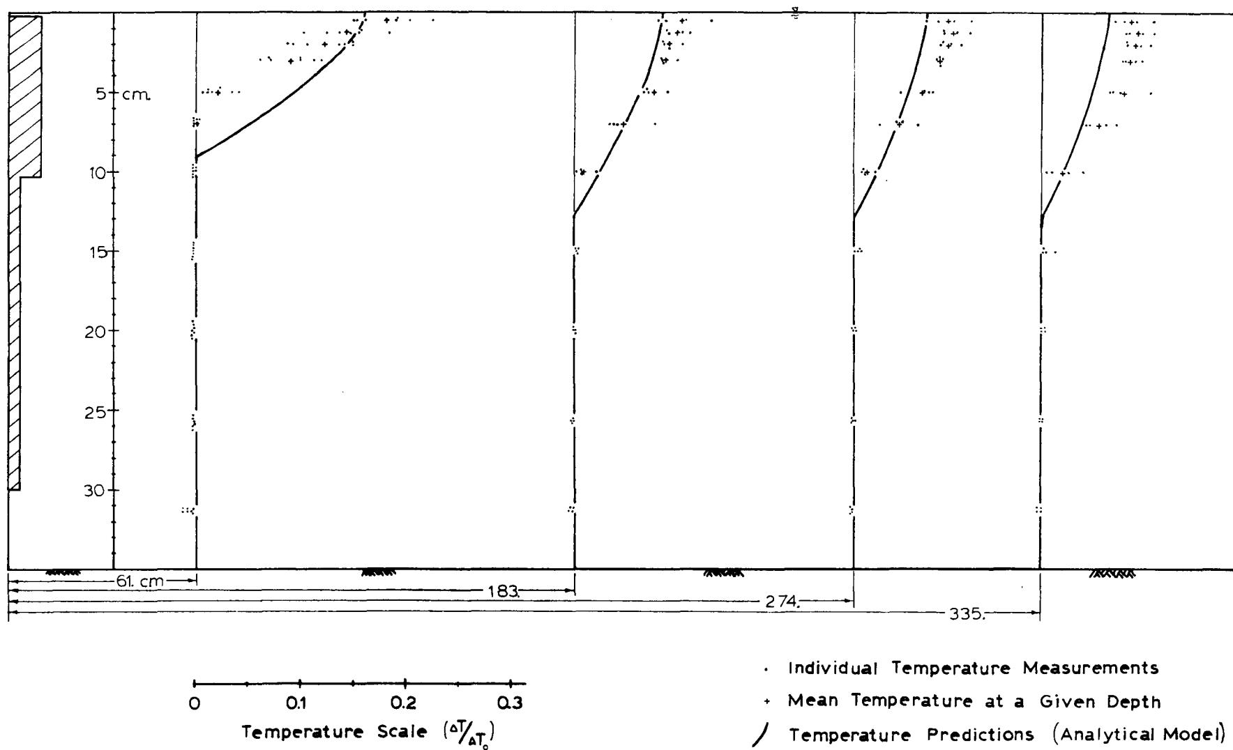
Figure 7.15 Temperature Profile Comparison Between Analytical Model and Data (Experiment #33; Stagnant, Radial Jet Discharge).
