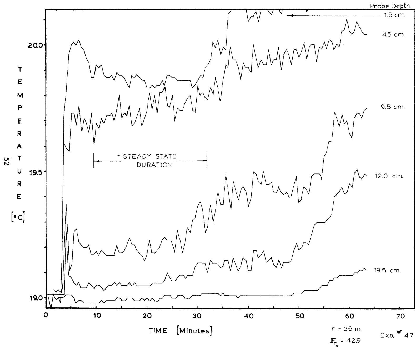
Figure 4.4 Temperature vs. Time at Various Depths
