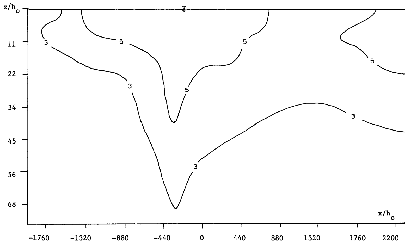
Figure A.3.14 Longitudinal Transect A-A at y = 2.25\text{m} , Run #21.
