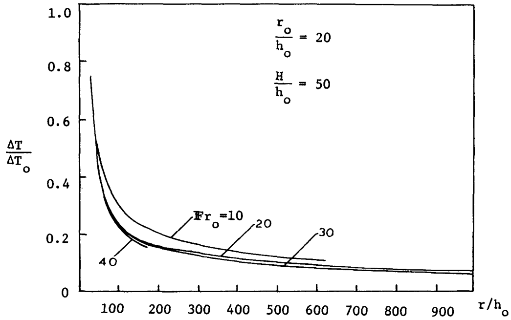
Figure 7.2a Temperature vs. Distance, Varying Fr_o
