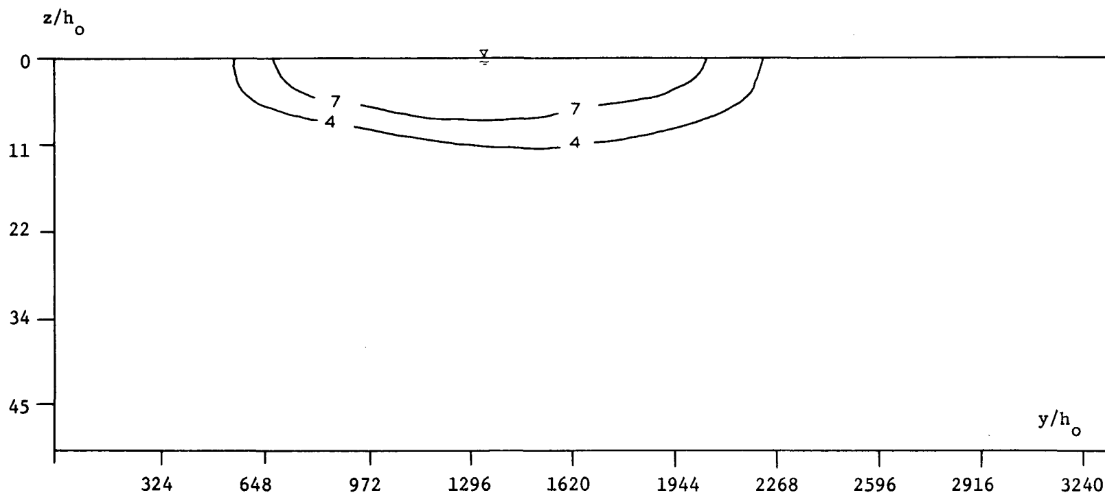
Figure A.3.18 Lateral Transect B-B at x = -4\text{m} , Run #22.
