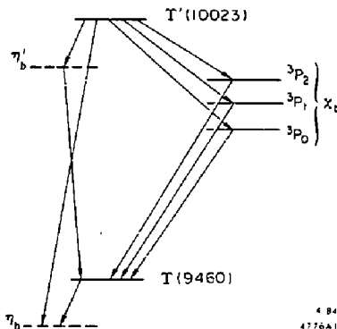
Fig. 1. The level scheme for b\bar{b} bound states below the T(2S) . The transitions to the \chi_b states are electric multipole. Transitions to the \eta_b states are magnetic multipole and hence suppressed in comparison to the electric transitions.
