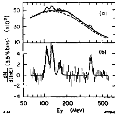
Fig. 7. (a) A fit to the photon spectrum of Fig. 6(b) with a model for cascade transitions from the T(2S) . Details of the model are explained in the text, and (b) The fit of Fig. 7(a) after subtracting the polynomial background and the background due to charged particles.
