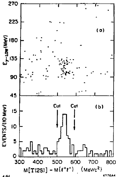
Fig. 4. (a) Scatter plot of the energy of the low energy photon in the reaction T(2S) \rightarrow \gamma\gamma\ell^+\ell^- vs. the mass difference M(T(2S)) - M(\ell^+\ell^-) . M(\ell^+\ell^-) is calculated as the mass recoiling against the \gamma\gamma system, and (b) Projection of Fig. 4(a) on the mass difference axis. A cut was made at 545 \pm 45 MeV to select cascade events.
