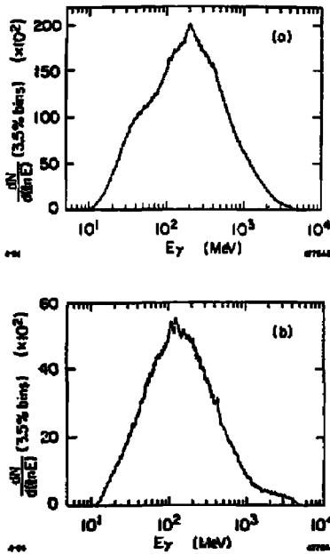
Fig. 6. Inclusive photon spectra from hadronic decays of the T(2S) : (a) All neutral tracks in the solid angle covered by the chambers, and (b) After applying all the photon selection criteria described in the text.
