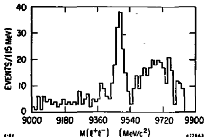
Fig. 3. A plot of the recoil mass ( M_{l^+l^-} ) in the exclusive channel T(2S) \rightarrow \gamma\gamma l^+l^- after selecting events of this topology.
