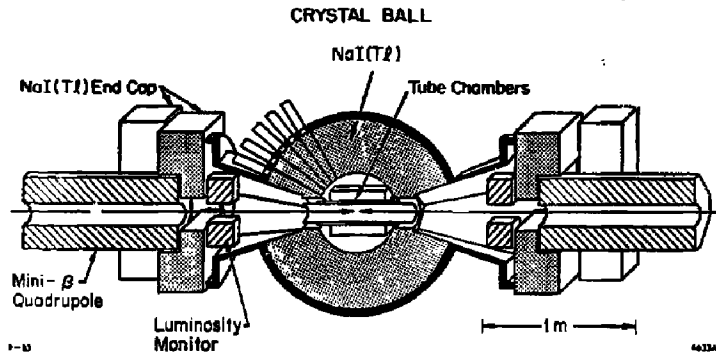
Fig. 2. The Crystal Ball Detector at DORIS II.
