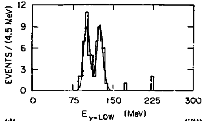
Fig. 5. Energy distribution of the low energy photon from the final cascade sample [T(2S) \rightarrow \gamma\gamma\ell^+\ell^-] . The curve is a fit to the data as described in the text.
