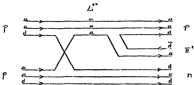
Fig. 1. Quark diagram for the reaction p + p \rightarrow \Delta^{++} + n
