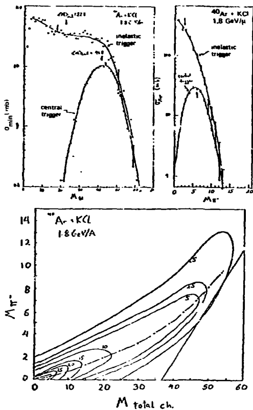
Fig. 3. Top: total multiplicity and \pi^- multiplicity distributions for the inelastic and central trigger in the interaction of Ar on KCl at 1.8 GeV/A. Bottom: correlation between total multiplicity and \pi^- multiplicity for the inelastic trigger as contours of constant cross section (mbarns).
