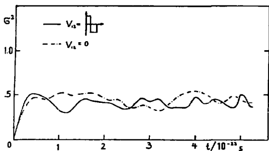
Fig.2: Same as fig. 1 but a different two-body interaction V_1=45 MeV, V_2=-30 MeV, R_1=2 fm, R_2=5 fm.
