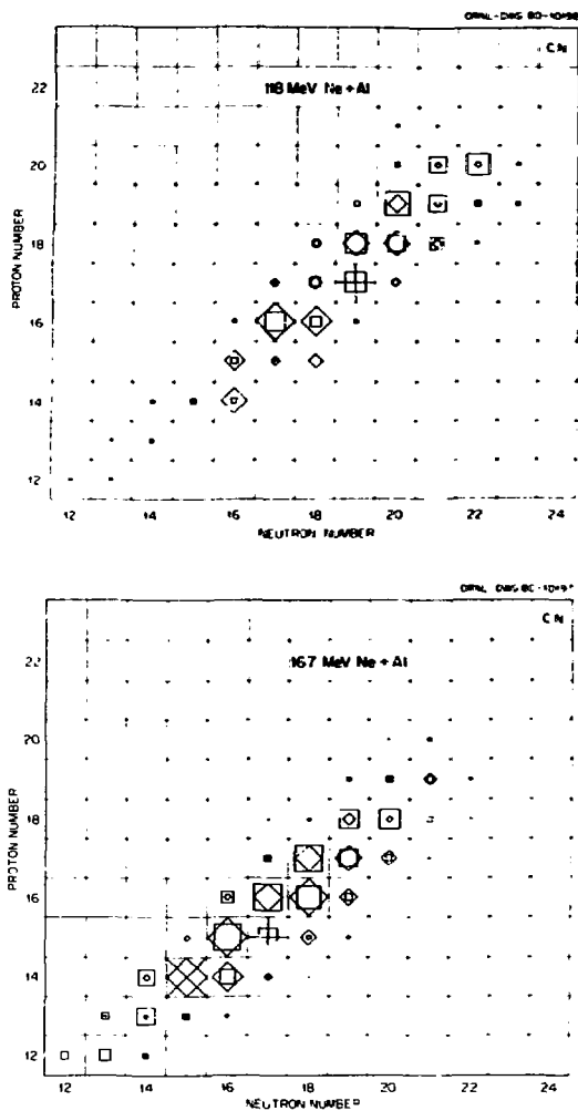
Fig. 2. Comparisons between measured yields ( \square, X ) and Monte Carlo evaporation calculations ( \diamond, + ). Cf. Fig. 1.
