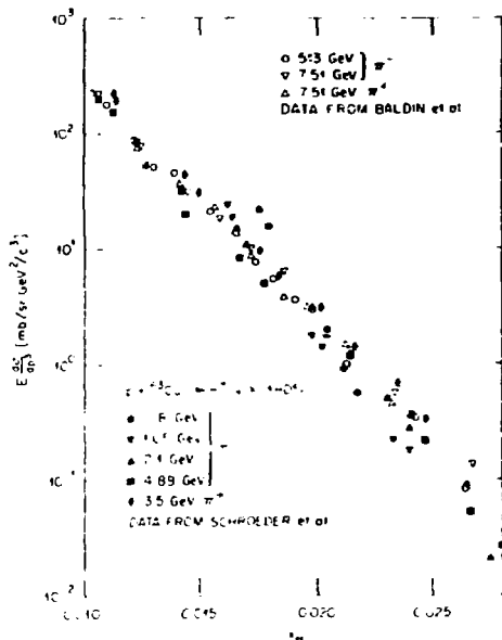
Fig. 2. Experimental invariant cross section for p + Cu \rightarrow \pi^{\pm} + X ( 180^{\circ} ). Data are from Refs. 5 and 7.
