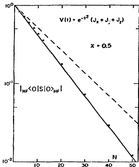
Fig. 2. The modulus of elastic amplitude |_{\text{HF}}\langle 0|S|0\rangle_{\text{HF}}| vs. the number of fermions ( N ) in the forced Lipkin model: exact ( x ), ordinary TDHF along the loop (dashed line) and zero'th order mean field approximation (continuous line).
