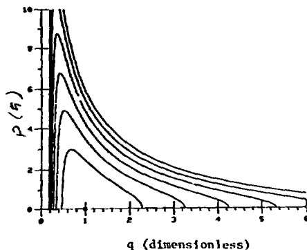
^{16}\text{O} , quadrupole
