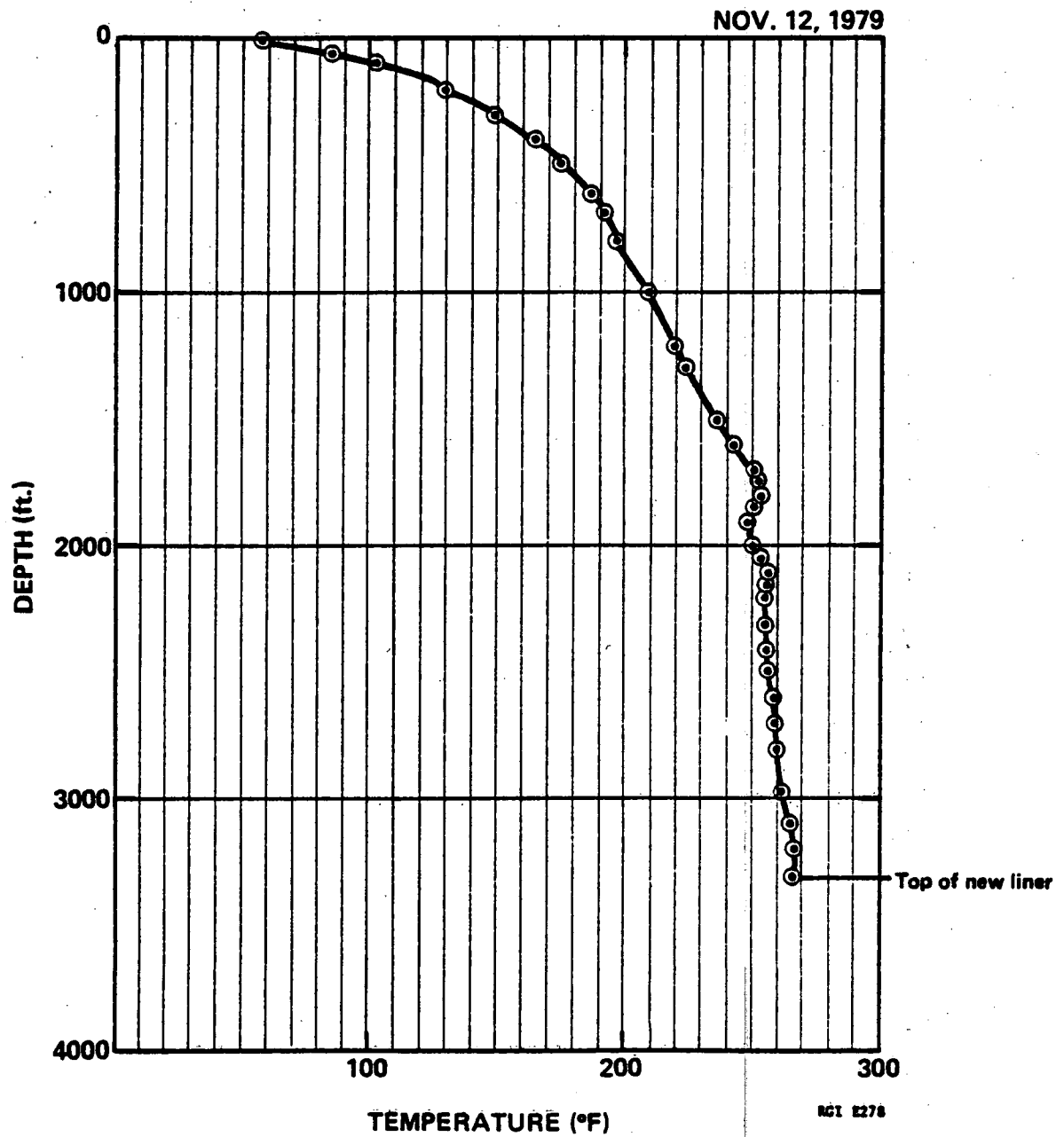
FIGURE 15 STATIC TEMPERATURE SURVEY RRGP-4 RAFT RIVER, IDAHO
