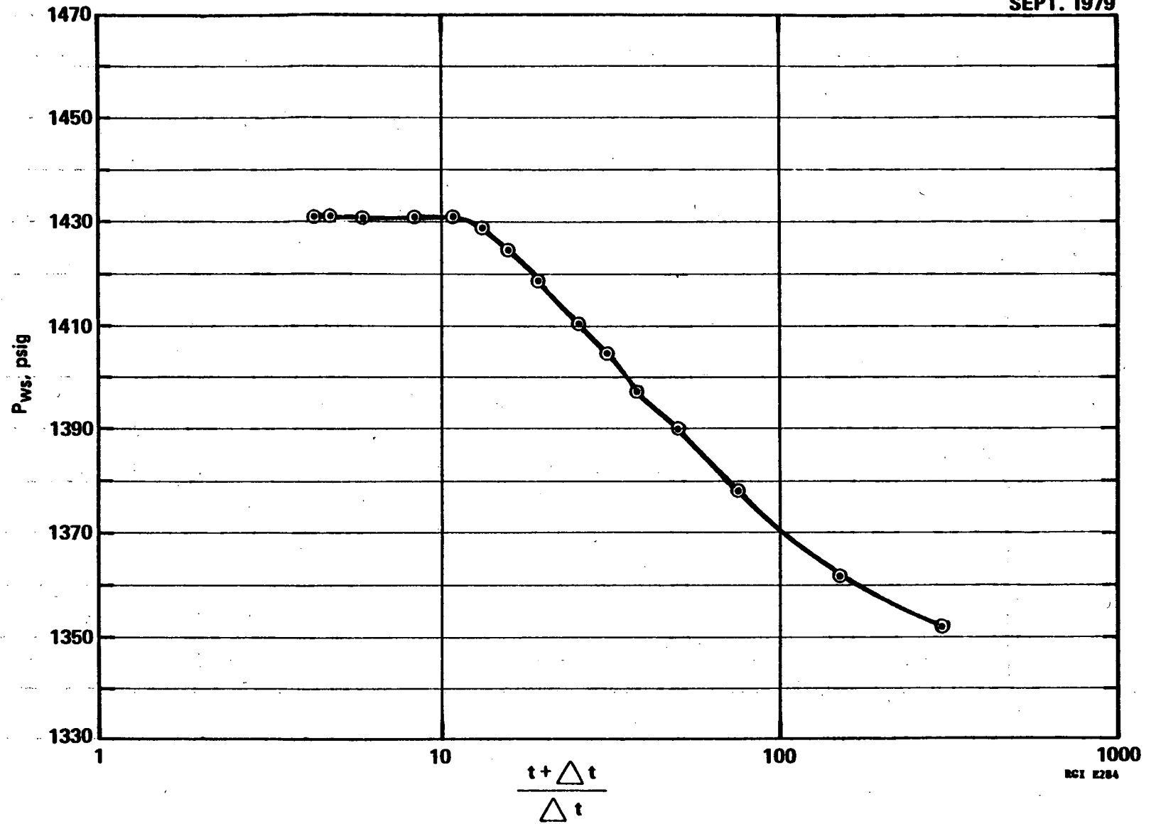
FIGURE 20 RRGP-4 BUILDUP DATA
