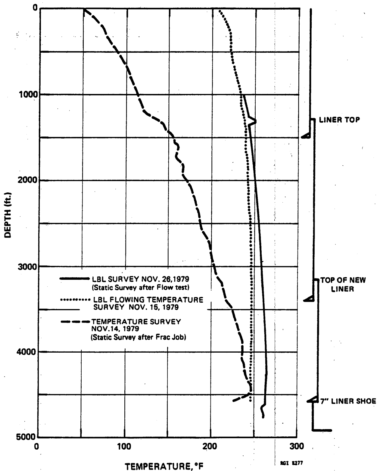
FIGURE 25 TEMPERATURE SURVEYS RAFT RIVER, IDAHO RRGP-5
