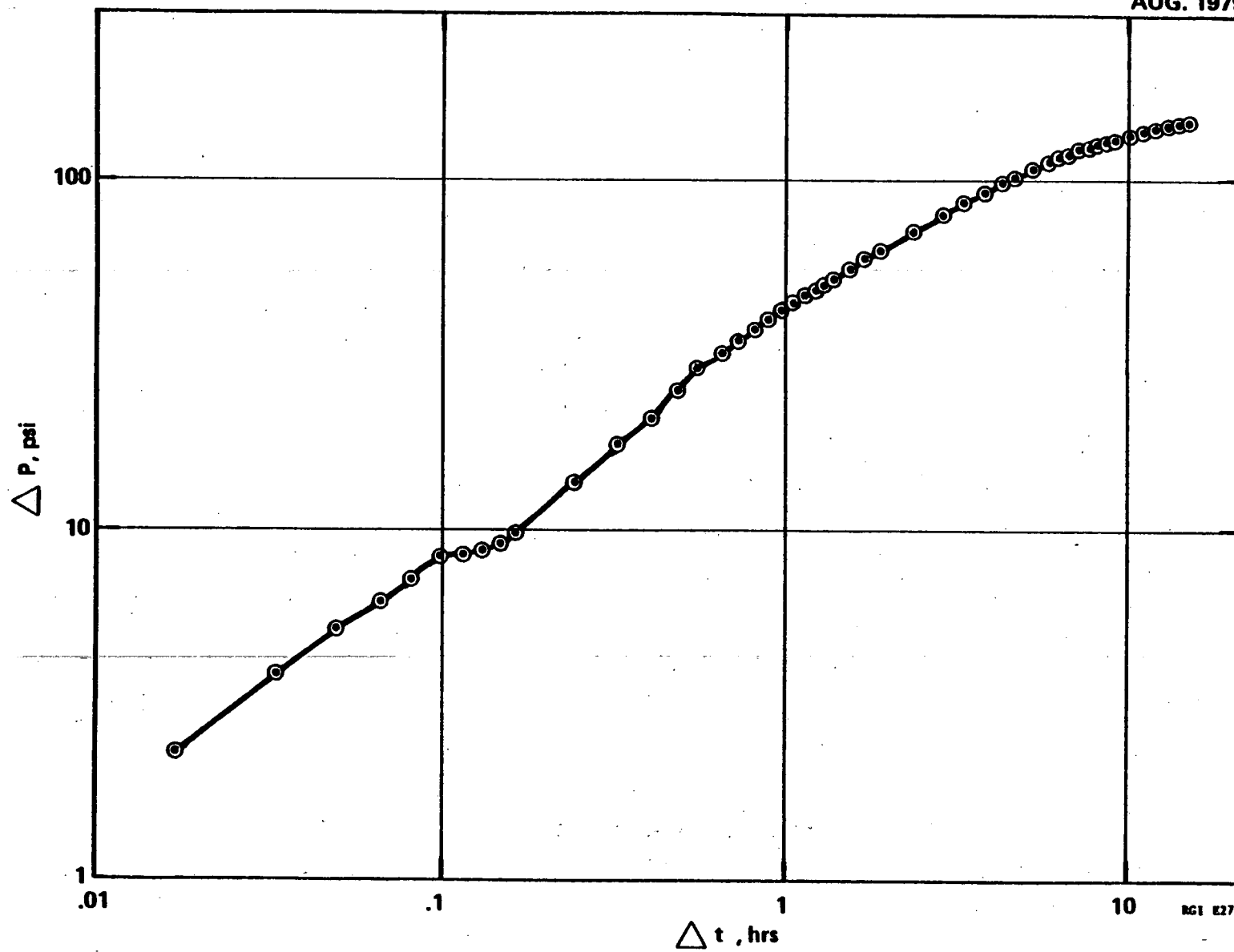
FIGURE 13 RRGP -4 BUILDUP DATA
