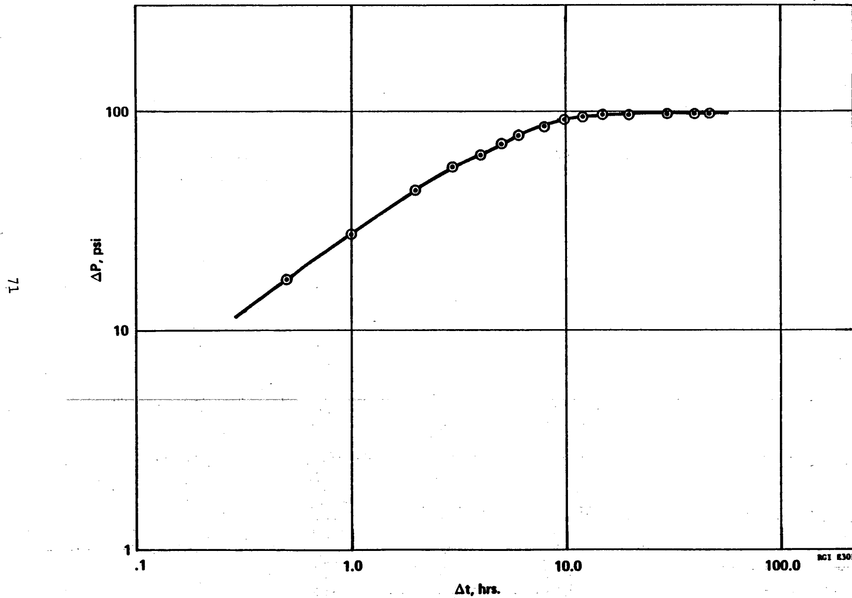
FIGURE 19 RRGP-4 BUILDUP DATA
