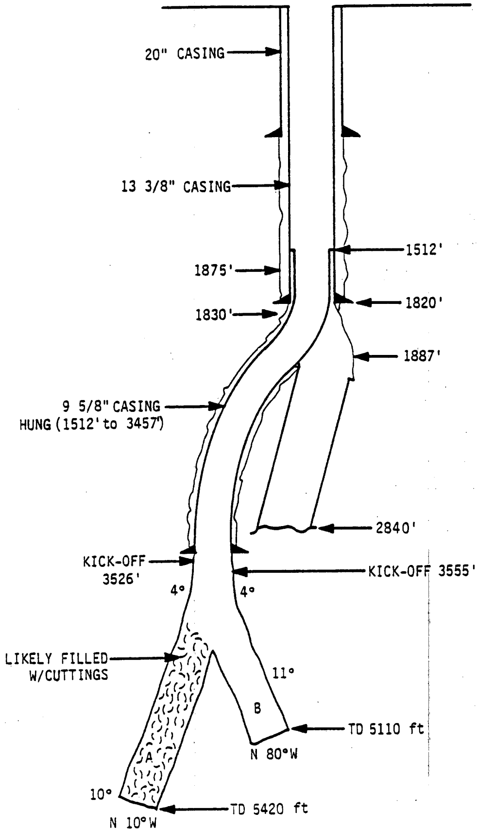
FIGURE 3 SCHEMATIC OF RAFT RIVER RRG-4
