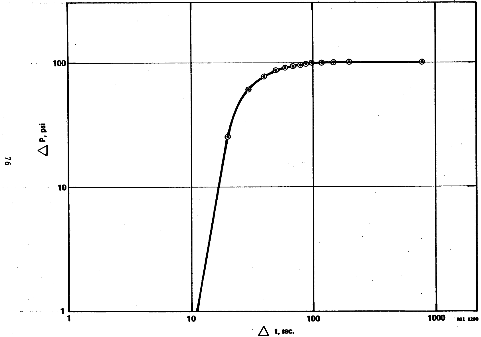
FIGURE 24 RRGP-5 BUILDUP DATA
