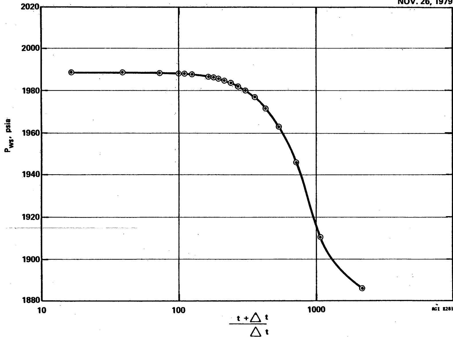
FIGURE 23 RRGP-5 BUILDUP DATA
