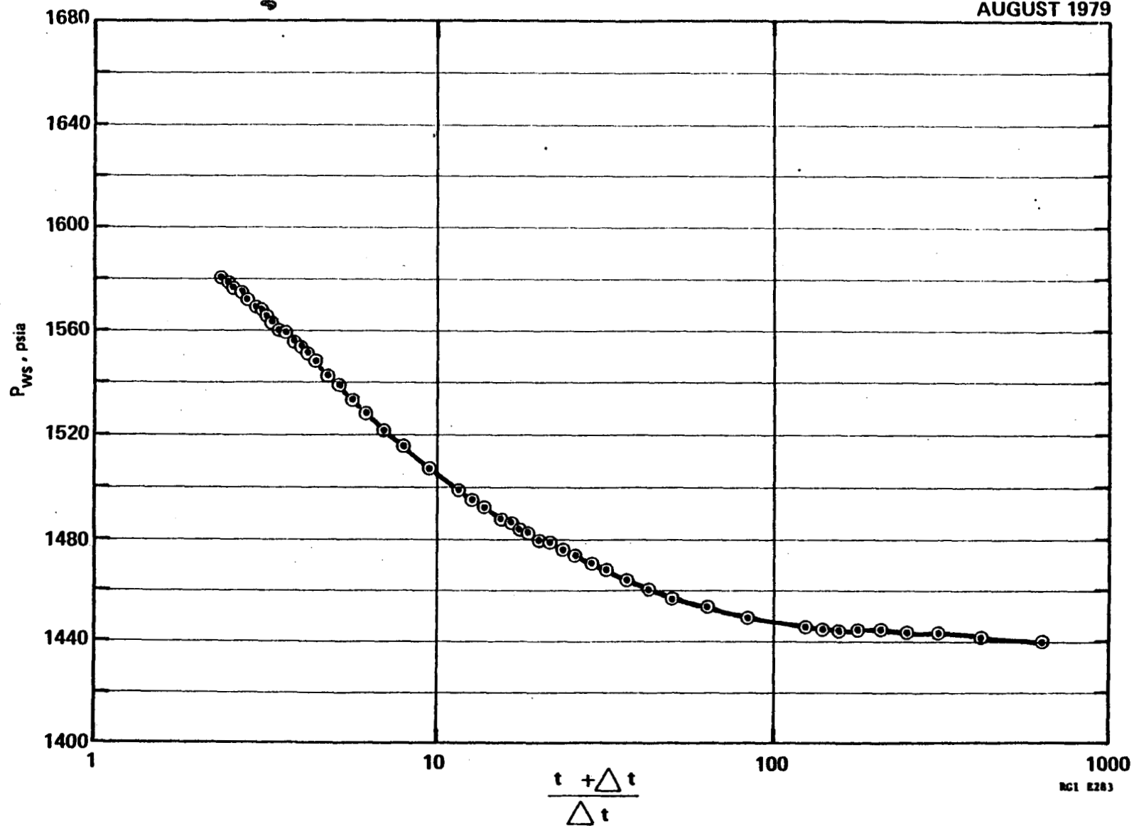
FIGURE 14 RRGP-4 BUILDUP DATA
