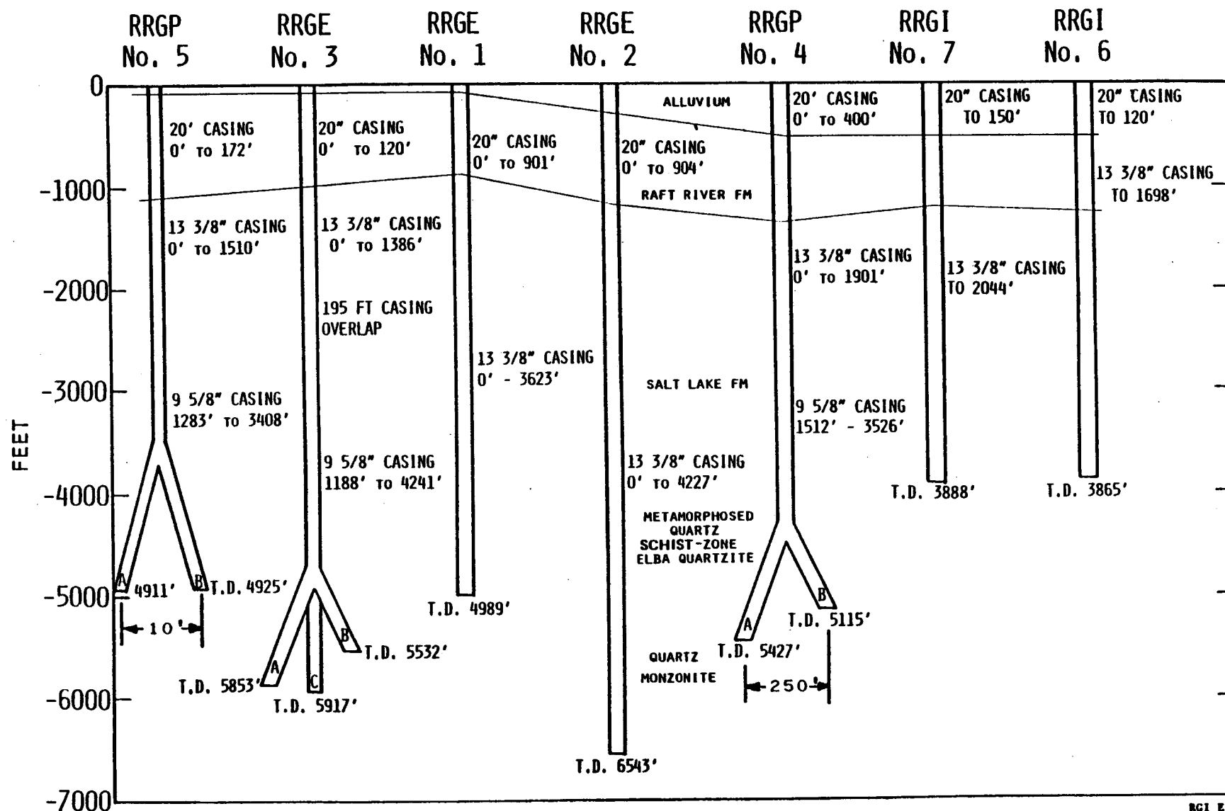
FIGURE 2 RAFT RIVER WELL SYSTEM JANUARY 1979
