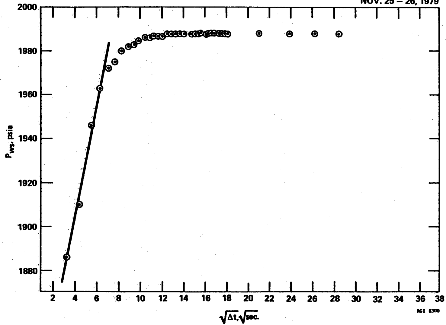
FIGURE 22 RRGP-5 BUILDUP DATA
