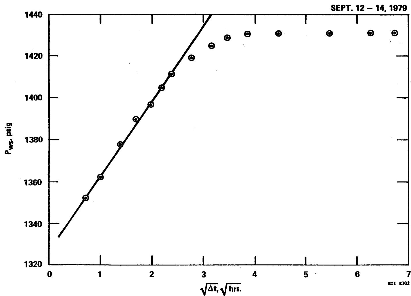
FIGURE 18 RRGP-4 BUILDUP DATA
