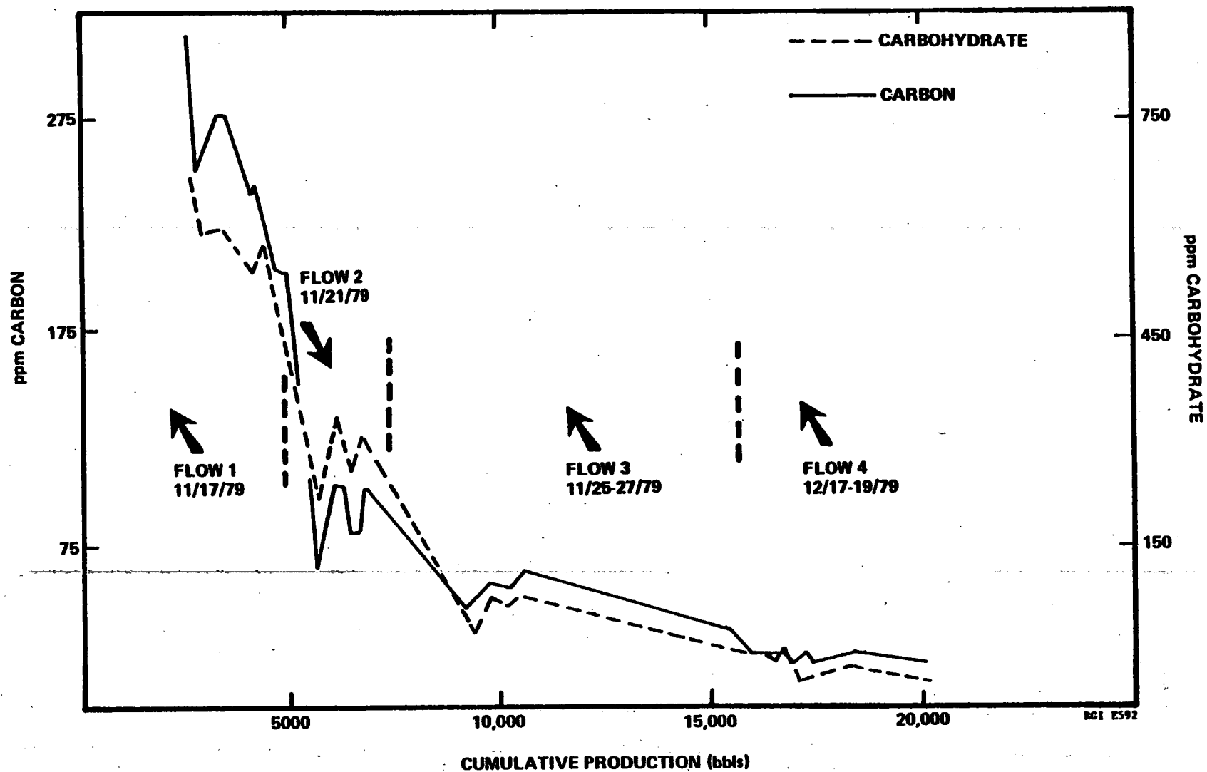
FIGURE 29 TOTAL ORGANIC CARBON AND CARBOHYDRATE CONCENTRATION OF RRGP-5 PRODUCED FLUID
