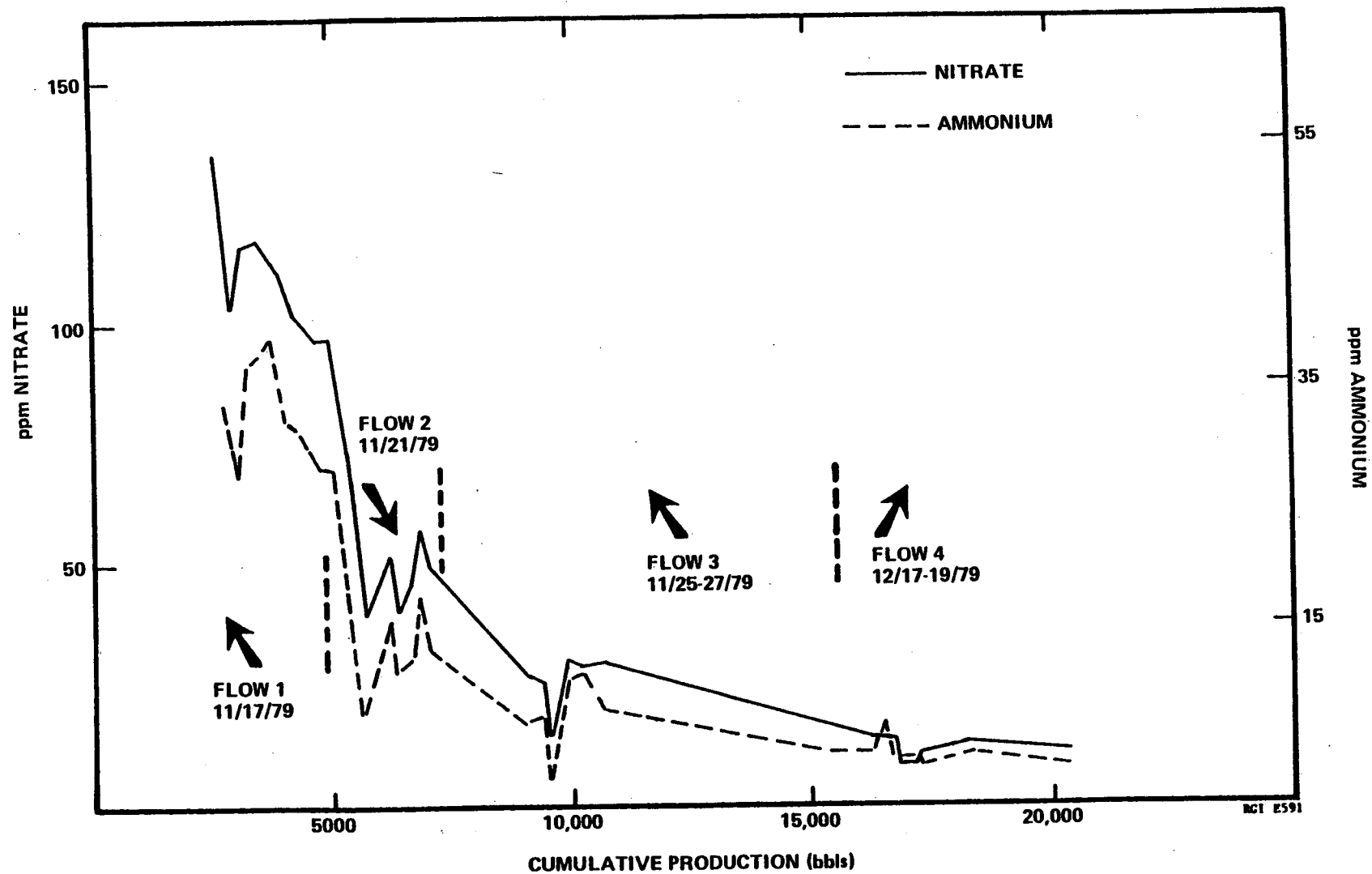
FIGURE 30 AMMONIUM AND NITRATE TRACER CONCENTRATION IN RRGP-5 PRODUCED FLUID
