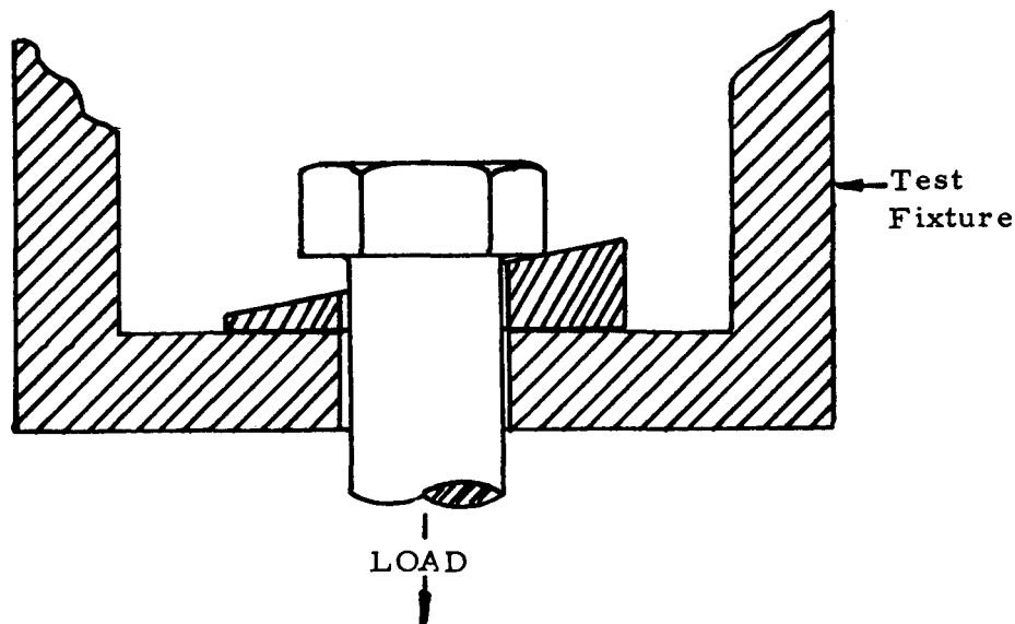
Figure 53. Wedge test.
