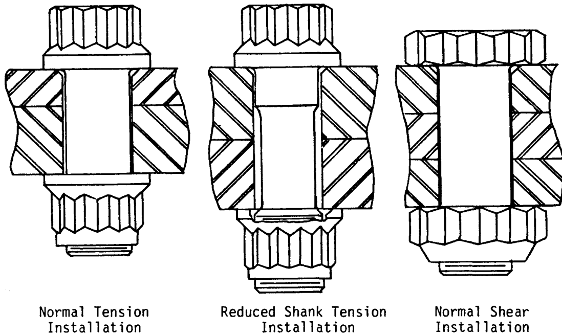
Figure 8. Shank clearances.
