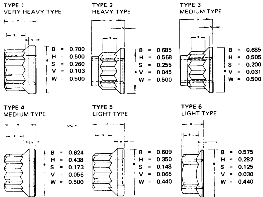
Figure 37. For the purpose of calculating preload loss due to permanent set, aircraft nuts are classified into six types. (Measurements refer to 3/8" nut.)
