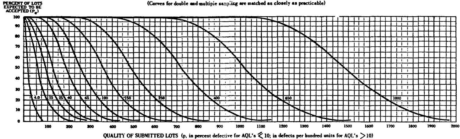
CHART B - OPERATING CHARACTERISTIC CURVES FOR SINGLE SAMPLING PLANS
