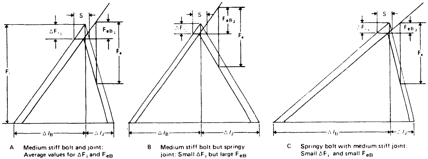
Figure 35. The effect of bolt and joint stiffness on preload loss and external load absorbed by the bolt.
