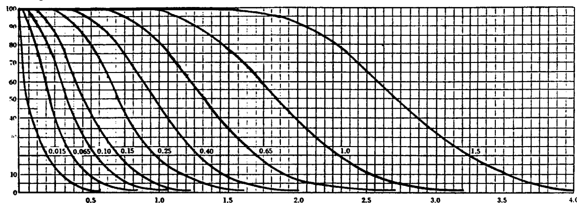
CHART P - OPERATING CHARACTERISTIC CURVES FOR SINGLE SAMPLING PLANS
