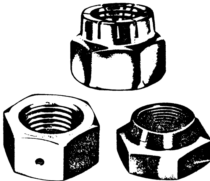
Figure 1. Three types of one-piece, all-metal, prevailing-torque locknuts -- deflected beam (top), deflected thread (left) and out-of-round threaded collar (right).
