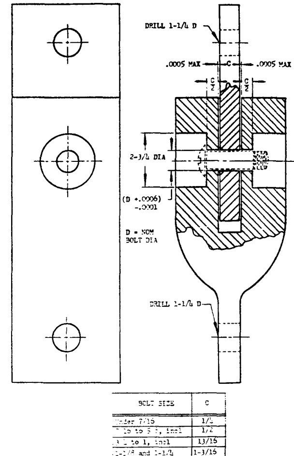
FIGURE 2. Double shear jig for clevis bolts
