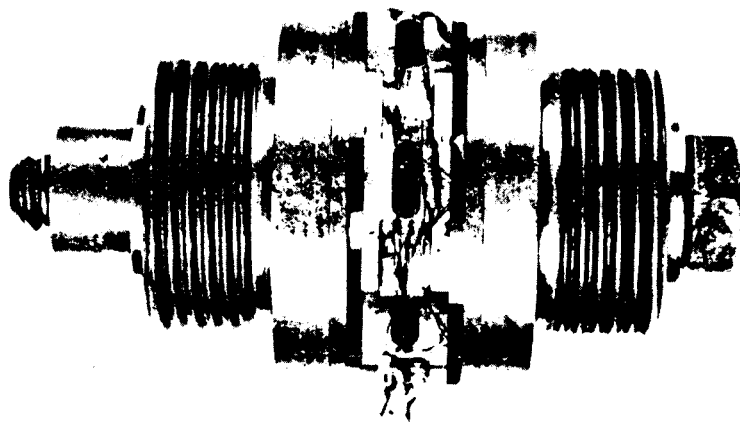
Figure 39. Strain-gaged test joint used in deriving preload and preload-loss formulae.
