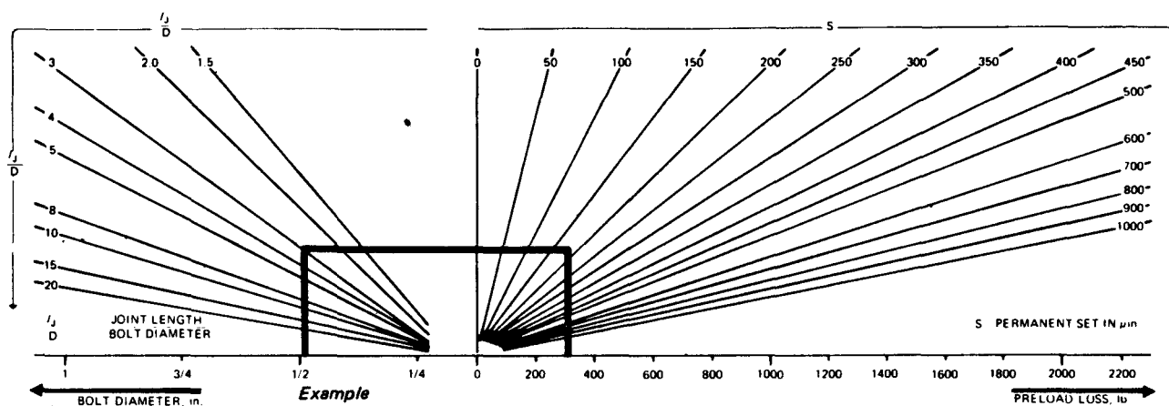
Figure 43. Nomograph converts permanent set into preload loss as a function of joint stiffness ( I_j/D ) for socket head cap screws and hex-head screws installed in steel plates.
