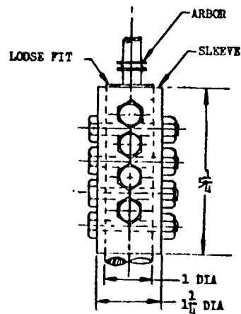
FIGURE 1. Test arbor
