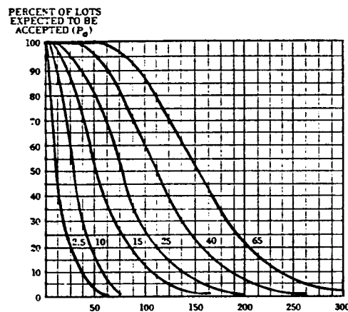
CHART C - OPERATING CHARACTERISTIC CURVES FOR SINGLE SAMPLING PLANS
