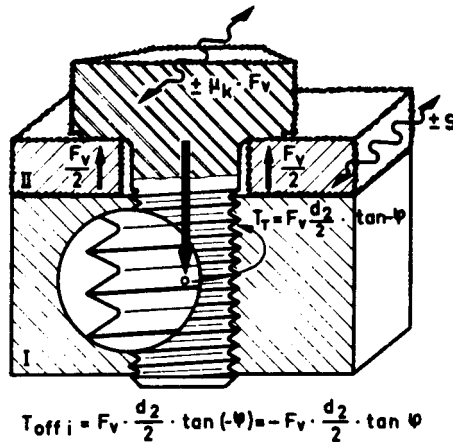
Figure 48. Transverse force relative motion diagram.
