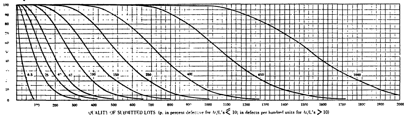
CHART A - OPERATING CHARACTERISTIC CURVES FOR SINGLE SAMPLING PLANS
