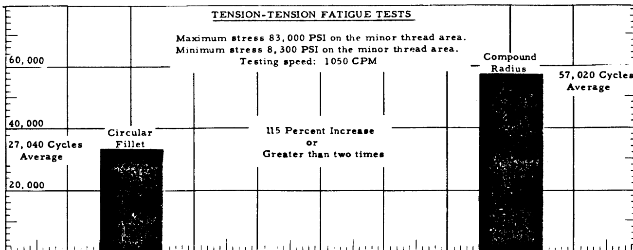
Figure 6. Effect of fillet radii configuration on fatigue life of socket head cap screws.
