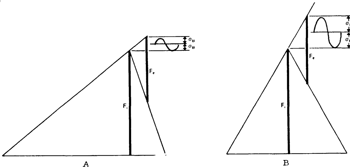
Figure 28. Joint diagram of a springy bolt in a stiff joint (A) is compared to a diagram of a stiff bolt in a springy joint (B). Preload F_i and external load F_e are the same, but diagrams show that alternating bolt stresses are significantly lower with a spring bolt in a stiff joint.
