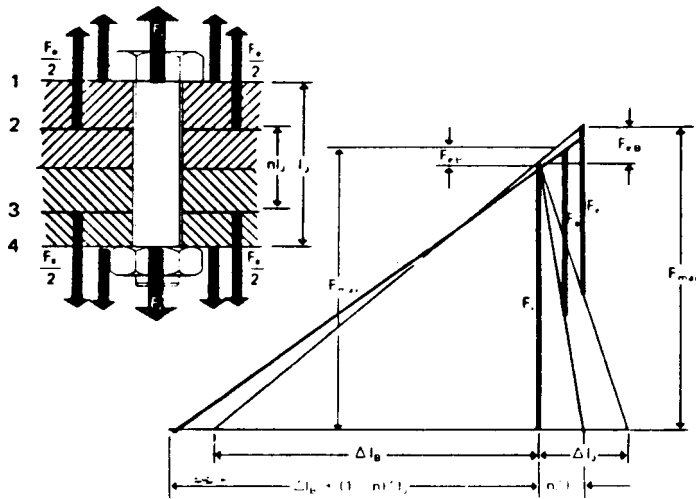
Figure 30. Joint diagram shows effect of loading planes of F_e on bolt loads F_{eB} and F_b max resulting from F_e applied in planes 1 and 4. The diagram shows reduced bolt loads when F_e is applied in planes 2 and 3.
