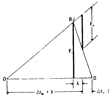
Figure 23. Simple joint diagram showing external load F_e added.
