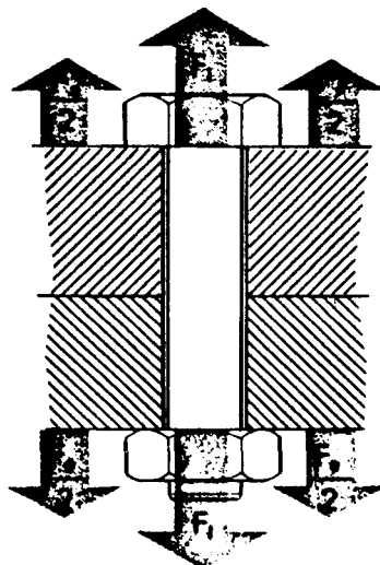
Figure 20. Simple bolted joint with axial tensile preload on bolt F_1 and axial tensile extrenal load on joint F_e .
