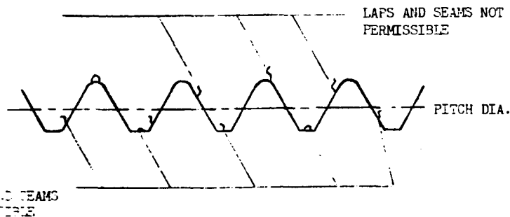
FIGURE 3. Location of permissible and nonpermissible laps, seams, and irregularities
