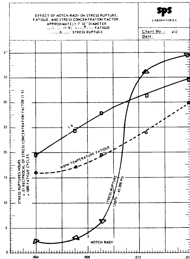
Figure 13. Effect of notch radii on stress rupture, fatigue, and stress concentration factor approximately 7/16" diameter.
