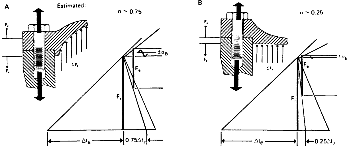
Figure 31. When external load is applied relatively near the bolt head, the joint diagram shows the resulting alternating stress \Delta\sigma_B (A). When the same value of external load is applied relatively near the joint's center, lower alternating stress results (B).
