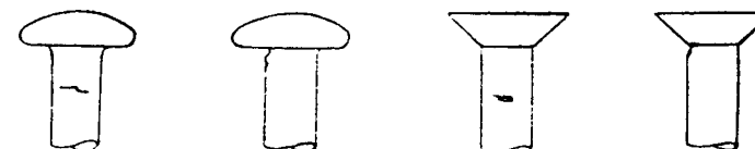
FIGURE 2. Transverse discontinuities in the head or shank.
