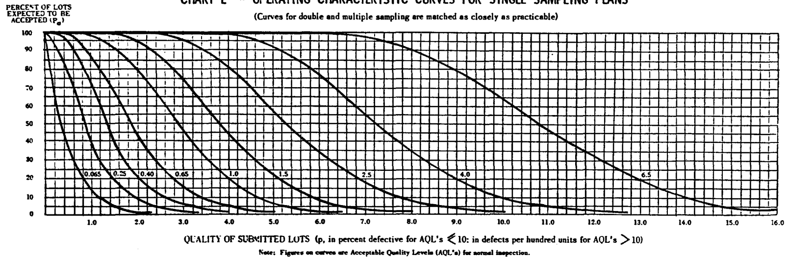
CHART L - OPERATING CHARACTERISTIC CURVES FOR SINGLE SAMPLING PLANS
