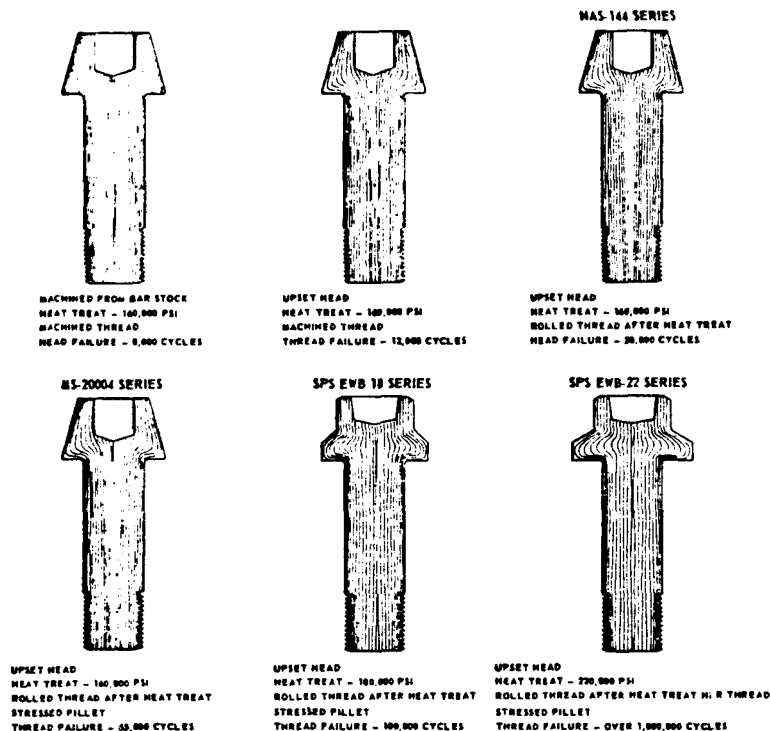
Figure 3. Bolt evolution.
