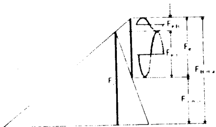
Figure 24. The external load divided into an additional bolt load, F_{eB} , and reduction in joint compression, F_{eJ} .
