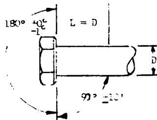
FIGURE 2. Head angularity
