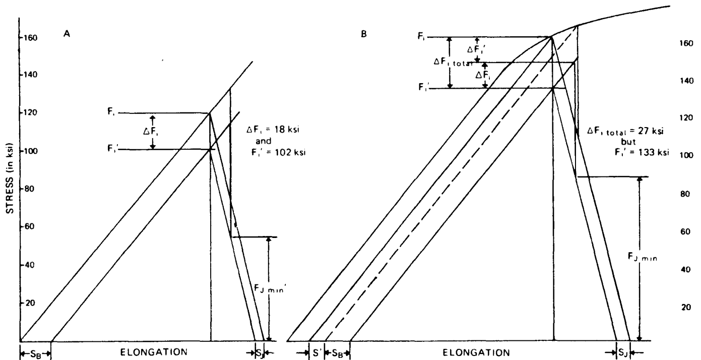
Figure 36. Comparison of preload loss and remaining load in elastic joint (left) and elastic-plastic joint (right).
