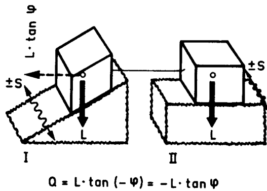
Figure 46. Transverse force dynamics.
