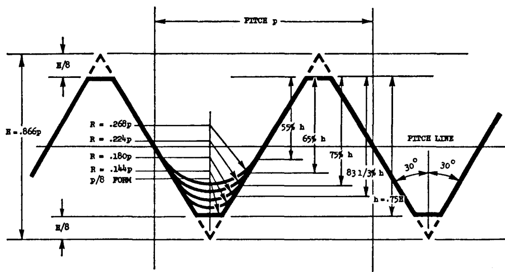
Figure 9. Radius root thread forms.
