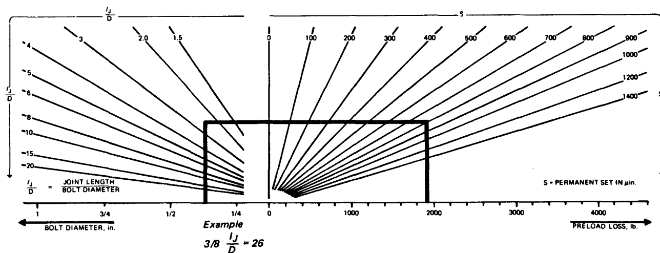
Figure 44. Nomograph converts permanent set into preload loss as a function of joint stiffness ( I_j/D ) for aircraft fasteners with bolt and nut flange diameters of 1.8 bolt diameters and holes equal to bolt diameter plus twice the fillet radius.
