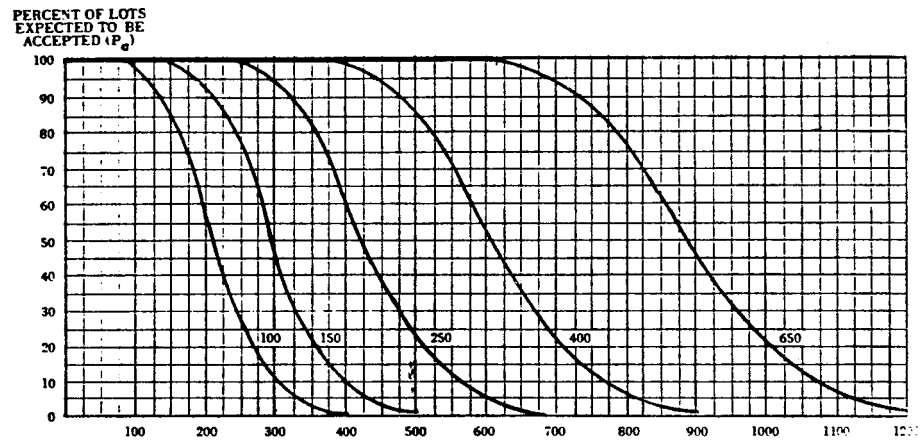
CHART C - OPERATING CHARACTERISTIC CURVES FOR SINGLE SAMPLING PLANS
