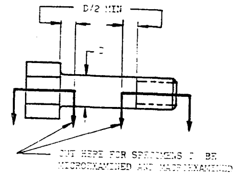
FIGURE 5. Metallurgical specimens
