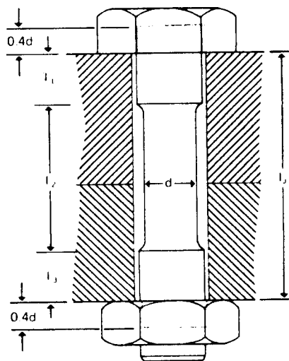
Figure 26. Analyses of bolt lengths contributing to the bolt spring rate.
