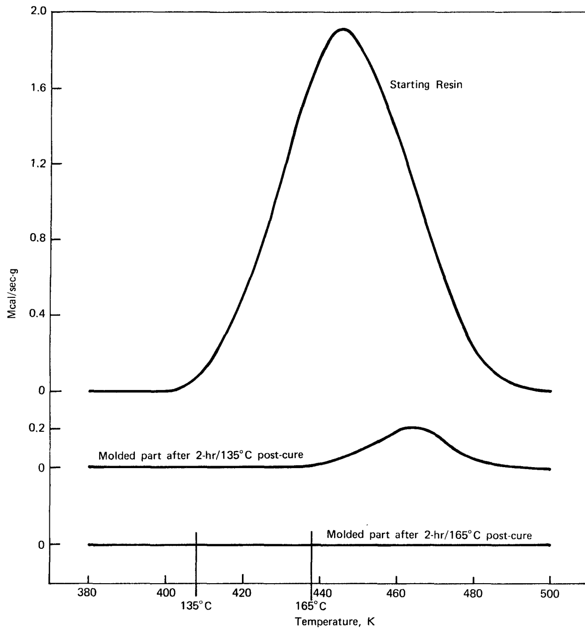
FIGURE 4 - DSC curves of DAP resin and molded Program C parts.
