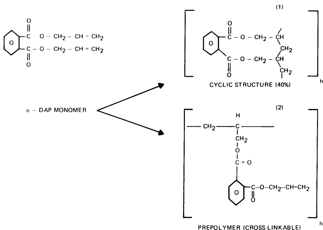
FIGURE 1 - DAP polymerization.
