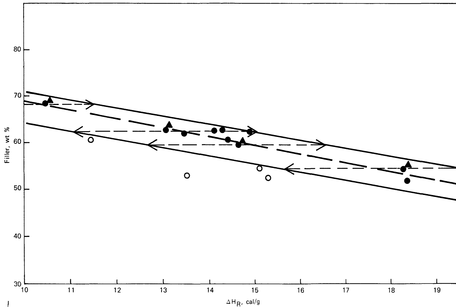
FIGURE 3 - DSC characterization of DAP molding resins. (See text on the previous page for an explanation.)
